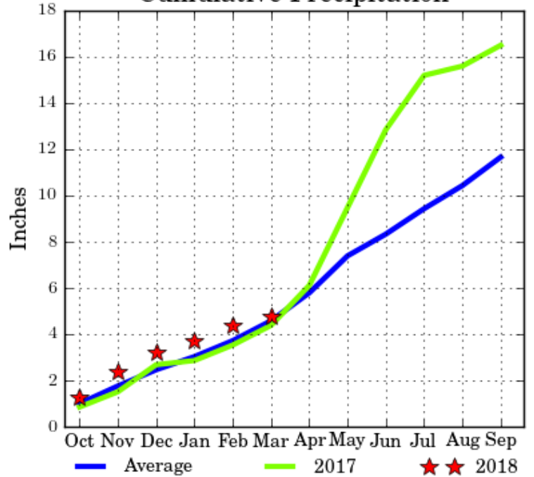
Cumulative Precipitation
