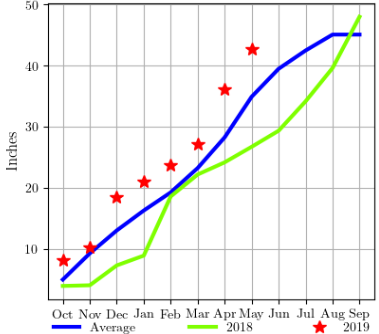
Cumulative Precipitation
