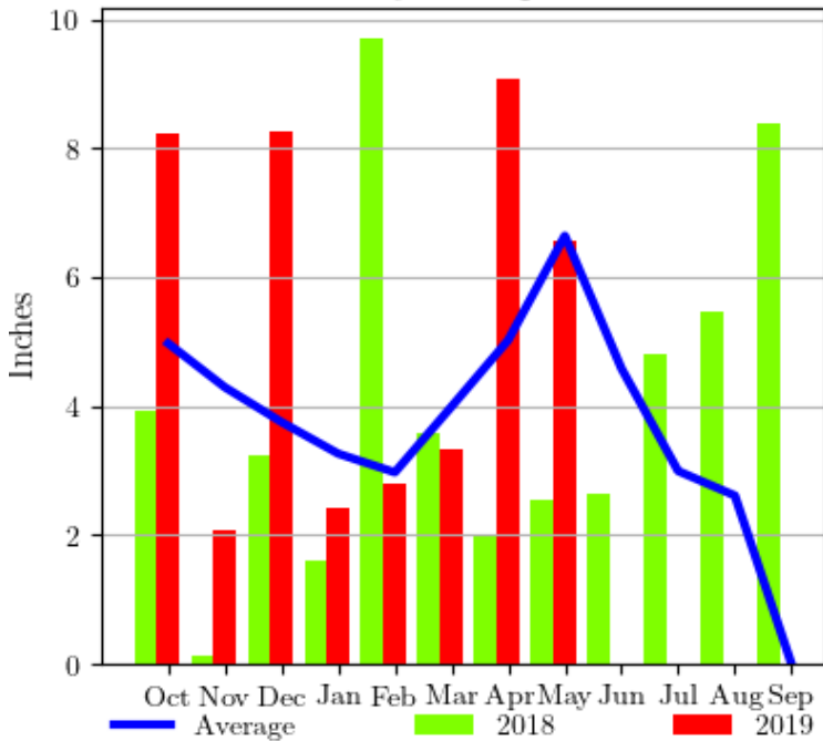
Monthly Precipitation
