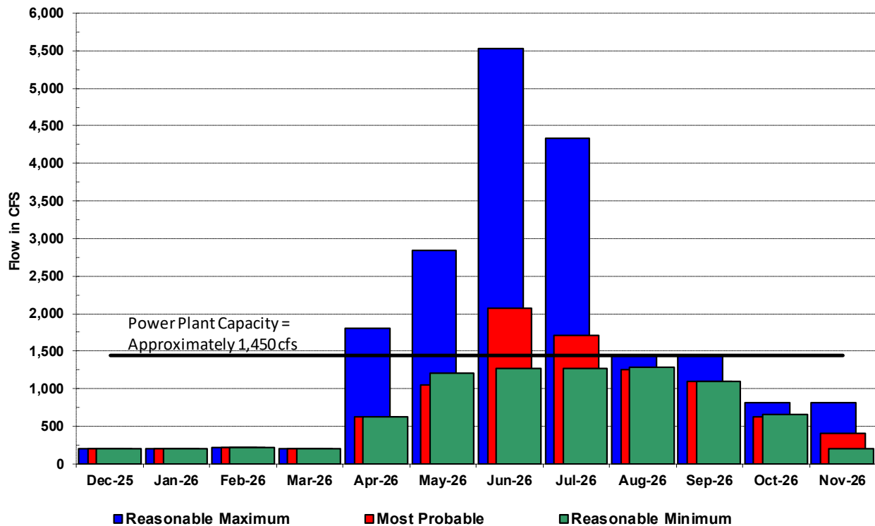
BUFFALO BILL RESERVOIR RELEASES
