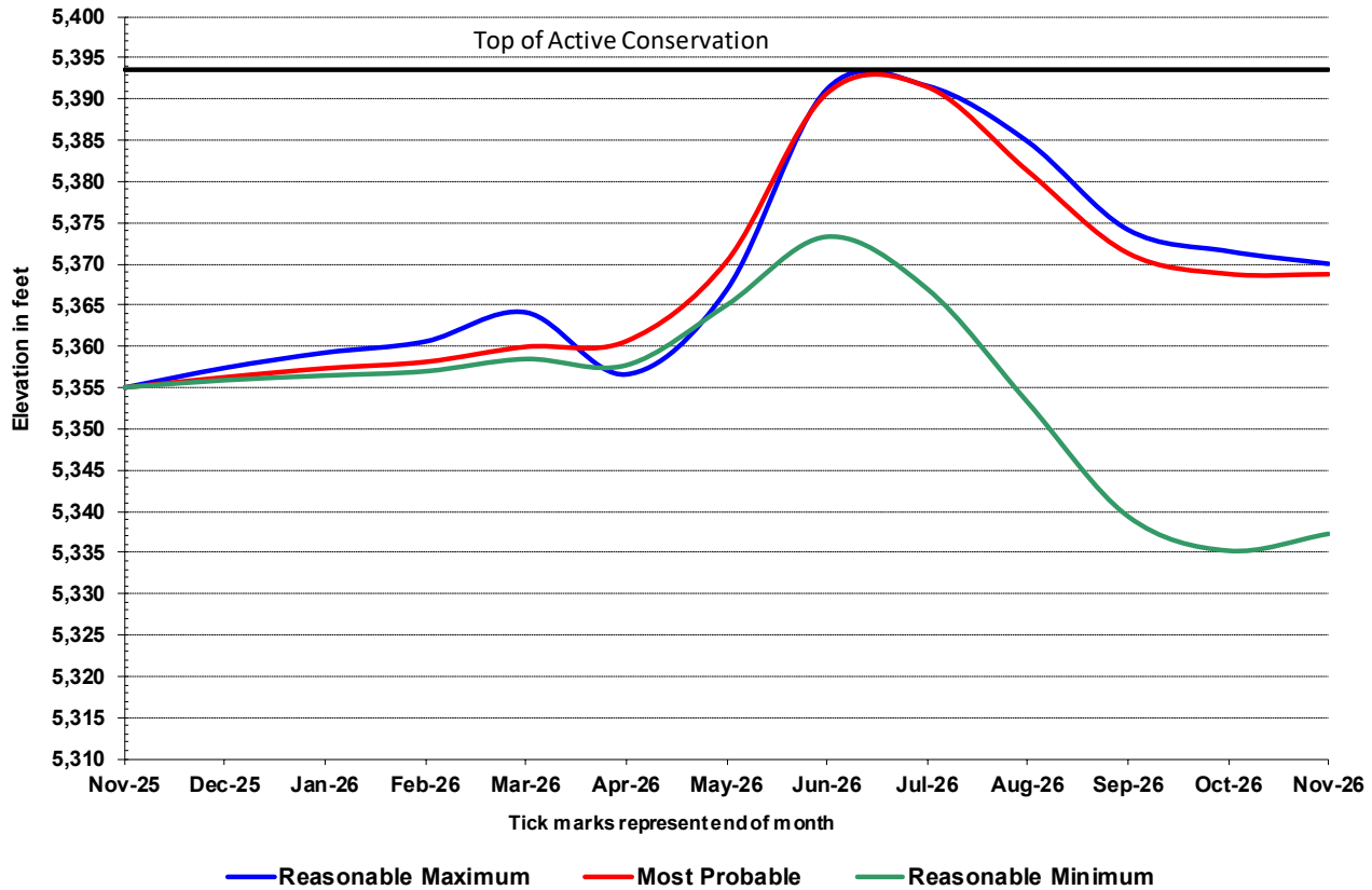
BUFFALO BILL RESERVOIR ELEVATION
