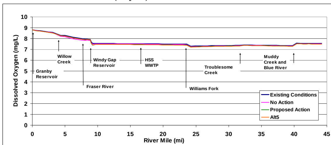
Figure 32. Colorado River dissolved oxygen concentrations predicted for Existing Conditions and alternatives (July 25)—cumulative effects.
