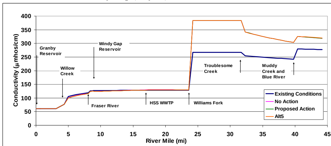
Figure 30. Colorado River average daily stream specific conductivity predicted for Existing Conditions and all alternatives assuming diversion to the minimum instream flow below Windy Gap (July 25)—cumulative effects.
