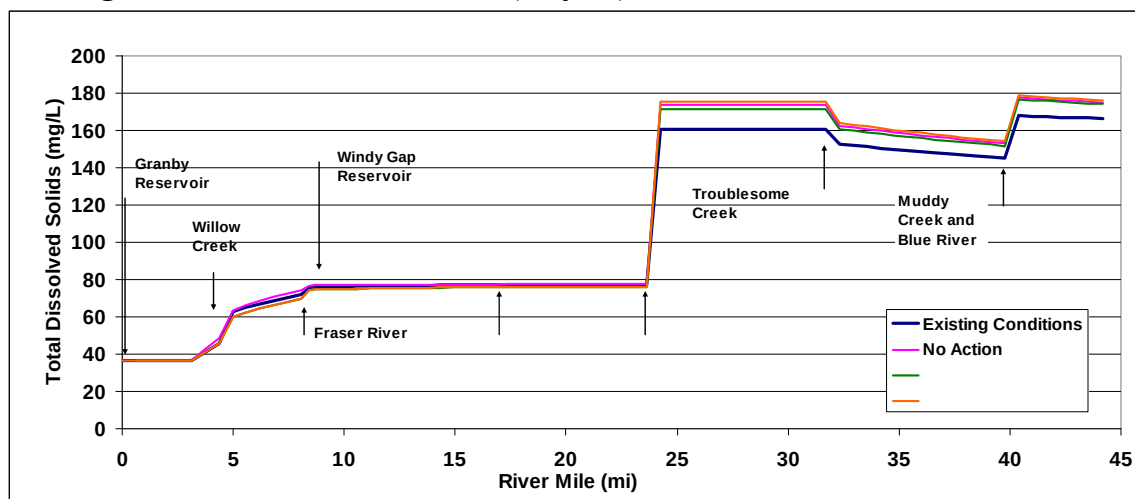
Figure 29. Colorado River total dissolved solids concentrations predicted for Existing Conditions and alternatives (July 25)—cumulative effects.
