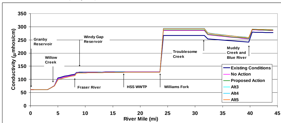
Figure 12. Colorado River specific conductivity predicted for Existing Conditions and all alternatives (July 25).
