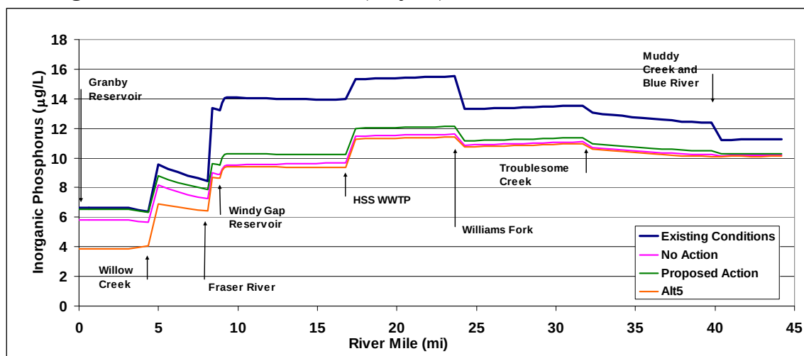
Figure 36. Colorado River inorganic phosphorus concentrations predicted for Existing Conditions and alternatives (July 25)—cumulative effects.
