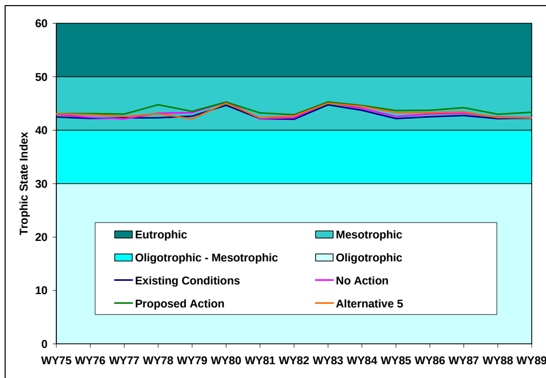
Figure 178: Predicted Trophic State Indices in Horsetooth Reservoir--Cumulative Effects
