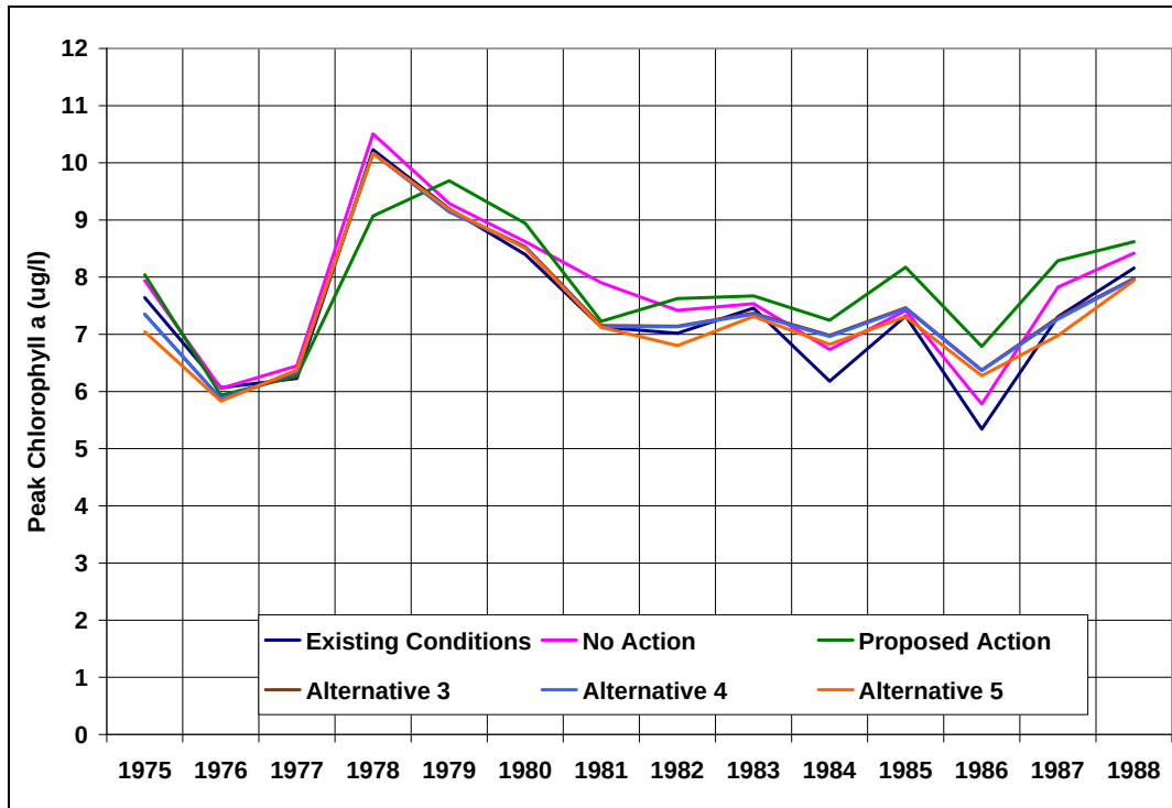
Figure 75: Predicted Peak Chlorophyll a Concentrations in Grand Lake by Year (Existing Conditions and the Alternatives)
