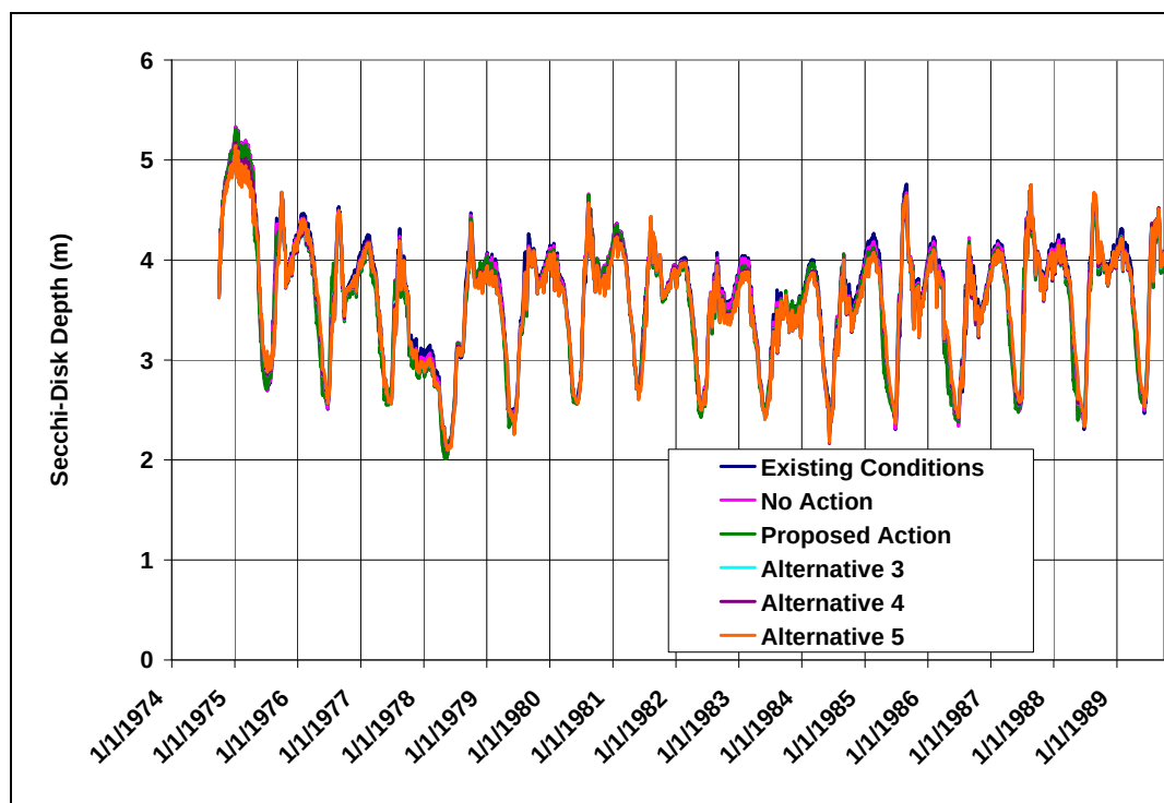
Figure 45: Predicted Daily Secchi-Disk Depth in Granby Reservoir (Existing Conditions and All Alternatives)
