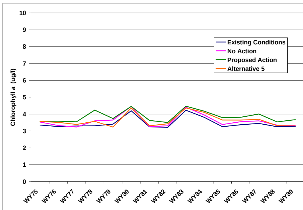
Figure 176: Predicted Chlorophyll a Concentrations in Horsetooth Reservoir--Cumulative Effects
