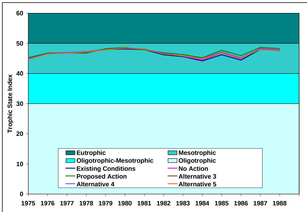
Figure 80: Predicted Trophic State Indices in Grand Lake (Existing Conditions and All Alternatives)
