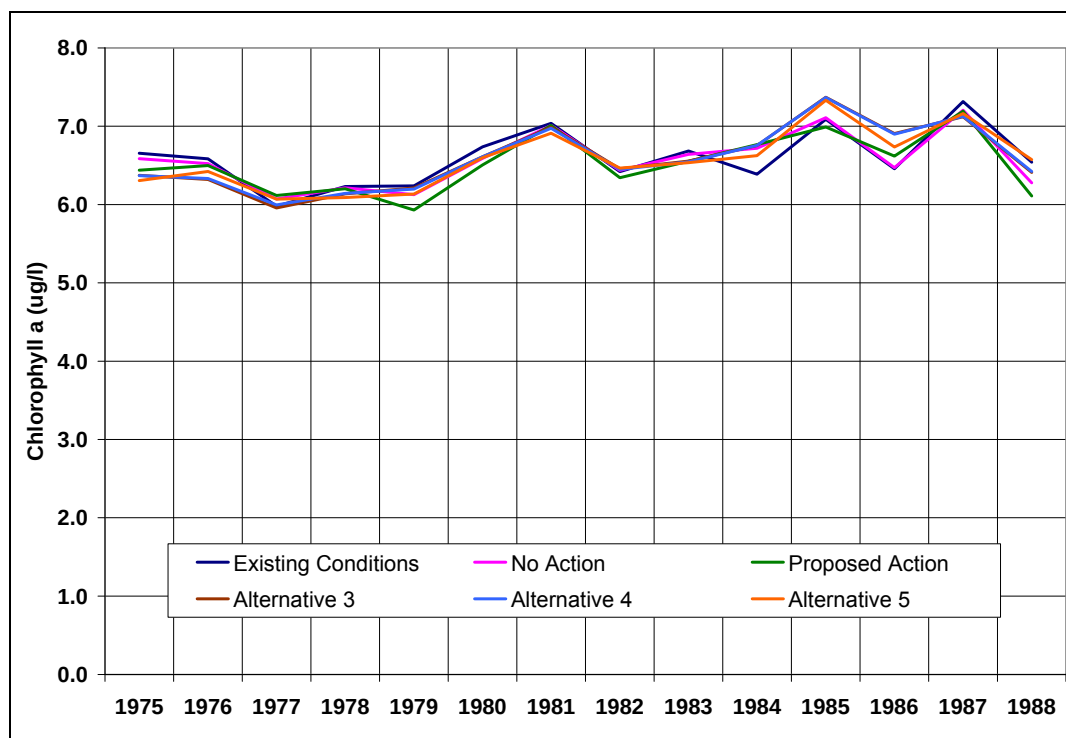
Figure 41: Simulated Annual Average Peak Chlorophyll a Concentrations in Granby Reservoir by Year for Existing Conditions and the Alternatives
