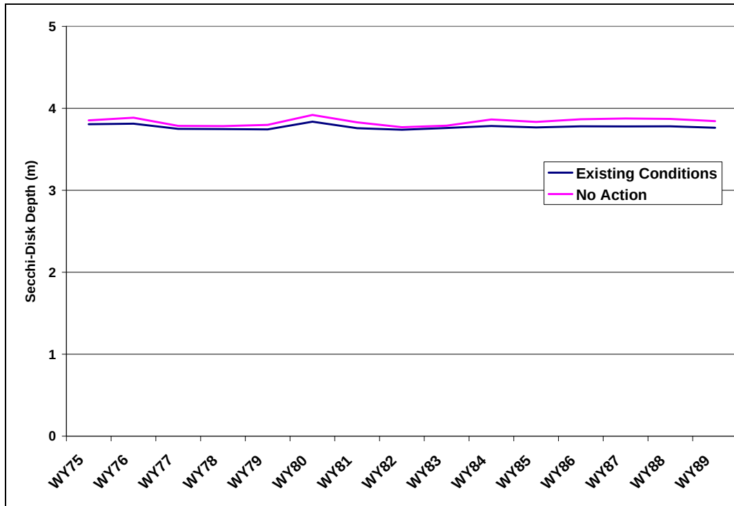
Figure 182: Predicted Secchi-Disk Depths in Ralph Price Reservoir--Cumulative Effects
