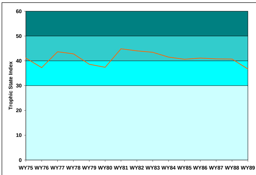
Figure 188: Predicted Annual Trophic State Indices in Rockwell Creek Reservoir--Cumulative Effects
