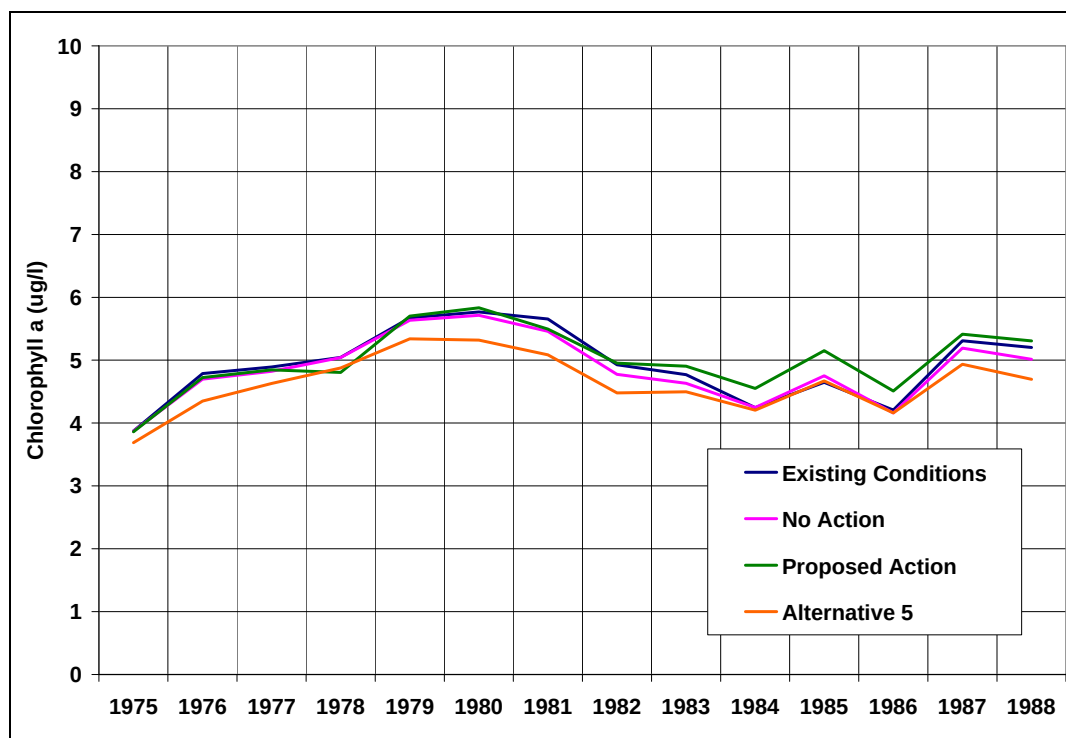
Figure 158: Predicted Average Annual Chlorophyll a Concentrations in Grand Lake--Cumulative Effects
