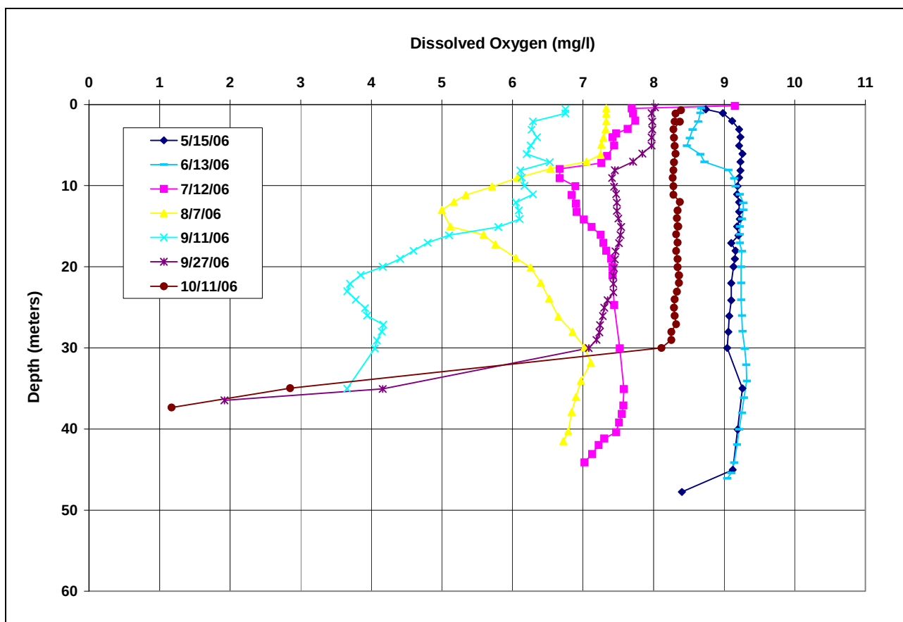
Figure 27: Dissolved Oxygen Profiles for Horsetooth Reservoir in 2006 (Site: Soldier Canyon Dam) (Data Sources: USGS, 2007; NCWCD, 2007b)
