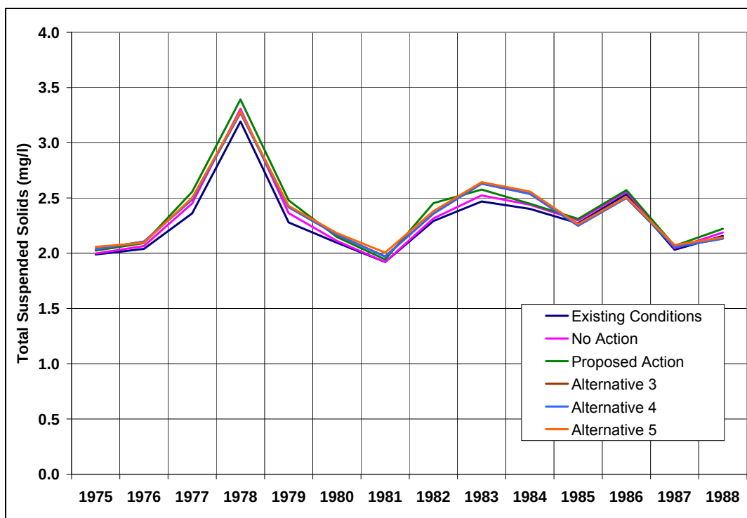
Figure 50: Predicted Annual Average Total Suspended Sediment Concentration in Granby Reservoir Epilimnion (Existing Conditions and All Alternatives)
