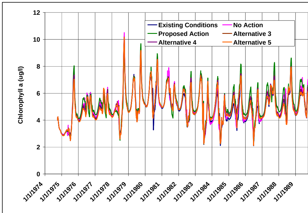
Figure 76: Predicted Daily Chlorophyll a Concentrations in Grand Lake (Existing Conditions and the Alternatives)
