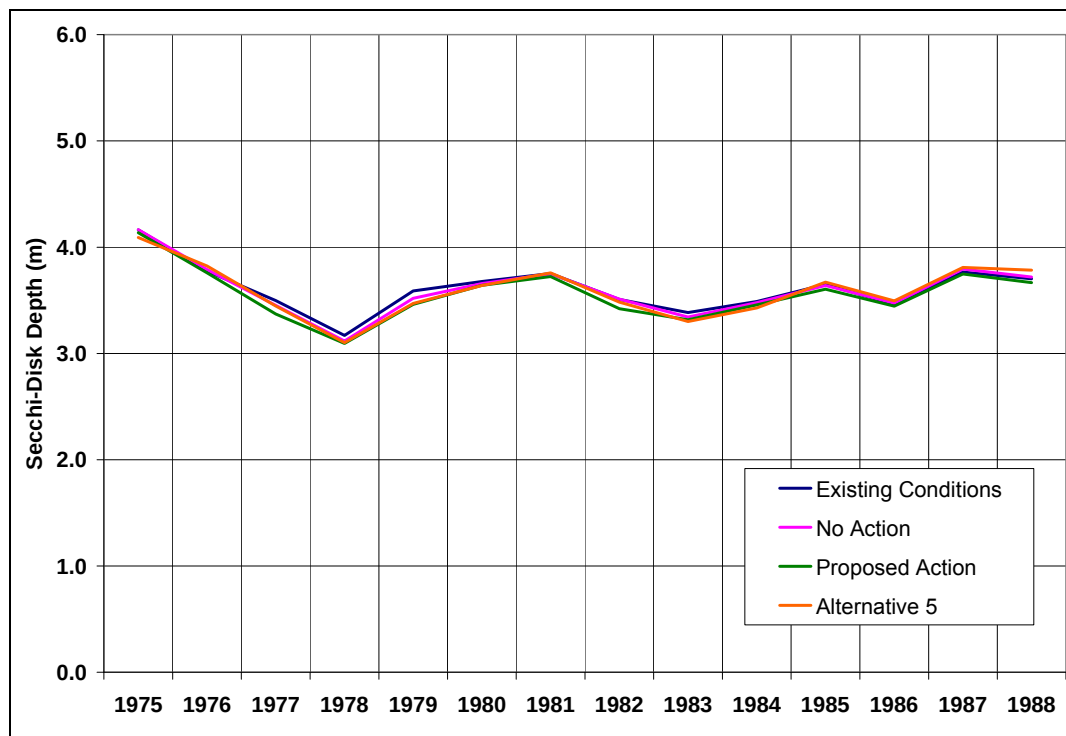
Figure 128: Predicted Average Annual Secchi-Disk Depths in Granby Reservoir--Cumulative Effects
