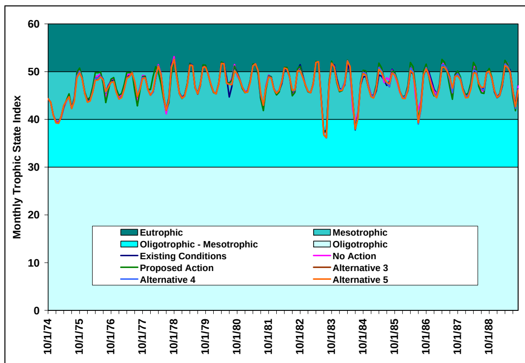
Figure 65: Predicted Monthly Trophic State Index for Shadow Mountain Reservoir
