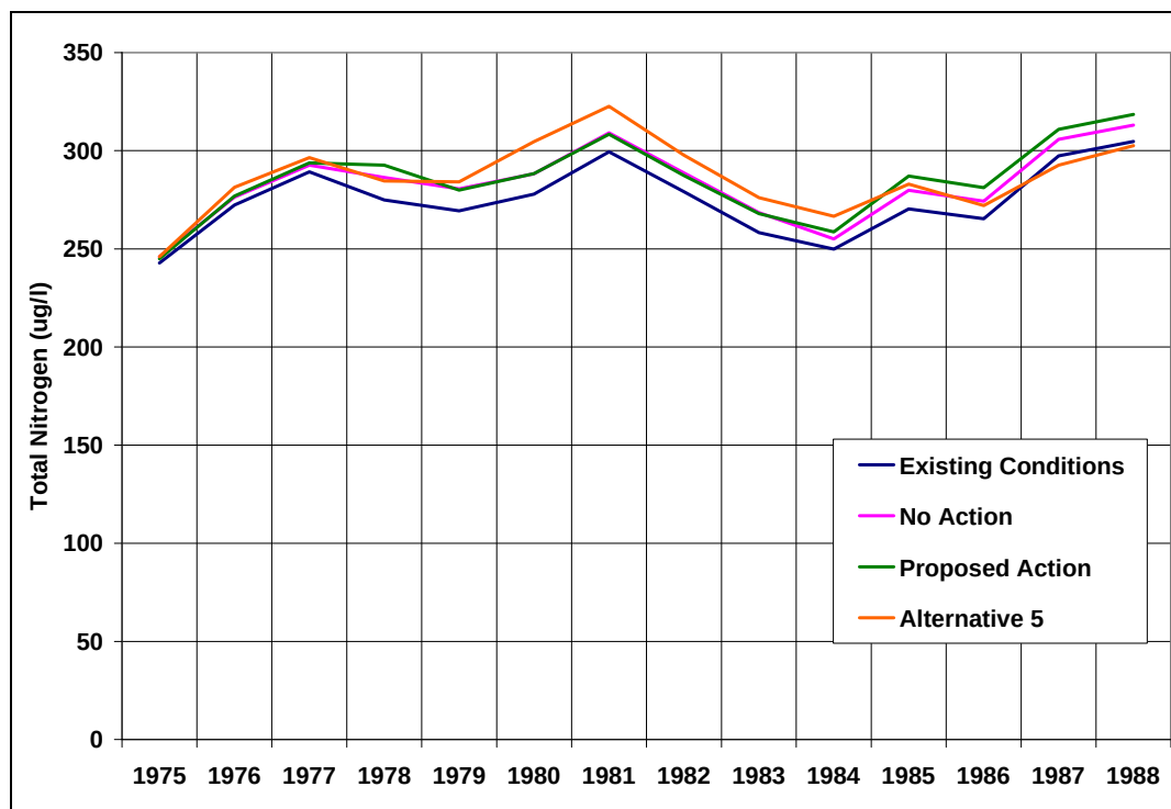
Figure 140: Predicted Average Annual Total Nitrogen Concentrations in Shadow Mountain Reservoir--Cumulative Effects
