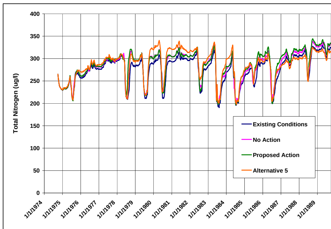
Figure 141: Predicted Daily Total Nitrogen Concentrations in Shadow Mountain Reservoir--Cumulative Effects
