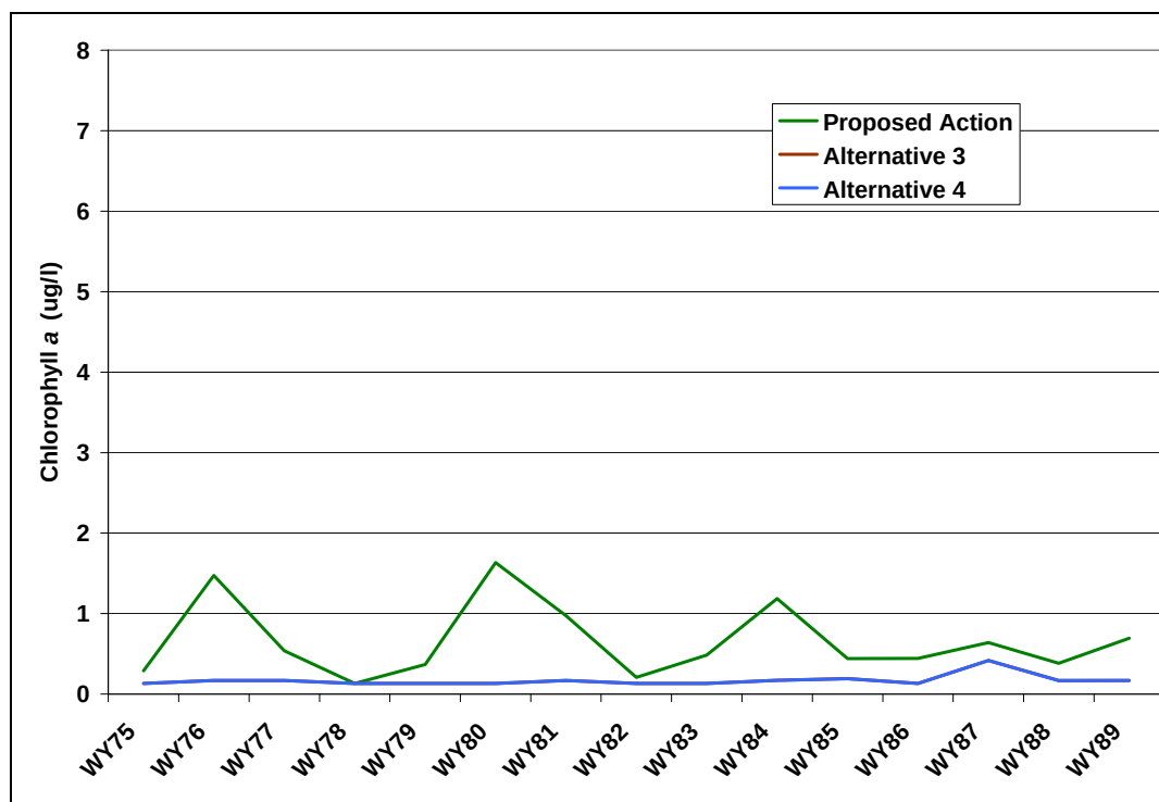
Figure 113: Predicted Annual Average Chlorophyll a Concentrations in Chimney Hollow Reservoir (Proposed Action and Alternatives 3 and 4)
