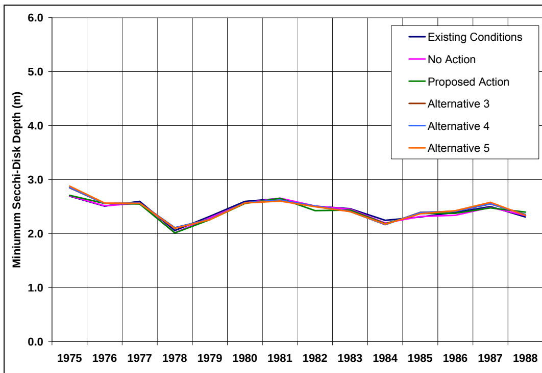
Figure 44: Predicted Minimum Secchi-Disk Depth in Granby Reservoir (Existing Conditions and All Alternatives)
