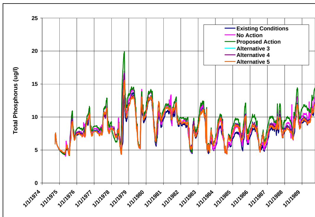
Figure 71: Predicted Daily Total Phosphorus Concentrations in Grand Lake Epilimnion (Existing Conditions and All Alternatives)
