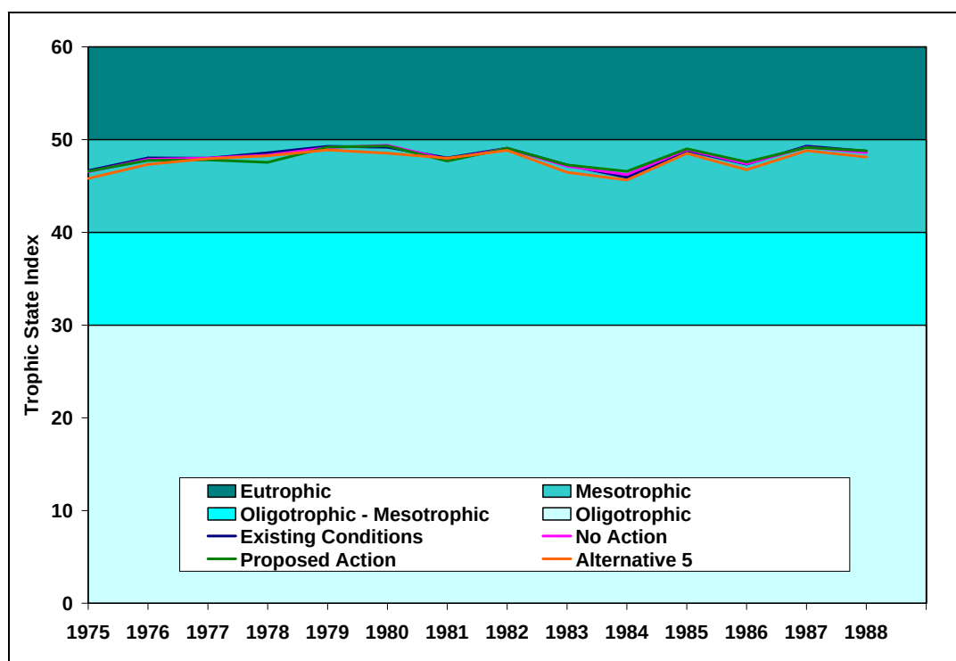
Figure 148: Predicted Annual Trophic State Indices in Shadow Mountain Reservoir--Cumulative Effects
