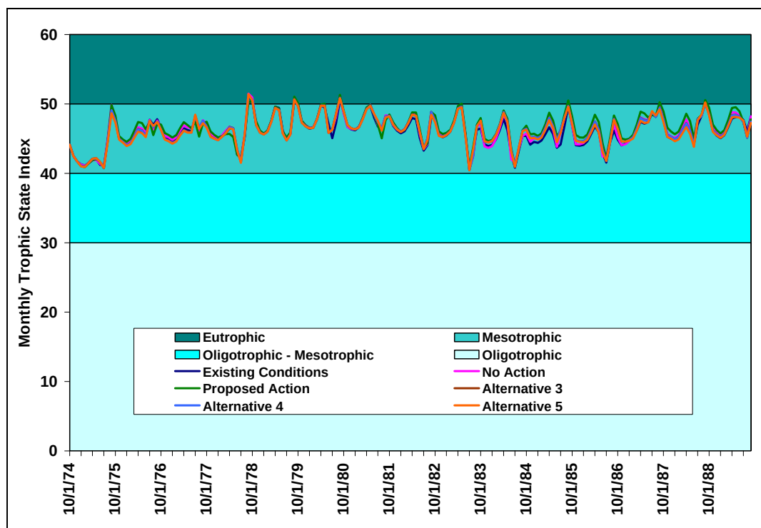
Figure 81: Predicted Monthly Trophic State Index for Grand Lake
