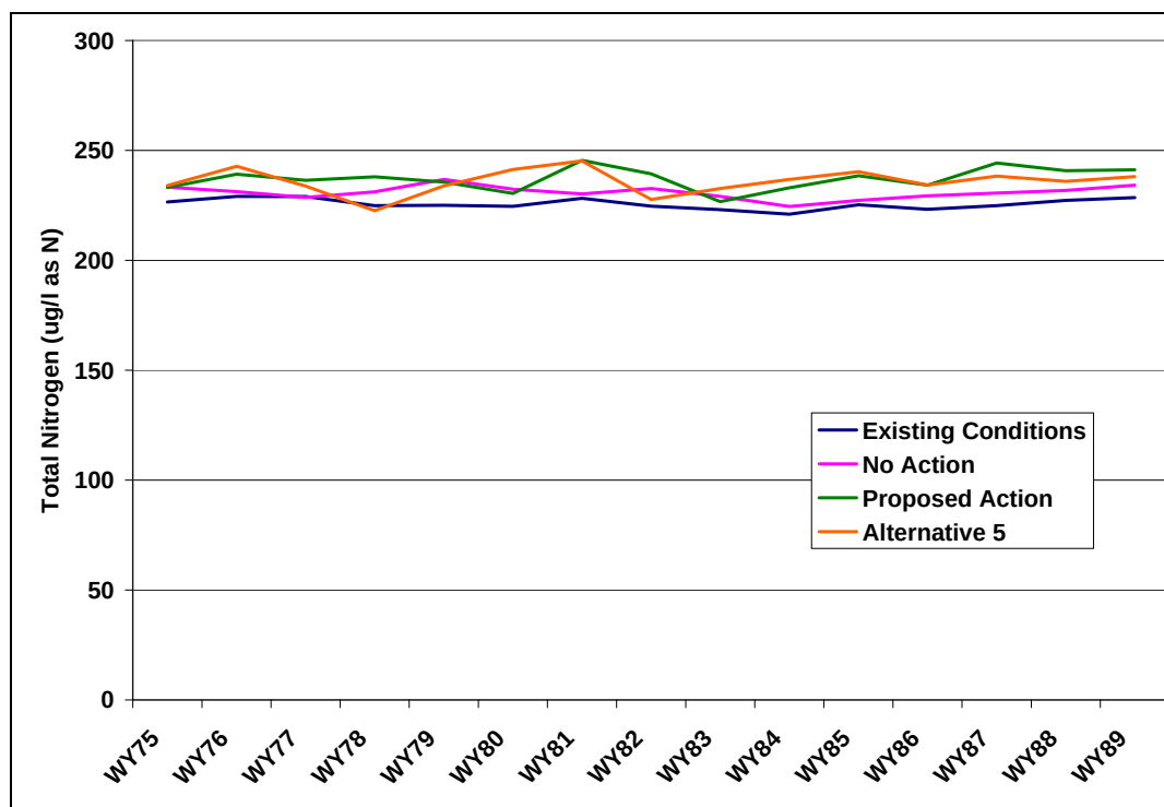
Figure 170: Predicted Total Nitrogen Concentrations in Carter Lake--Cumulative Effects
