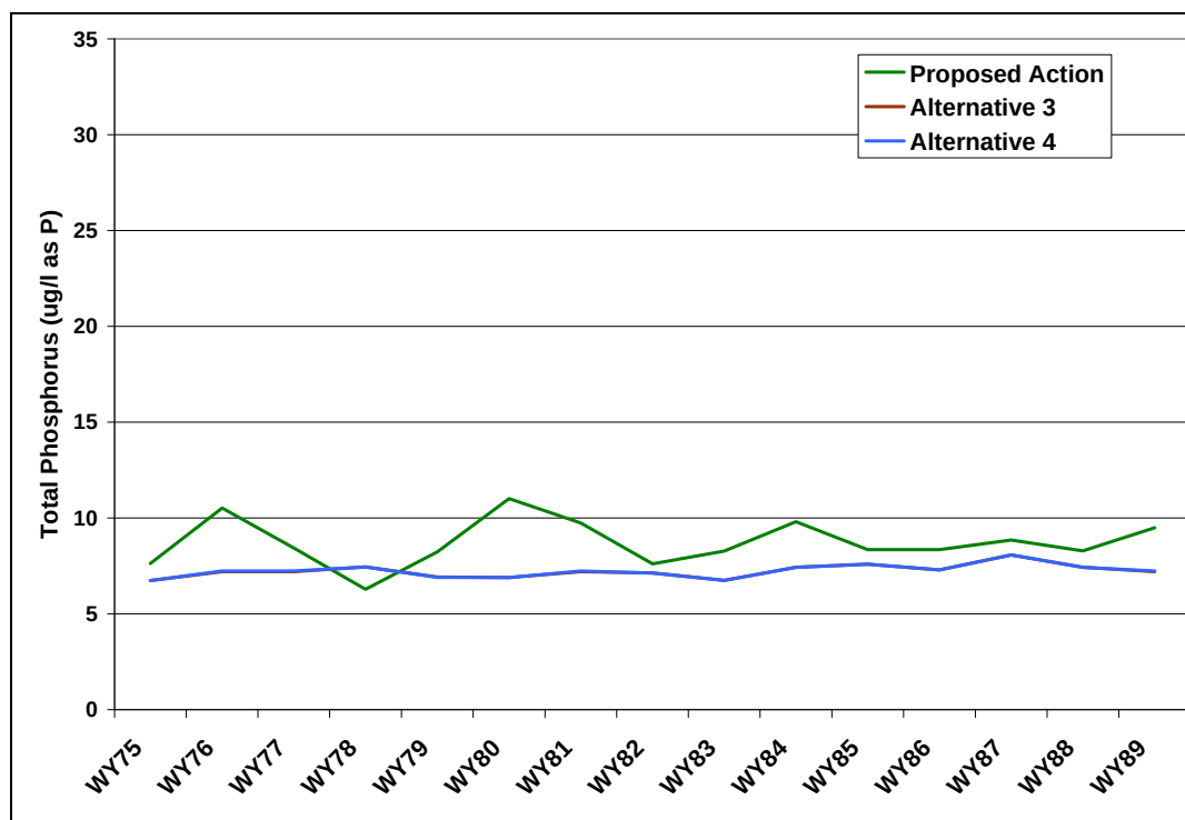
Figure 111: Predicted Annual Average Total Phosphorus Concentrations in Chimney Hollow Reservoir (Proposed Action and Alternatives 3 and 4)
