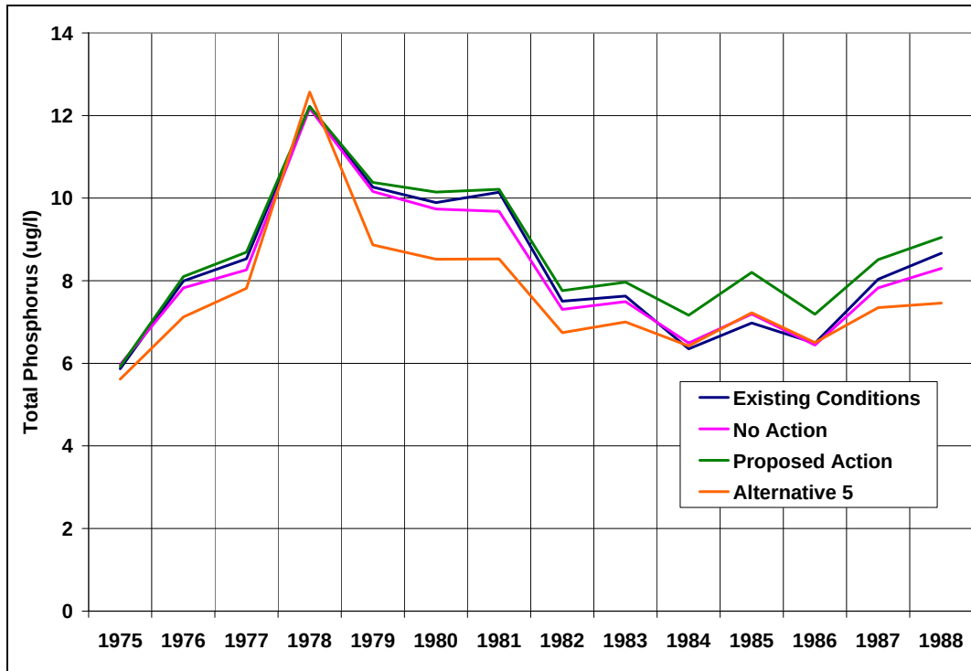
Figure 154: Predicted Average Annual Total Phosphorus Concentrations in Grand Lake--Cumulative Effects
