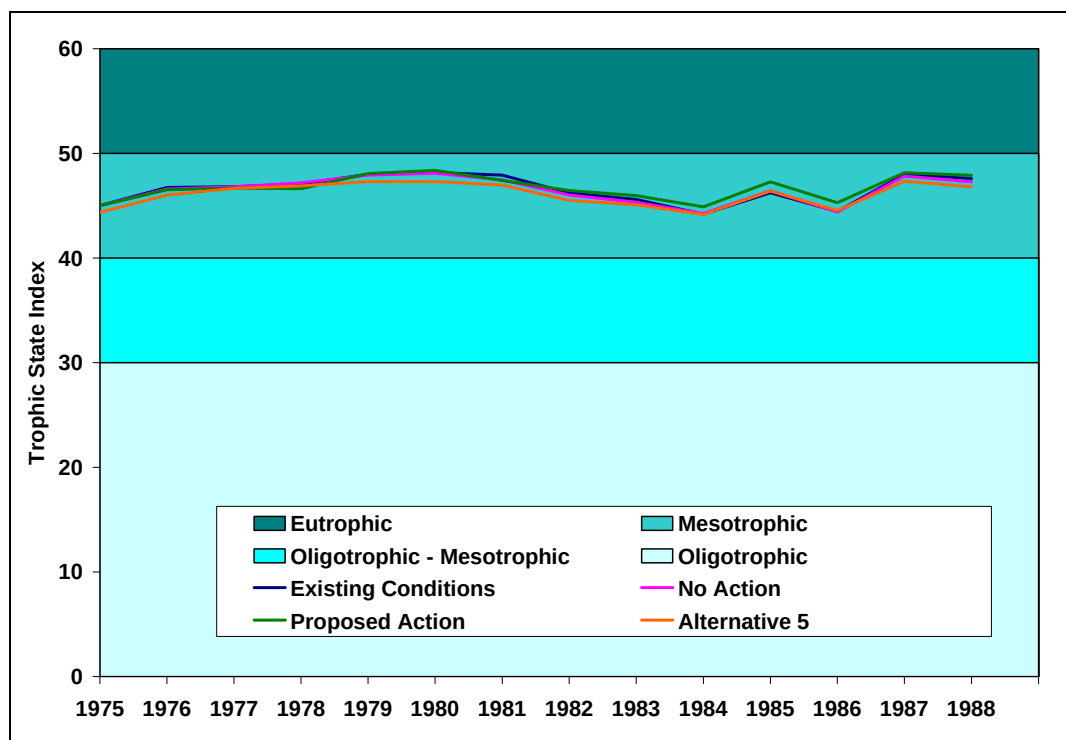
Figure 164: Predicted Annual Trophic State Indices in Grand Lake--Cumulative Effects
