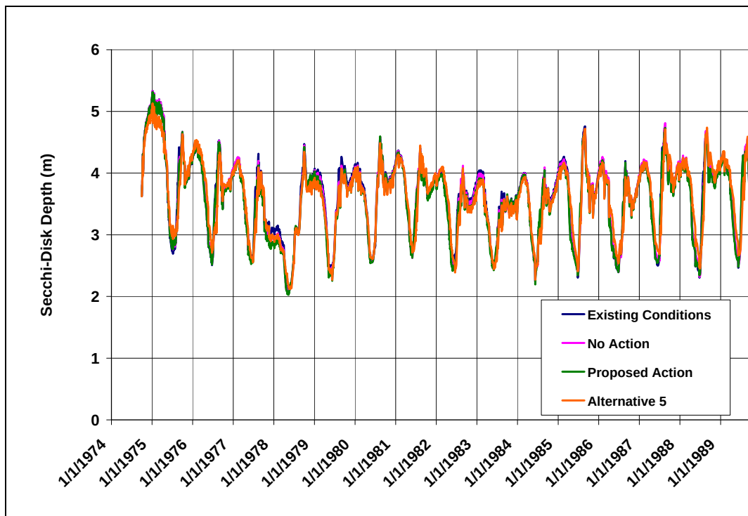
Figure 130: Predicted Daily Secchi-Disk Depths in Granby Reservoir--Cumulative Effects
