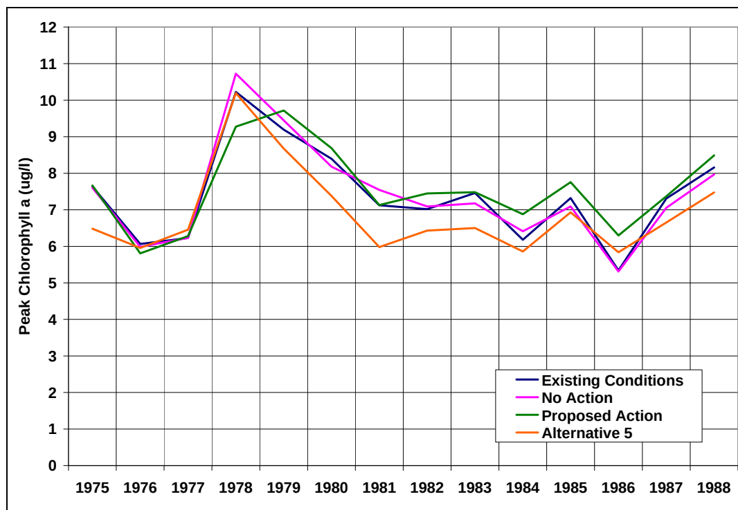
Figure 159: Predicted Annual Peak Chlorophyll a Concentrations in Grand Lake--Cumulative Effects
