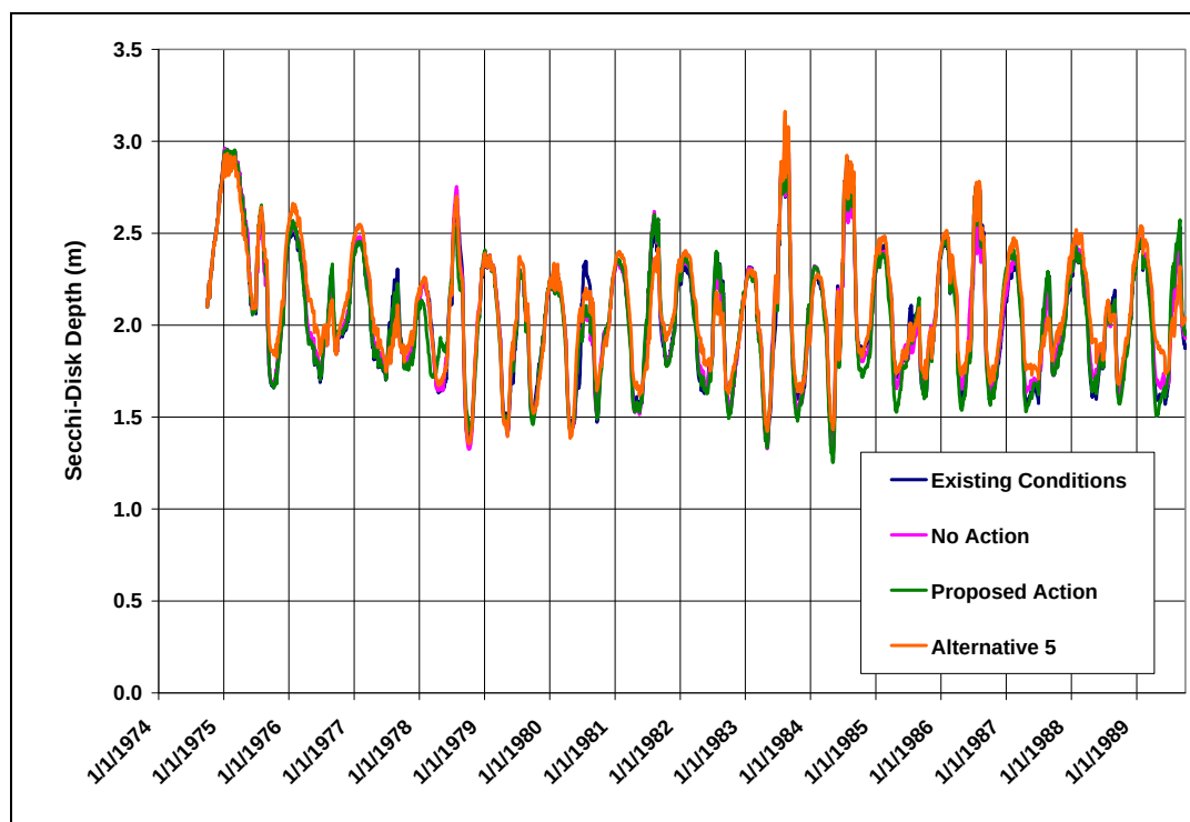
Figure 147: Predicted Daily Secchi-Disk Depth in Shadow Mountain Reservoir--Cumulative Effects
