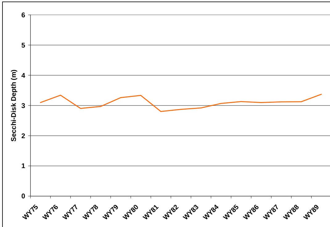
Figure 187: Predicted Secchi-Disk Depth in Rockwell Creek Reservoir--Cumulative Effects
