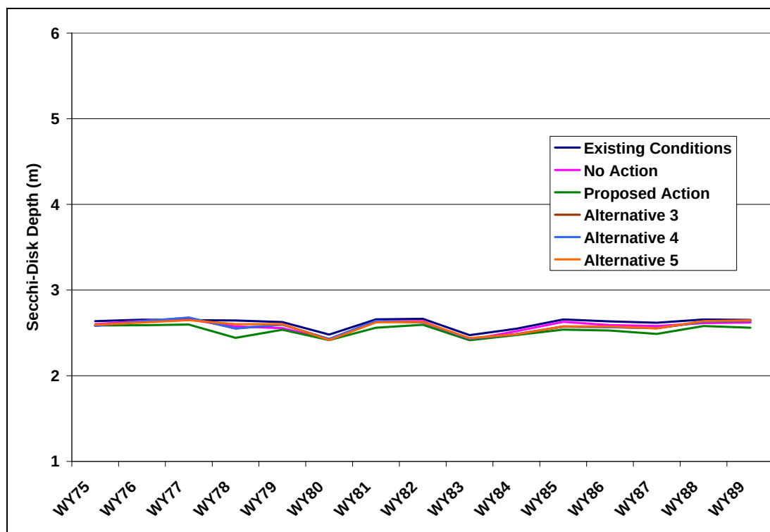
Figure 94: Predicted Annual Average Secchi-Disk Depths in Horsetooth Reservoir (Existing Conditions and All Alternatives)
