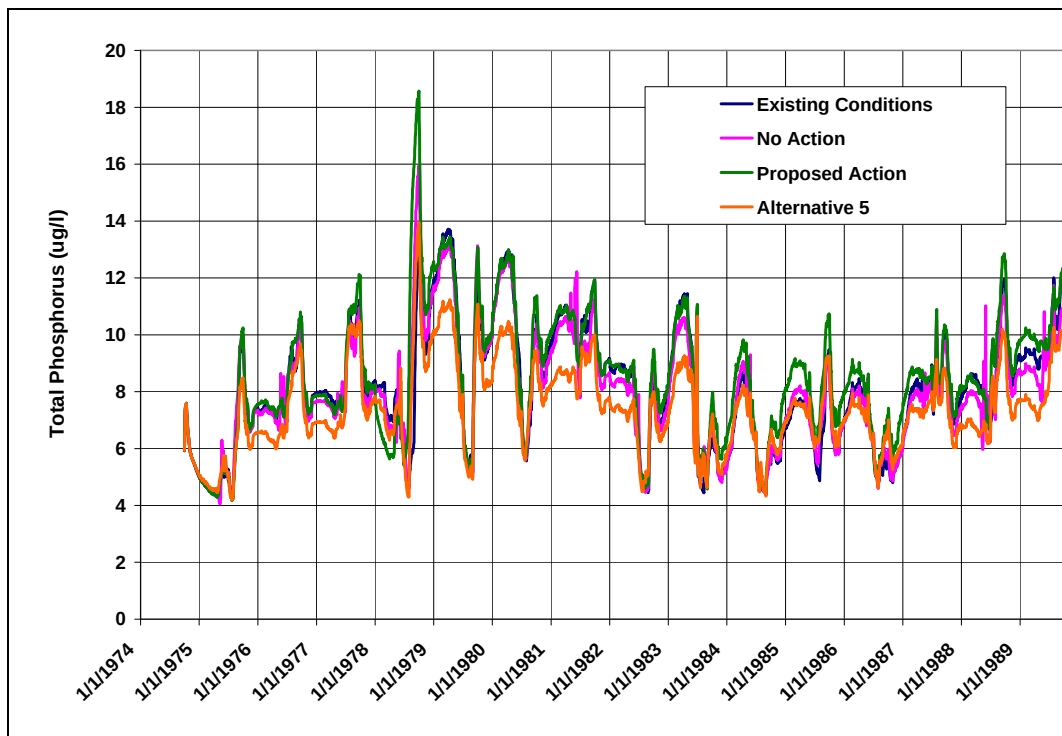
Figure 155: Predicted Daily Total Phosphorus Concentrations in Grand Lake--Cumulative Effects
