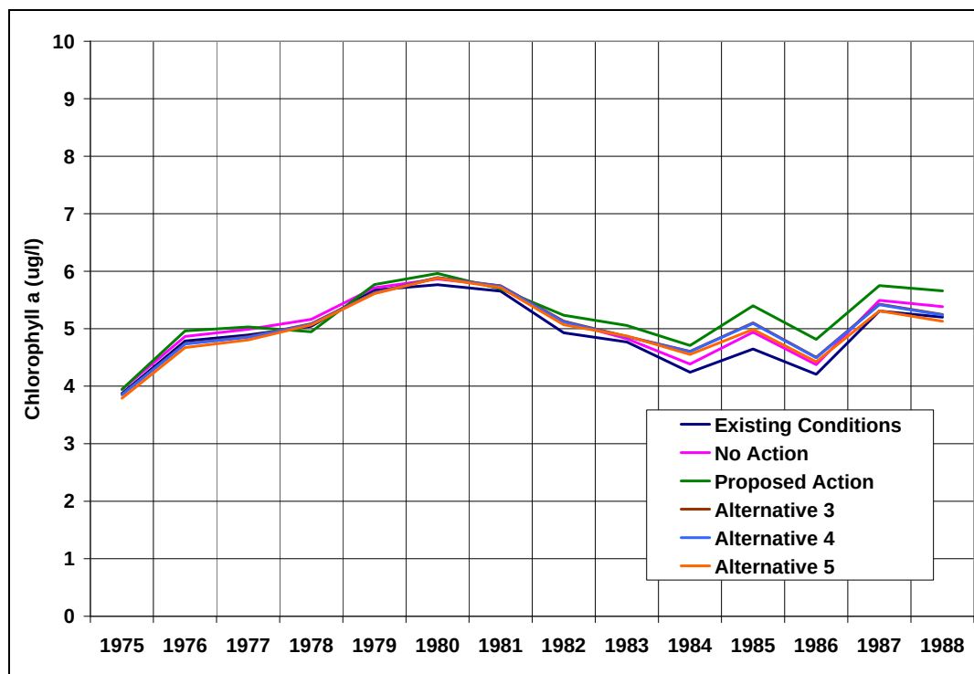
Figure 74: Predicted Annual Average Chlorophyll a Concentrations in Grand Lake (Existing Conditions and All Alternatives)
