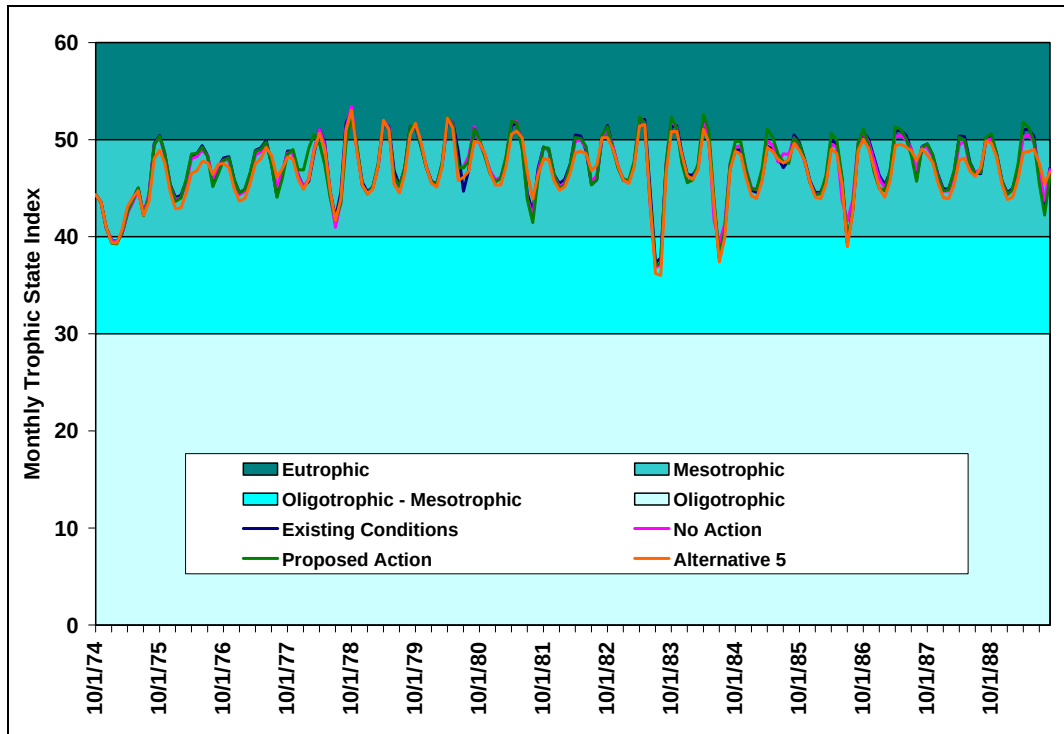
Figure 149: Predicted Monthly Trophic State Index for Shadow Mountain Reservoir--Cumulative Effects
