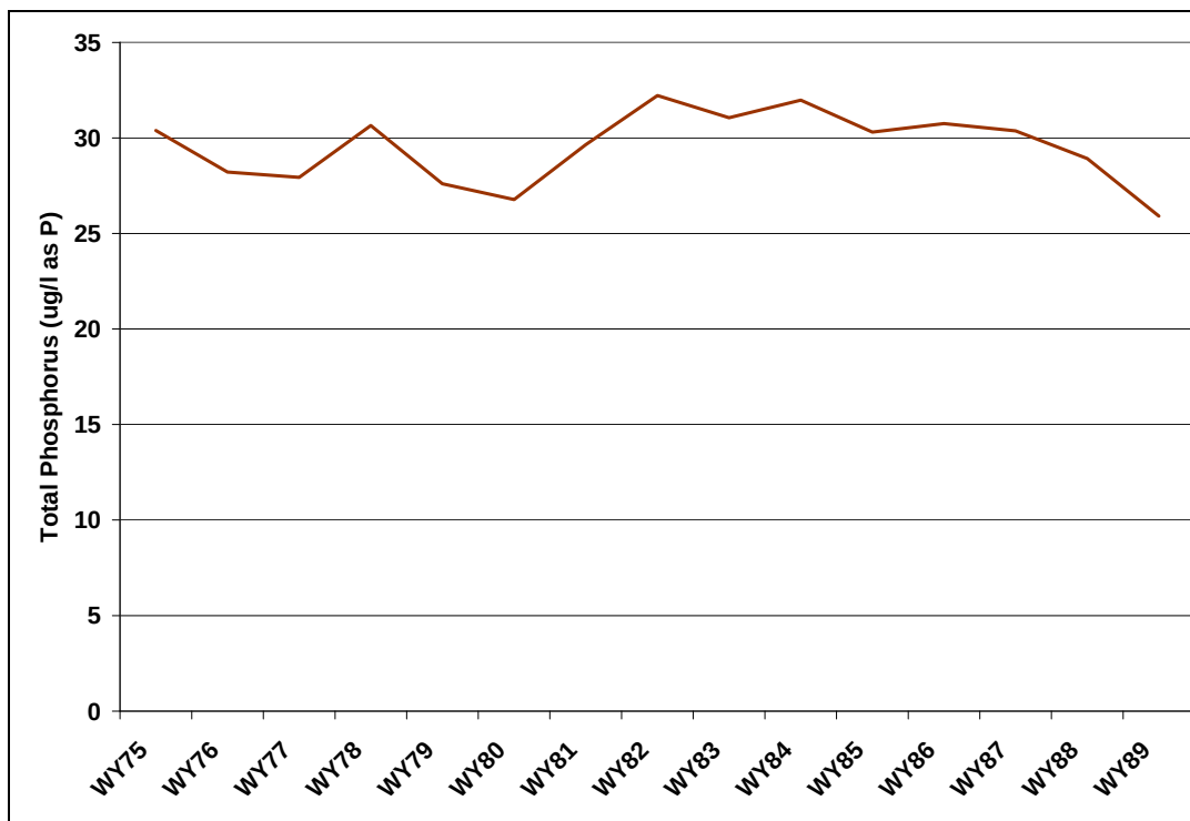
Figure 101: Predicted Annual Average Total Phosphorus Concentrations in Jasper East Reservoir (Alternative 3)
