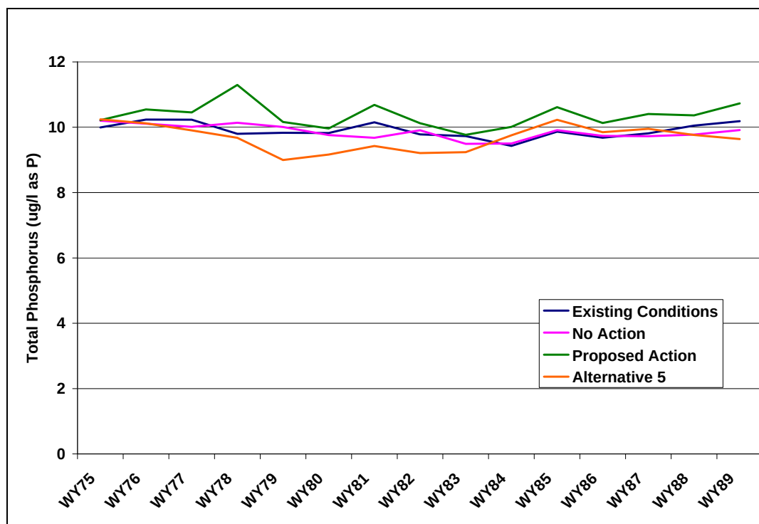
Figure 169: Predicted Total Phosphorus Concentrations in Carter Lake--Cumulative Effects
