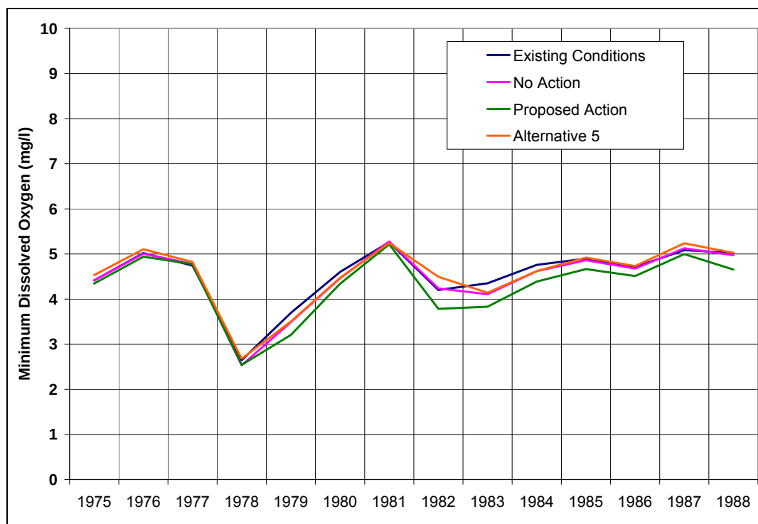
Figure 133: Predicted Minimum Dissolved Oxygen Concentrations in Granby Reservoir Hypolimnion--Cumulative Effects
