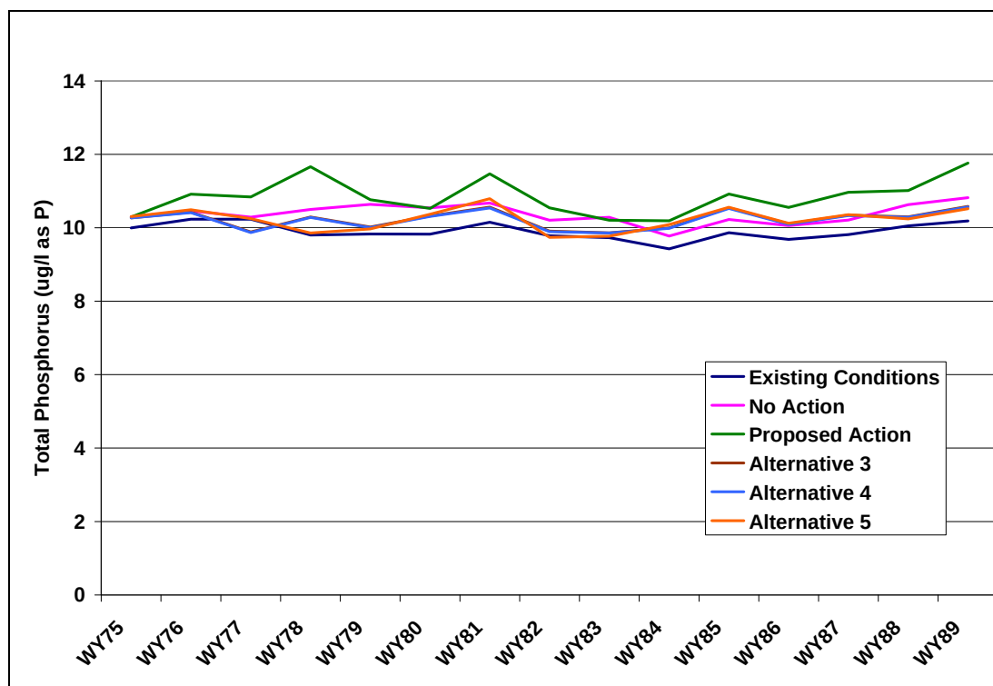
Figure 86: Predicted Annual Average Total Phosphorus Concentrations in Carter Lake (Existing Conditions and All Alternatives)
