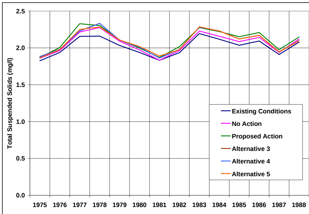
Figure 68: Predicted Annual Average Total Suspended Sediment Concentration in Shadow Mountain Reservoir (Existing Conditions and All Alternatives)
