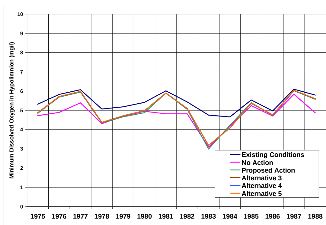
Figure 82: Predicted Minimum Dissolved Oxygen Concentration in Grand Lake (Existing Conditions and All Alternatives)
