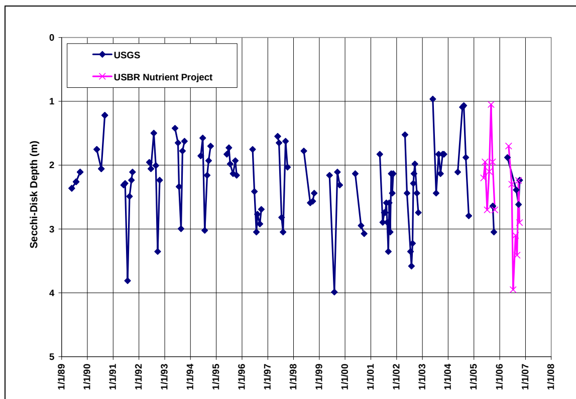
Figure 12: Shadow Mountain Reservoir Secchi-Disk Depth
