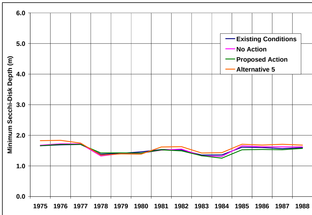
Figure 146: Predicted Minimum Secchi-Disk Depth in Shadow Mountain Reservoir--Cumulative Effects
