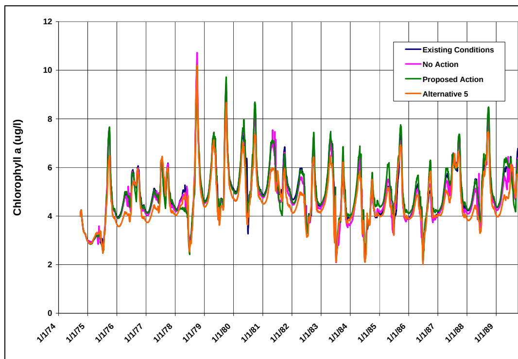
Figure 160: Predicted Daily Chlorophyll a Concentrations in Grand Lake--Cumulative Effects
