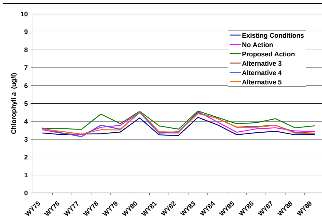
Figure 93: Predicted Annual Average Chlorophyll a Concentrations in Horsetooth Reservoir (Existing Conditions and All Alternatives)
