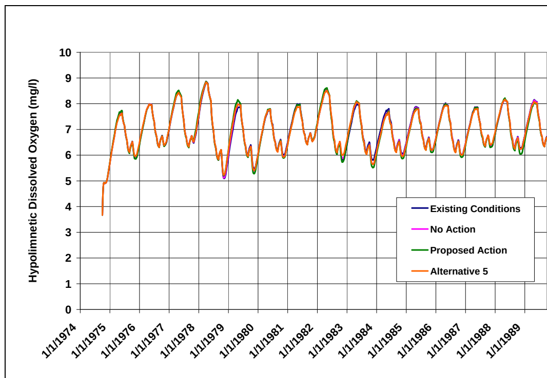
Figure 134: Predicted Daily Dissolved Oxygen Concentrations in Granby Reservoir Hypolimnion--Cumulative Effects
