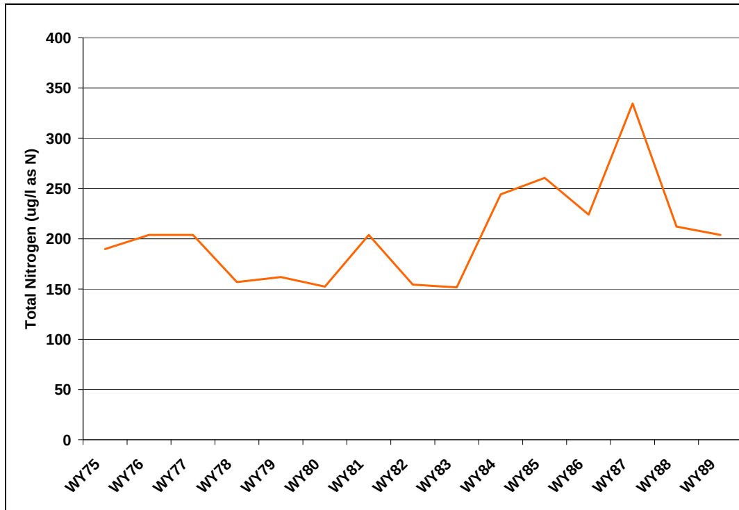
Figure 117: Predicted Annual Average Total Nitrogen Concentrations in Dry Creek Reservoir (Alternative 5)
