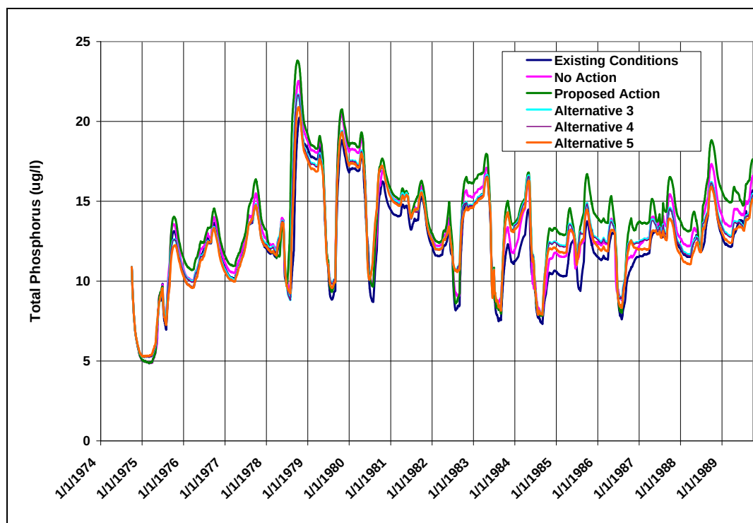
Figure 55: Predicted Daily Total Phosphorus Concentrations in Shadow Mountain Reservoir (Existing Conditions and All Alternatives)
