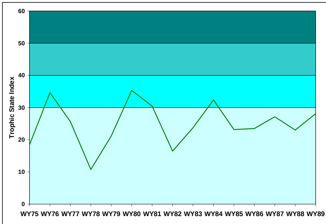
Figure 193: Predicted Annual Trophic State Indices in Chimney Hollow Reservoir (Cumulative Effects Proposed Action)
