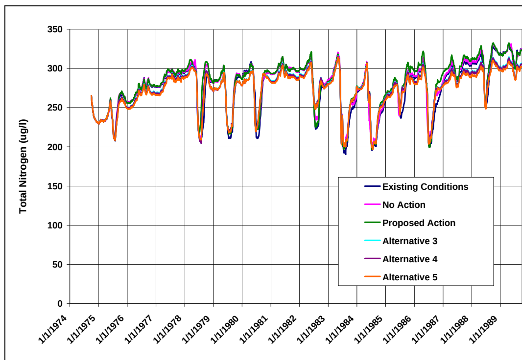
Figure 57: Predicted Daily Total Nitrogen Concentrations in Shadow Mountain Reservoir (Existing Conditions and All Alternatives)
