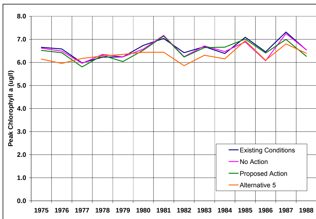
Figure 126: Predicted Annual Peak Chlorophyll a Concentrations in Granby Reservoir--Cumulative Effects
