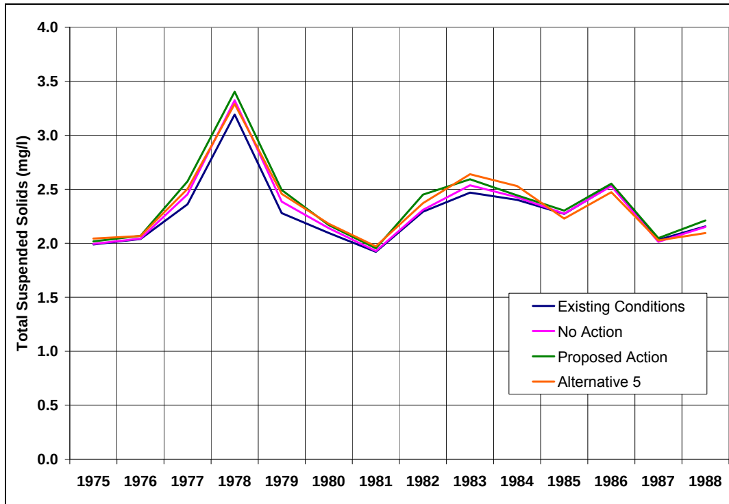
Figure 135: Predicted Average Annual Total Suspended Sediment Concentrations in Granby Reservoir--Cumulative Effects
