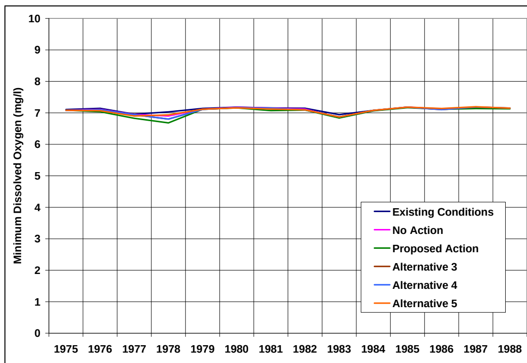
Figure 66: Predicted Minimum Dissolved Oxygen in Shadow Mountain Reservoir (Existing Conditions and All Alternatives)
