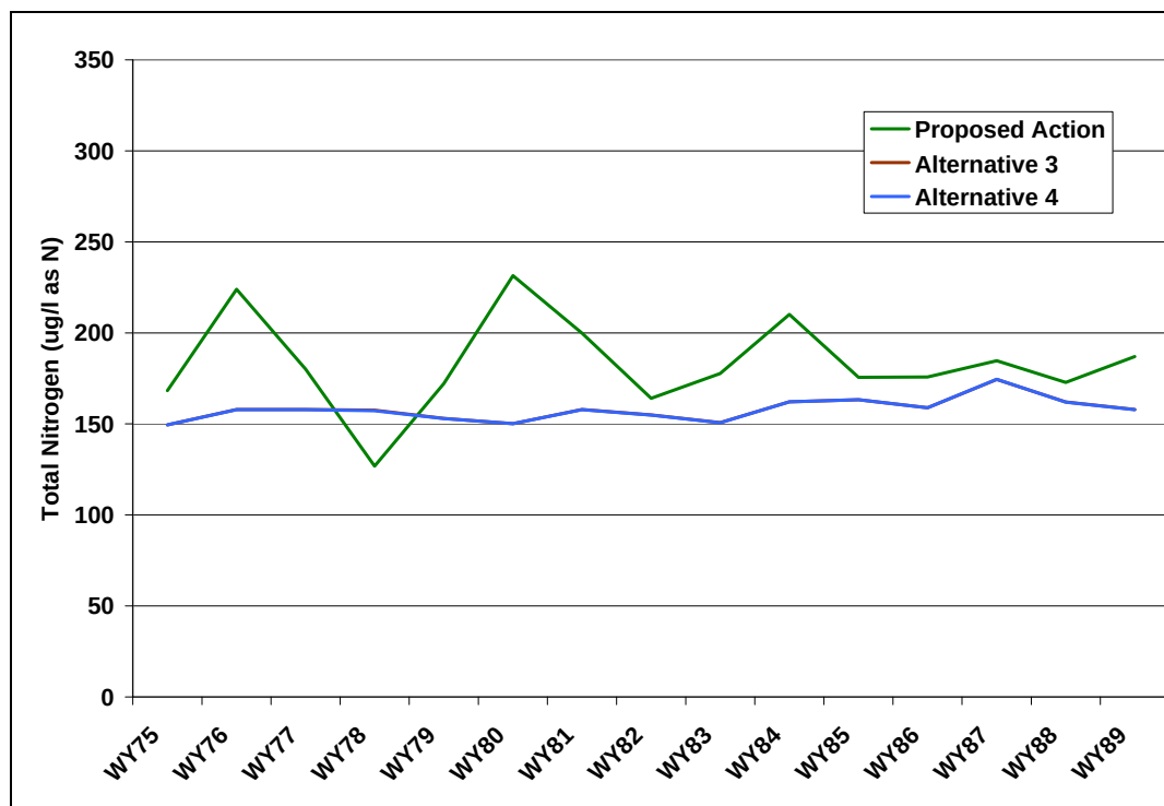
Figure 112: Predicted Annual Average Total Nitrogen Concentrations in Chimney Hollow Reservoir (Proposed Action and Alternatives 3 and 4)
