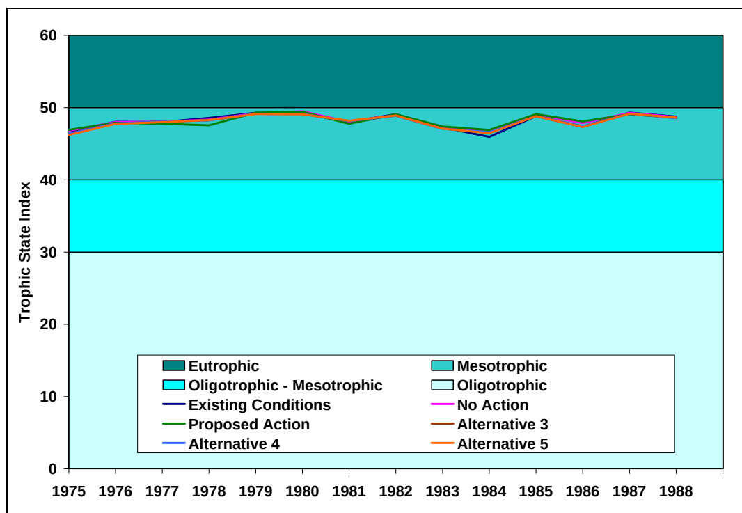
Figure 64: Predicted Trophic State Indices in Shadow Mountain Reservoir (Existing Conditions and All Alternatives)
