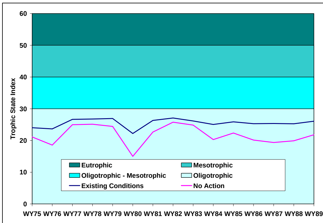
Figure 183: Predicted Annual Trophic State Indices in Ralph Price Reservoir--Cumulative Effects
