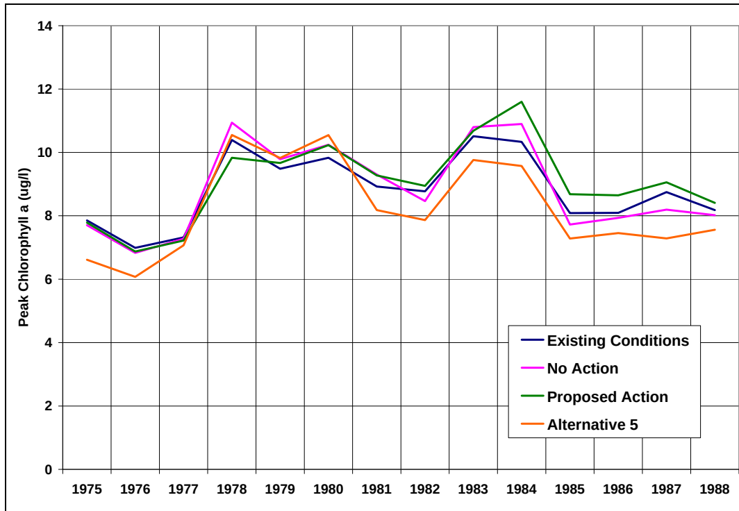
Figure 143: Predicted Annual Peak Chlorophyll a Concentrations in Shadow Mountain Reservoir--Cumulative Effects
