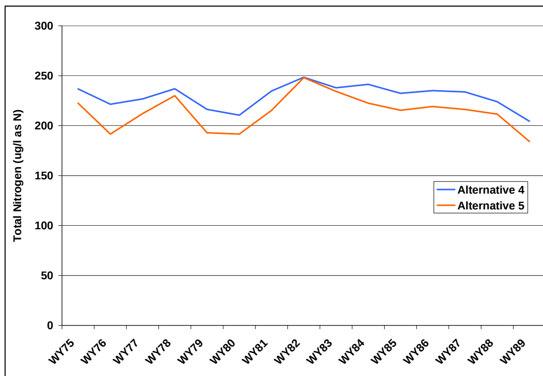
Figure 107: Predicted Annual Average Total Nitrogen Concentrations in Rockwell Creek Reservoir (Alternatives 4 and 5)
