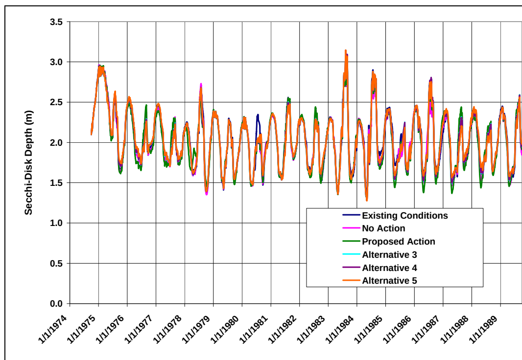
Figure 63: Predicted Daily Secchi-Disk Depths in Shadow Mountain Reservoir (Existing Conditions and All Alternatives)
