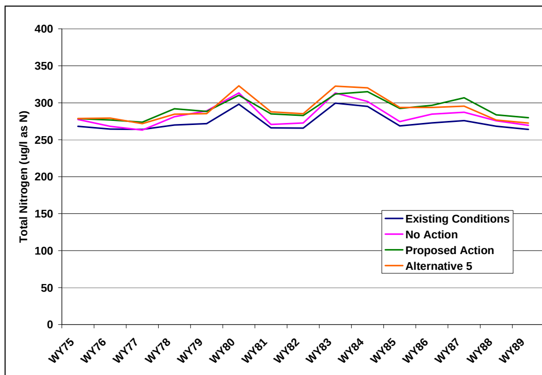
Figure 175: Predicted Total Nitrogen Concentrations in Horsetooth Reservoir--Cumulative Effects
