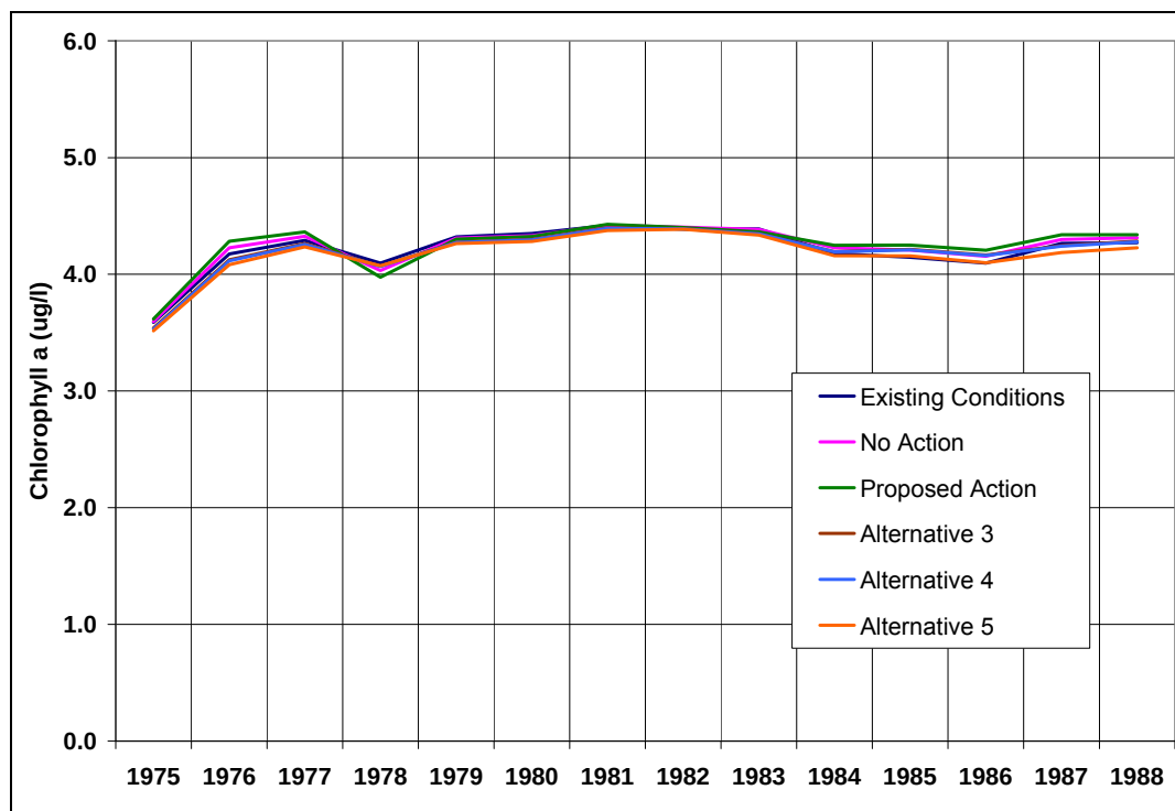
Figure 40: Predicted Annual Average Chlorophyll a Concentrations in Granby Reservoir (Existing Conditions and All Alternatives)
