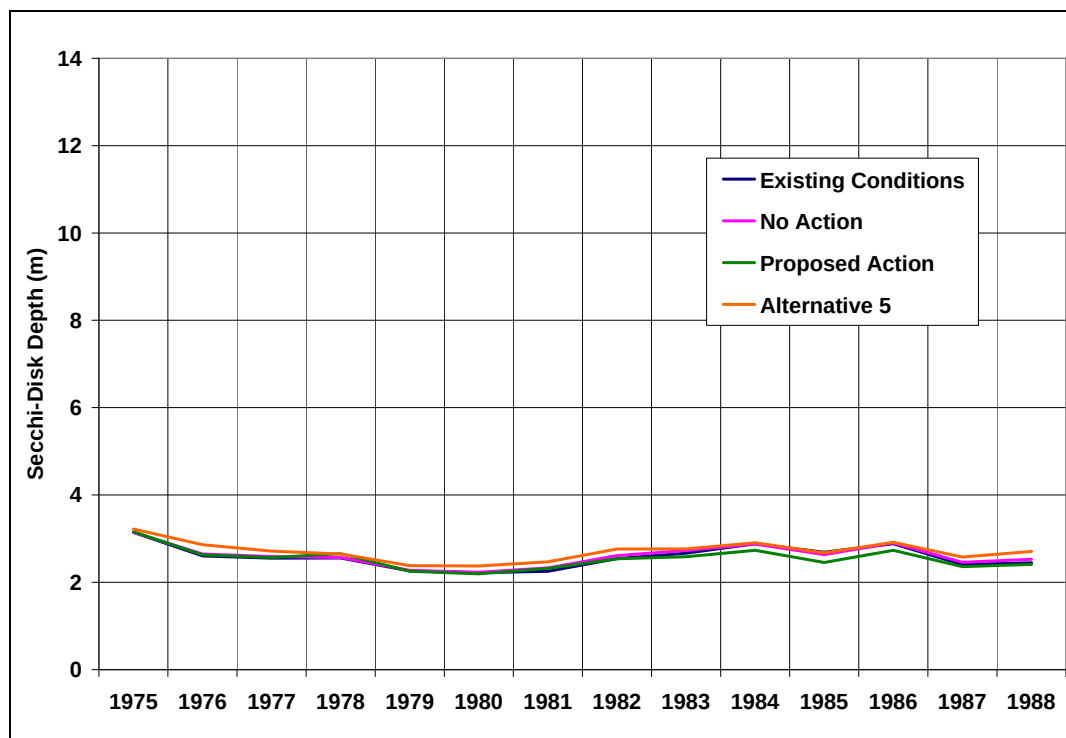
Figure 161: Predicted Average Annual Secchi-Disk Depth in Grand Lake--Cumulative Effects
