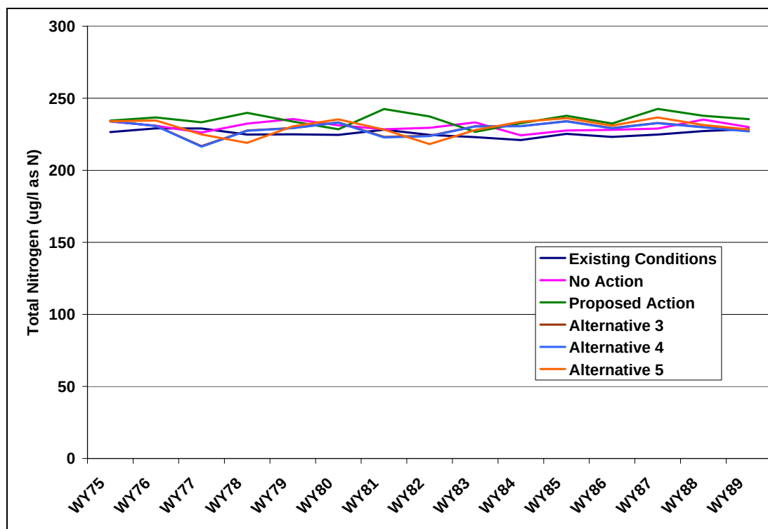
Figure 87: Predicted Annual Average Total Nitrogen Concentrations in Carter Lake (Existing Conditions and All Alternatives)
