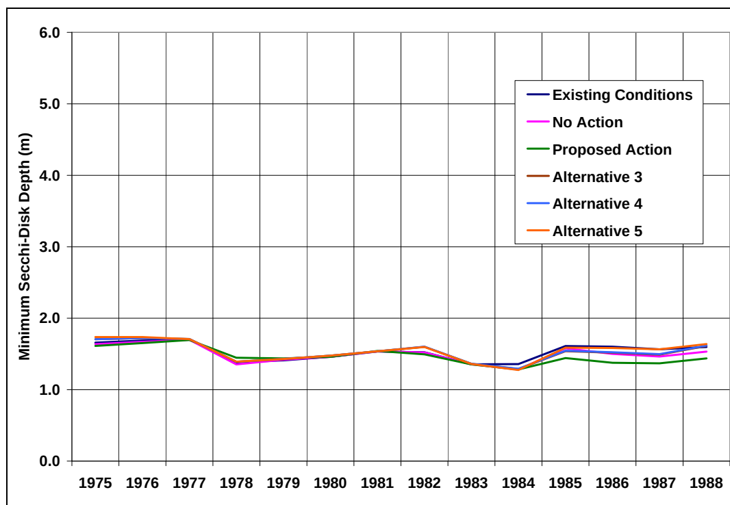
Figure 62: Predicted Minimum Secchi-Disk Depths in Shadow Mountain Reservoir (Existing Conditions and All Alternatives)
