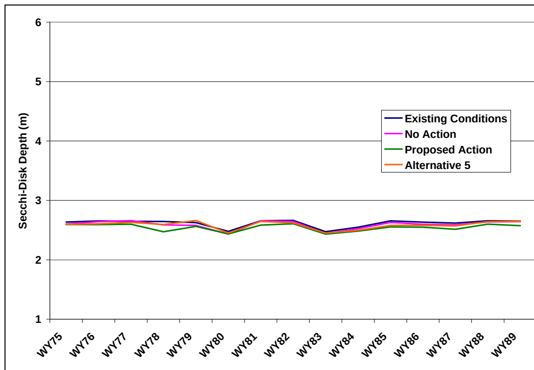
Figure 177: Predicted Secchi-Disk Depths in Horsetooth Reservoir--Cumulative Effects
