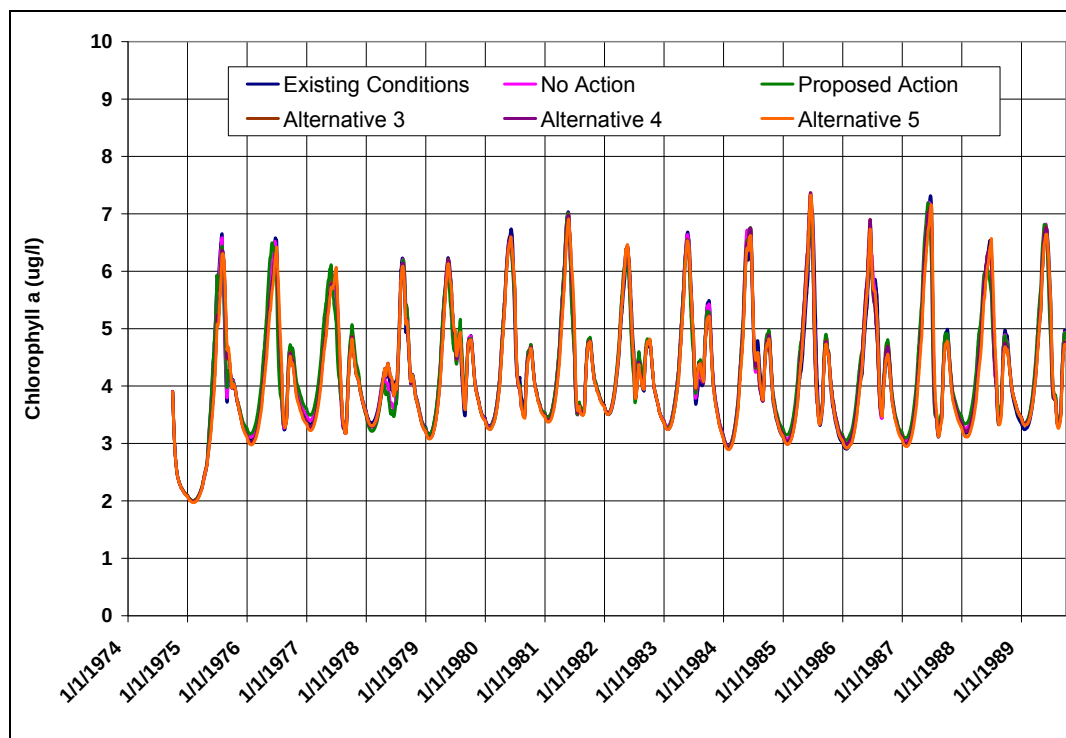
Figure 42: Simulated Daily Chlorophyll a Concentrations in Granby Reservoir (Existing Conditions and All Alternatives)
