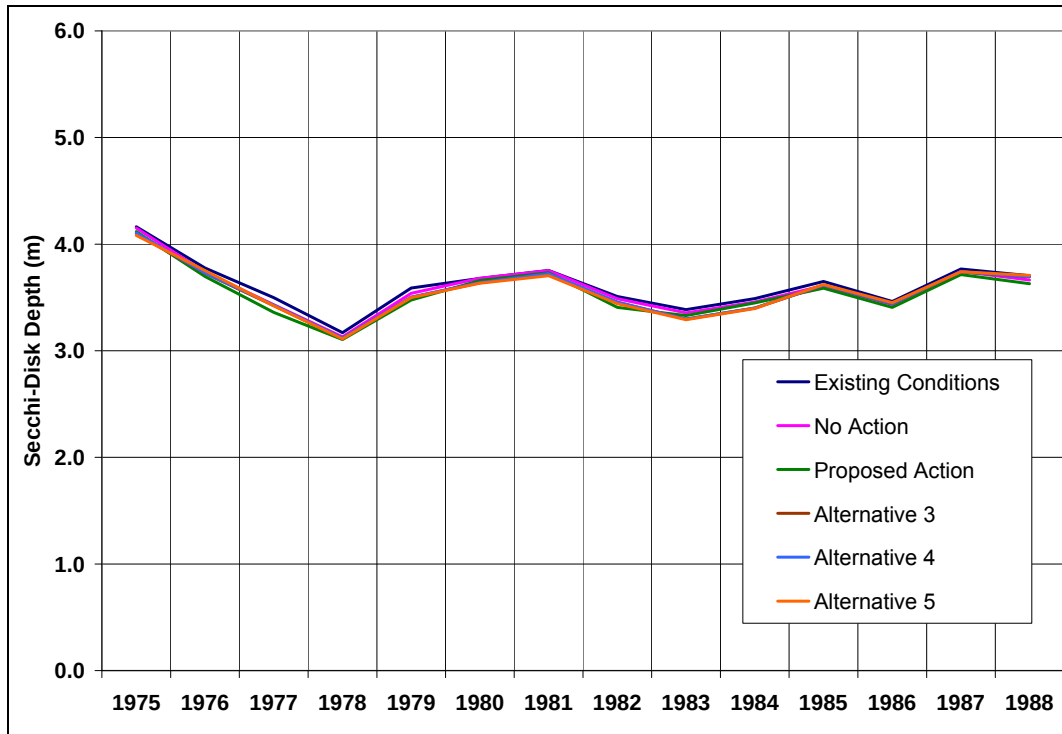
Figure 43: Predicted Annual Average Secchi-Disk Depth in Granby Reservoir (Existing Conditions and All Alternatives)
