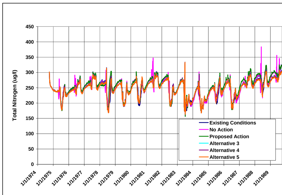
Figure 73: Predicted Daily Total Nitrogen Concentrations in Grand Lake Epilimnion (Existing Conditions and All Alternatives)
