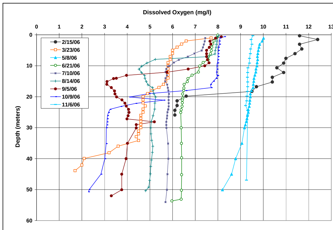
Figure 10: Dissolved Oxygen Profiles for Granby Reservoir in 2006 (Data Sources: USGS, 2007; NCWCD, 2007b)
