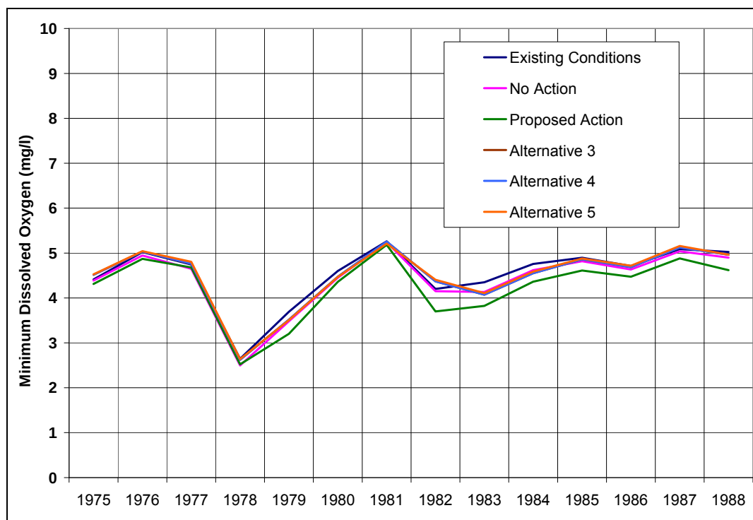
Figure 48: Predicted Minimum Dissolved Oxygen Concentration in Granby Reservoir Hypolimnion (Existing Conditions and All Alternatives)
