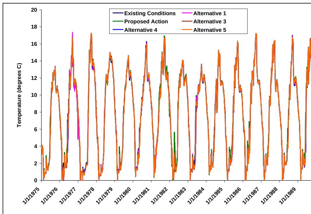
Figure 52: Simulated Epilimnetic Temperature in Granby Reservoir for Existing Conditions and the Alternatives
