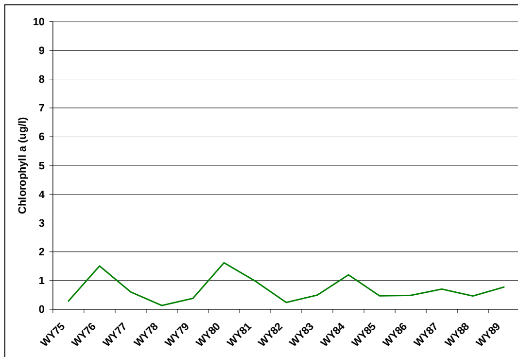
Figure 191: Predicted Chlorophyll a Concentrations in Chimney Hollow Reservoir (Cumulative Effects Proposed Action)
