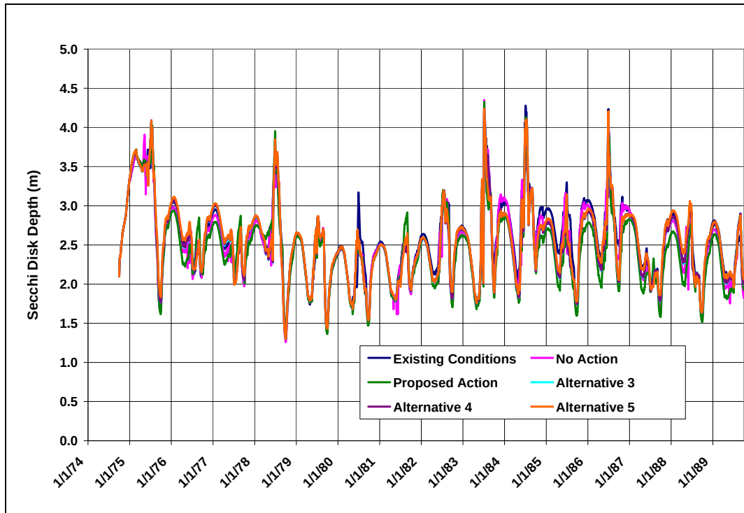
Figure 79: Predicted Daily Secchi-Disk Depths in Grand Lake (Existing Conditions and All Alternatives)
