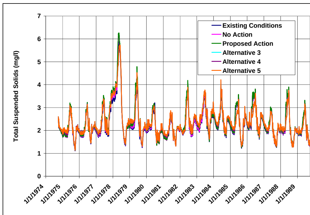
Figure 51: Predicted Daily Total Suspended Sediment Concentration in Granby Reservoir Epilimnion (Existing Conditions and All Alternatives)
