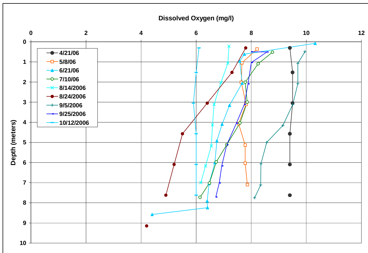
Figure 13: Dissolved Oxygen Profiles for Shadow Mountain Reservoir in 2006 (Data Sources: USGS, 2007; NCWCD, 2007b)
