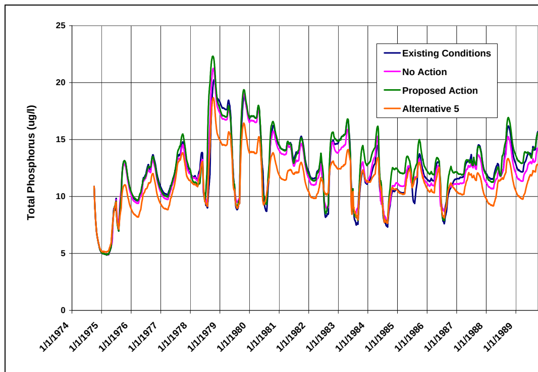
Figure 139: Predicted Daily Total Phosphorus Concentrations in Shadow Mountain Reservoir--Cumulative Effects
