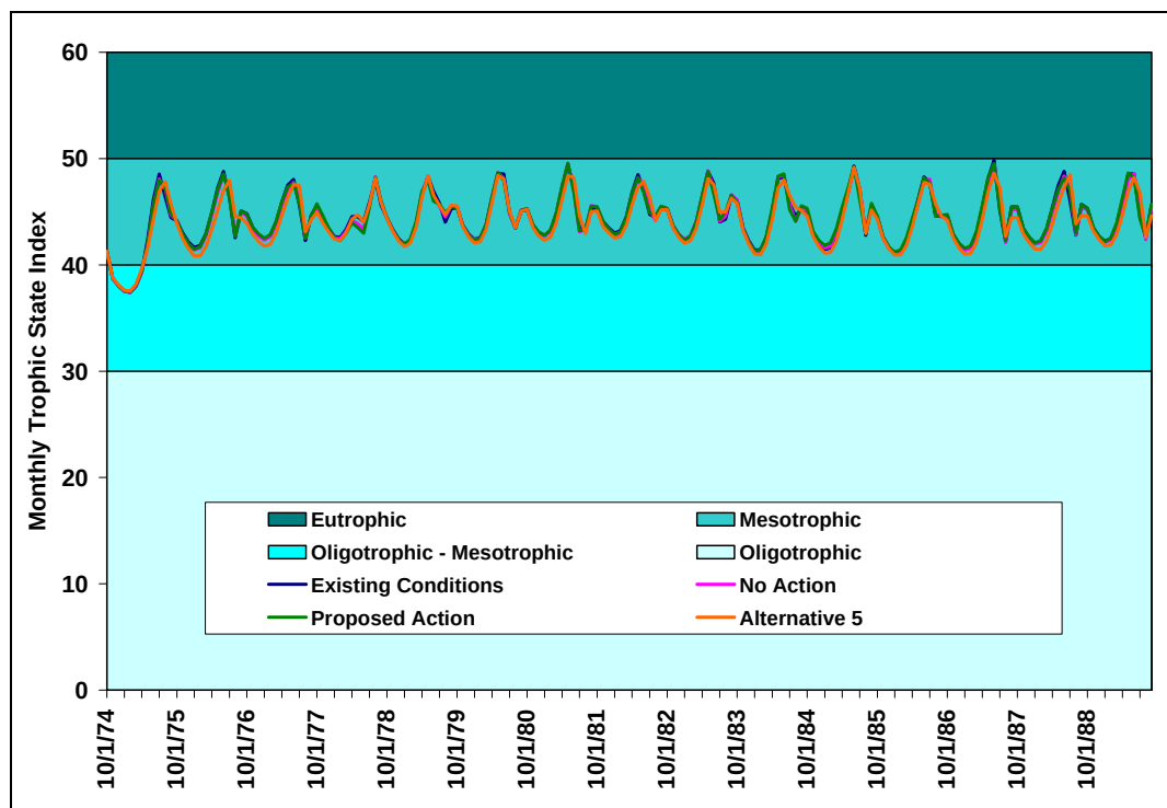
Figure 132: Predicted Monthly Trophic State Index for Granby Reservoir--Cumulative Effects
