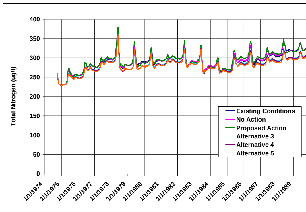
Figure 39: Predicted Daily Total Nitrogen Concentrations in Granby Reservoir Epilimnion (Existing Conditions and All Alternatives)
