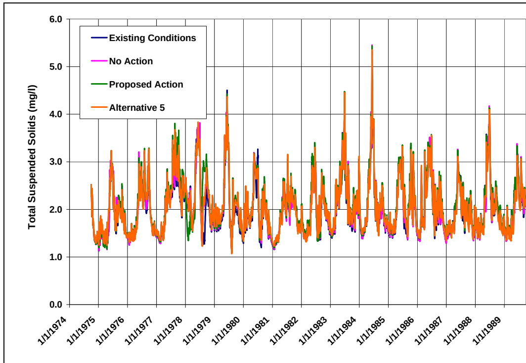
Figure 153: Predicted Daily Total Suspended Sediment Concentrations in Shadow Mountain Reservoir--Cumulative Effects
