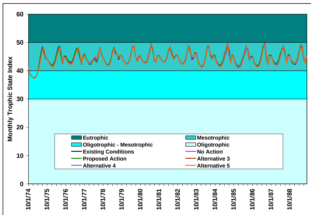
Figure 47: Predicted Monthly Trophic State Index for Granby Reservoir
