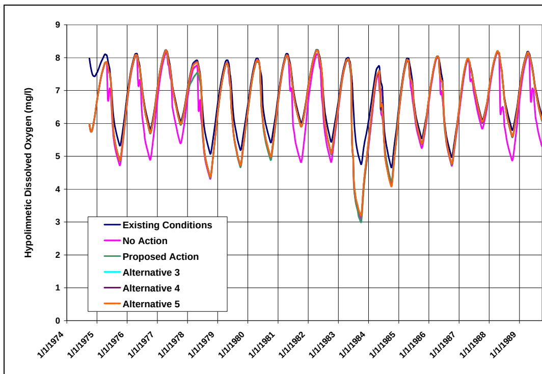
Figure 83: Predicted Daily Dissolved Oxygen Concentration in Grand Lake (Existing Conditions and All Alternatives)
