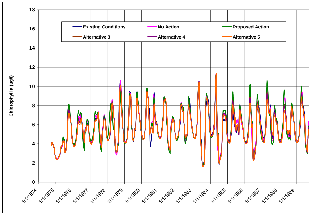
Figure 60: Simulated Daily Chlorophyll a Concentrations in Shadow Mountain Reservoir (Existing Conditions and All Alternatives)
