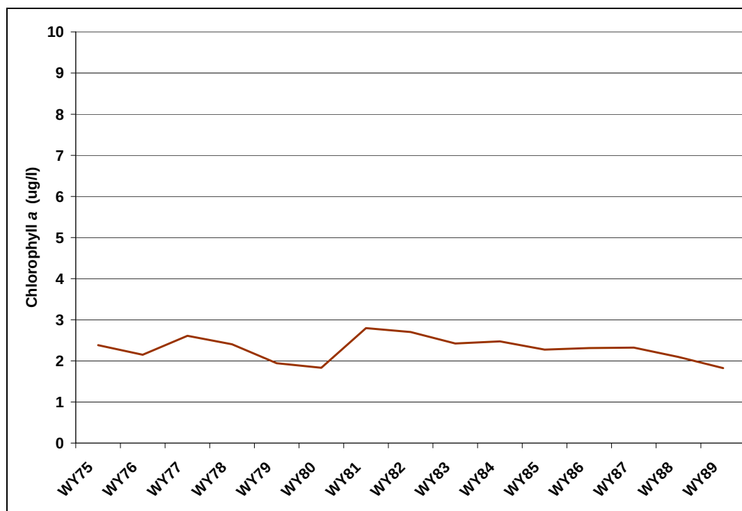
Figure 103: Predicted Annual Average Chlorophyll a Concentrations in Jasper East Reservoir (Alternative 3)
