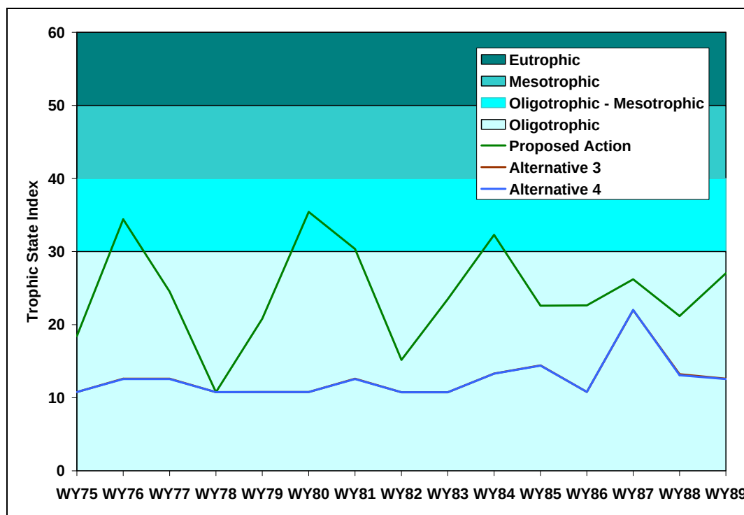
Figure 115: Predicted Trophic State Indices in Chimney Hollow Reservoir (Proposed Action and Alternatives 3 and 4)
