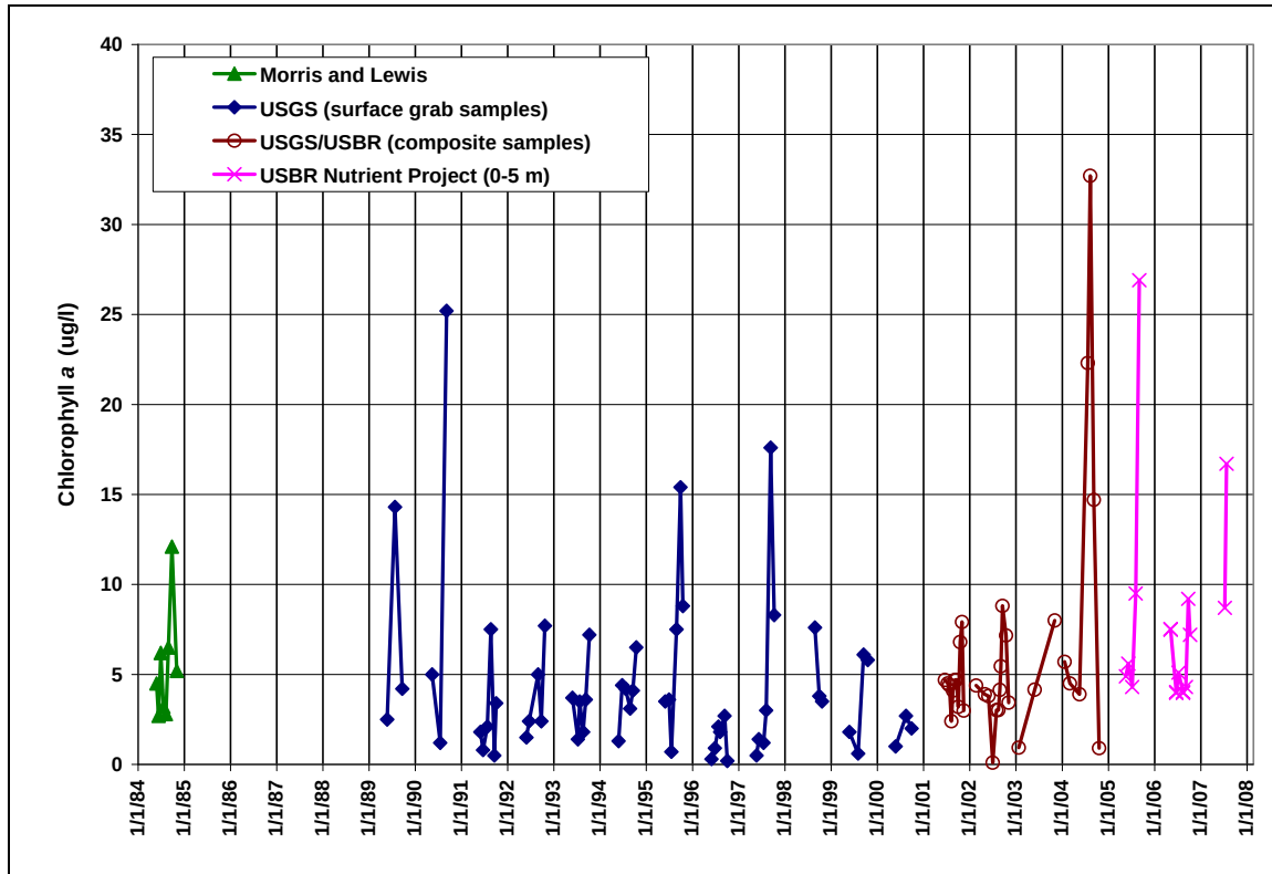
Figure 11: Chlorophyll a Concentrations in Shadow Mountain Reservoir (Data Sources: Morris & Lewis, 1988; USGS, 2007; USBR, 2005; NCWCD, 2007b)
