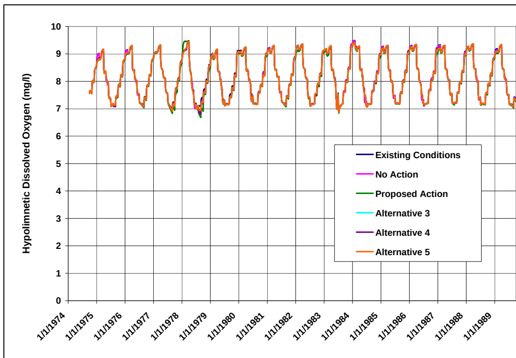
Figure 67: Predicted Daily Dissolved Oxygen in Shadow Mountain Reservoir (Existing Conditions and All Alternatives)
