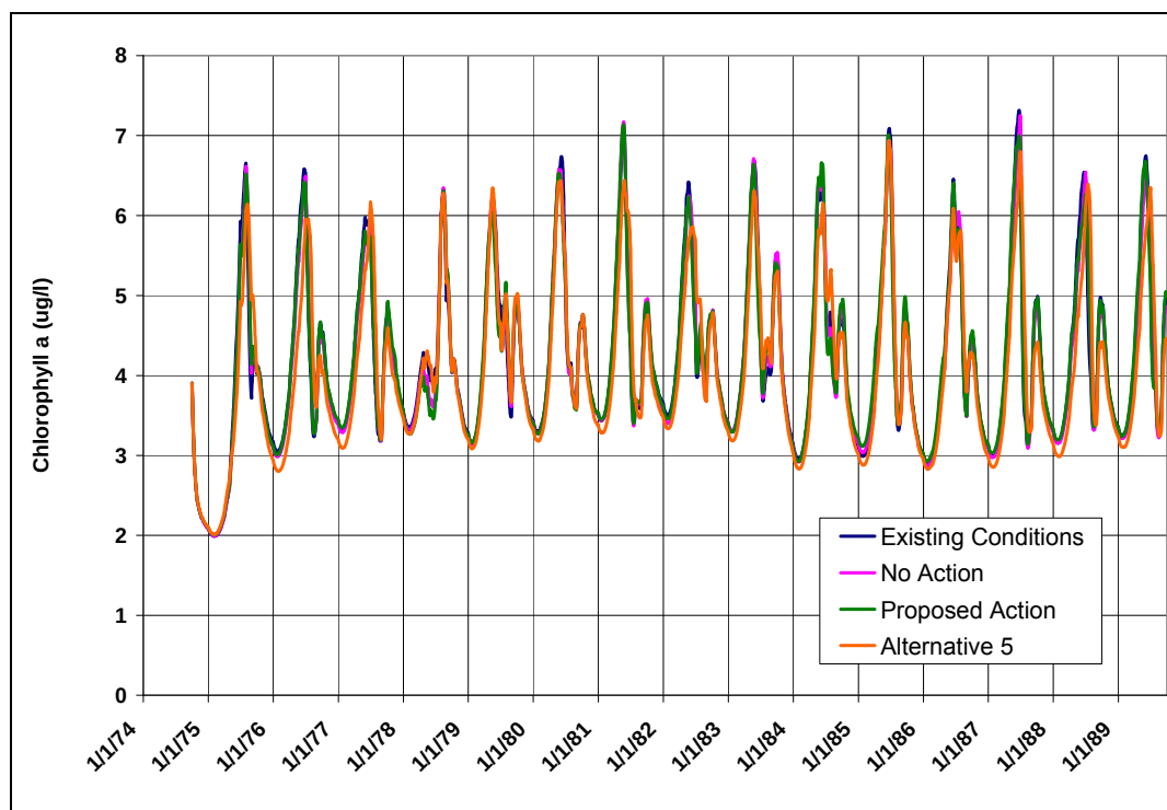
Figure 127: Predicted Daily Chlorophyll a Concentrations in Granby Reservoir--Cumulative Effects
