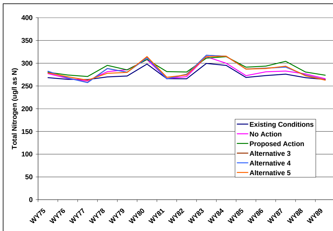
Figure 92: Predicted Annual Average Total Nitrogen Concentrations in Horsetooth Reservoir (Existing Conditions and All Alternatives)
