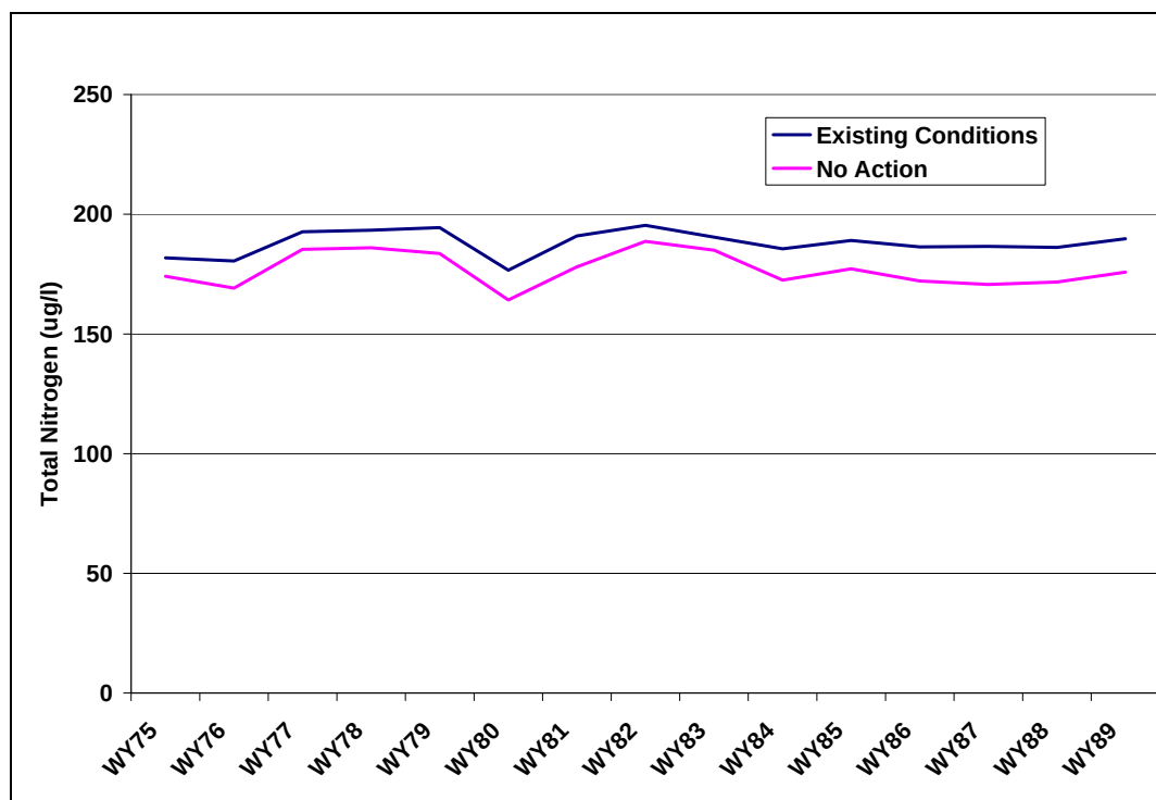
Figure 180: Predicted Total Nitrogen Concentrations in Ralph Price Reservoir--Cumulative Effects
