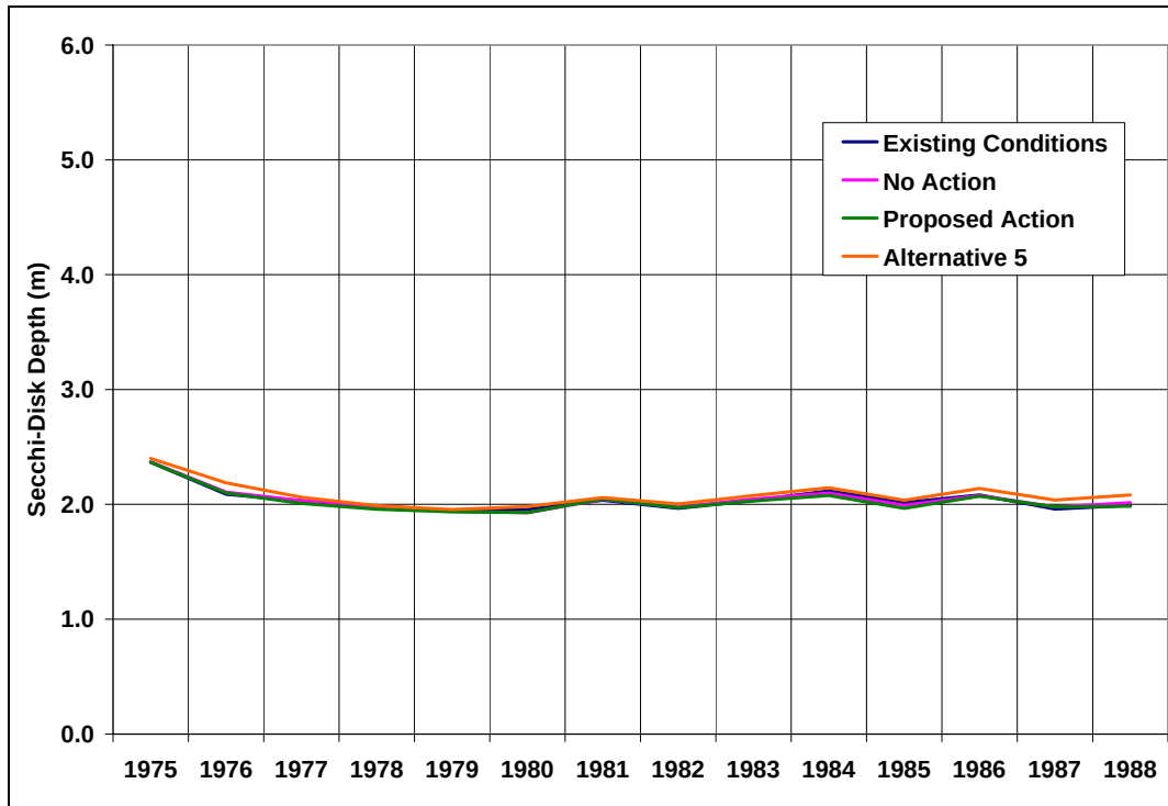
Figure 145: Predicted Average Annual Secchi-Disk Depth in Shadow Mountain Reservoir--Cumulative Effects
