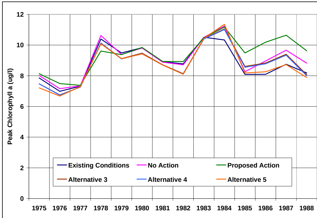
Figure 59: Simulated Peak Chlorophyll a Concentrations in Shadow Mountain Reservoir by Year for Existing Conditions and All Alternatives
