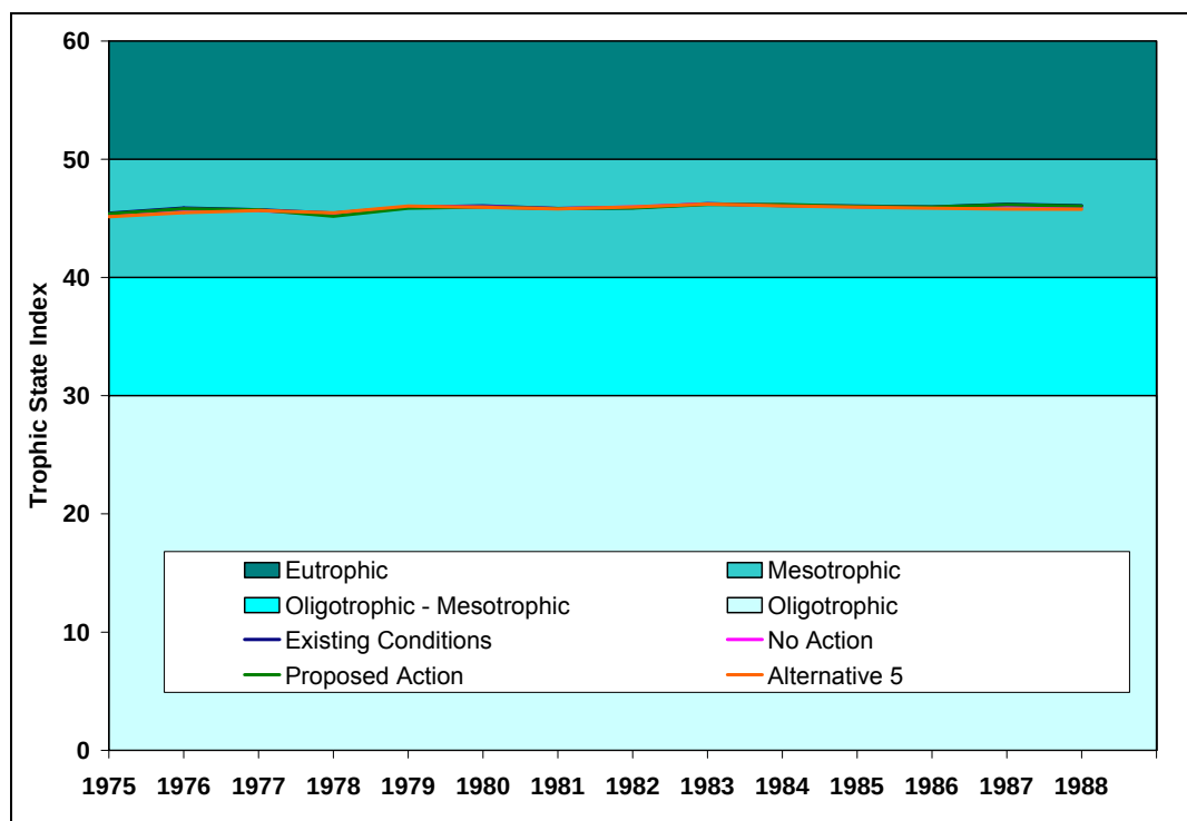
Figure 131: Predicted Annual Trophic State Indices in Granby Reservoir--Cumulative Effects
