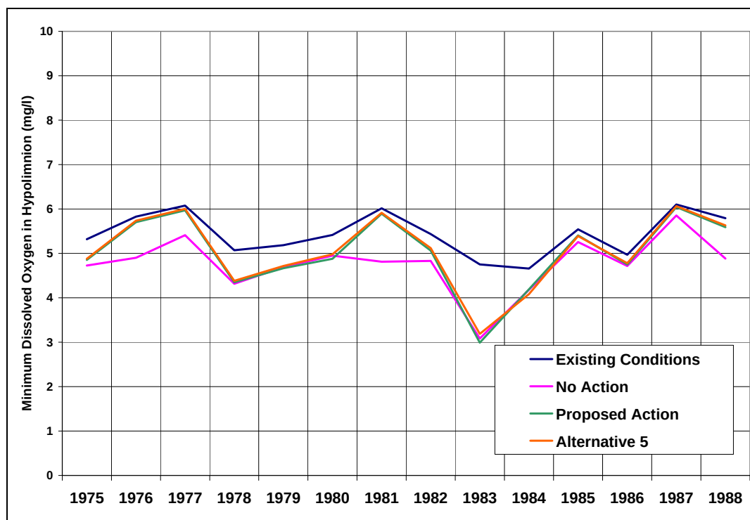
Figure 166: Predicted Minimum Dissolved Oxygen Concentrations in Grand Lake--Cumulative Effects
