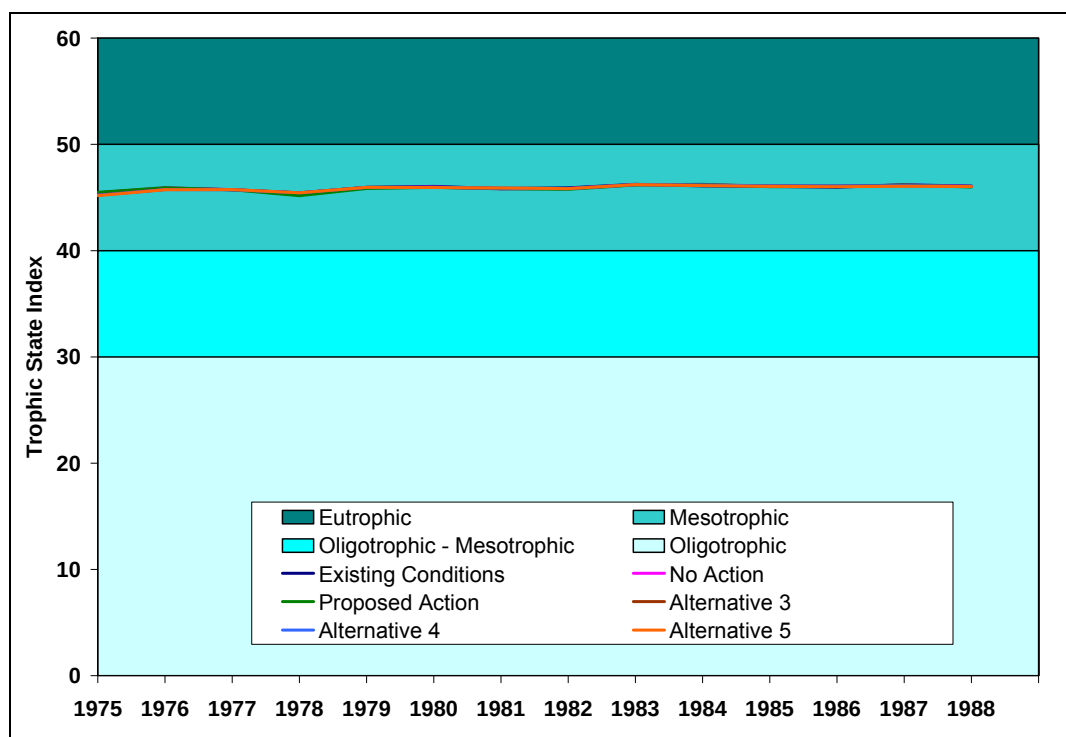
Figure 46: Predicted Trophic State Indices in Granby Reservoir (Existing Conditions and All Alternatives)
