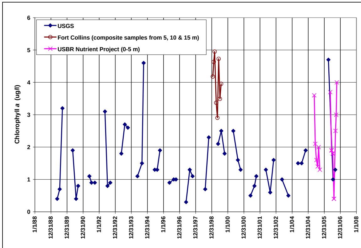
Figure 20: Carter Lake Chlorophyll a Concentrations (Data Sources: USGS, 2007; NCWCD, 2007b; Ft. Collins, 2007)
