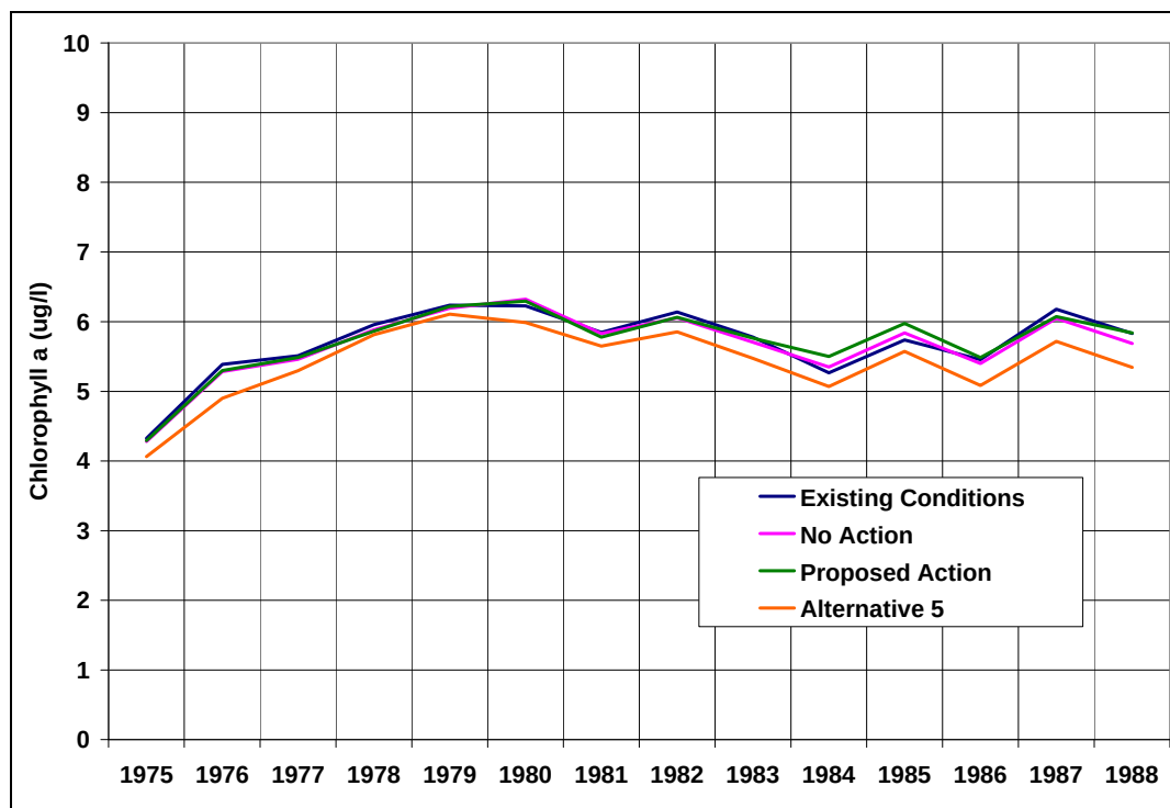
Figure 142: Predicted Average Annual Chlorophyll a Concentrations in Shadow Mountain Reservoir--Cumulative Effects
