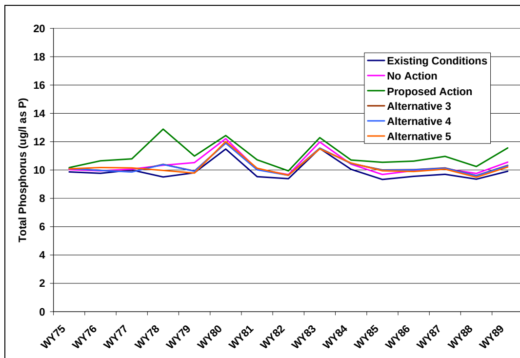
Figure 91: Predicted Annual Average Total Phosphorus Concentrations in Horsetooth Reservoir (Existing Conditions and All Alternatives)
