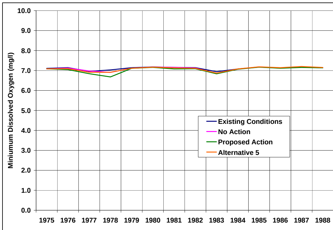
Figure 150: Predicted Minimum Dissolved Oxygen in Shadow Mountain Reservoir--Cumulative Effects
