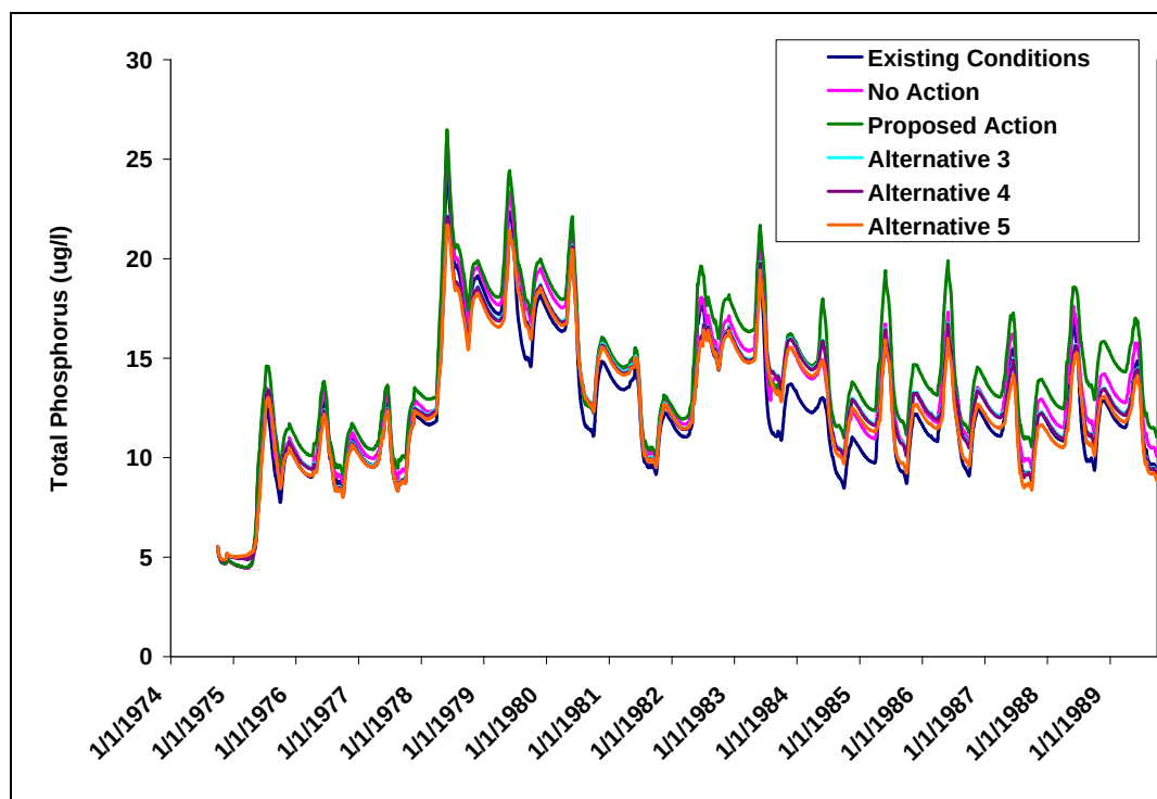
Figure 37: Predicted Daily Total Phosphorus Concentrations in Granby Reservoir Epilimnion (Existing Conditions and All Alternatives)
