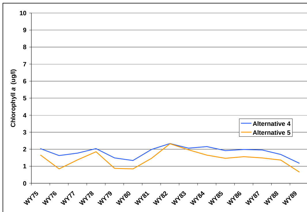
Figure 108: Predicted Annual Average Chlorophyll a Concentrations in Rockwell Creek Reservoir (Alternatives 4 and 5)
