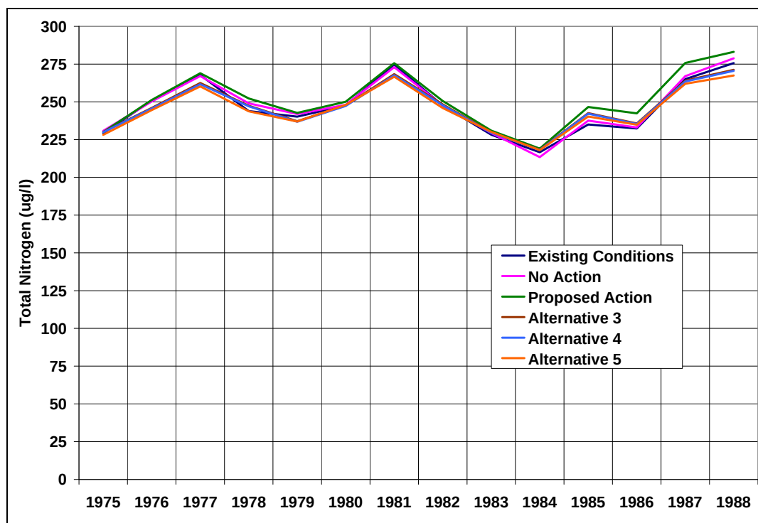
Figure 72: Predicted Annual Average Total Nitrogen Concentrations in Grand Lake Epilimnion (Existing Conditions and All Alternatives)
