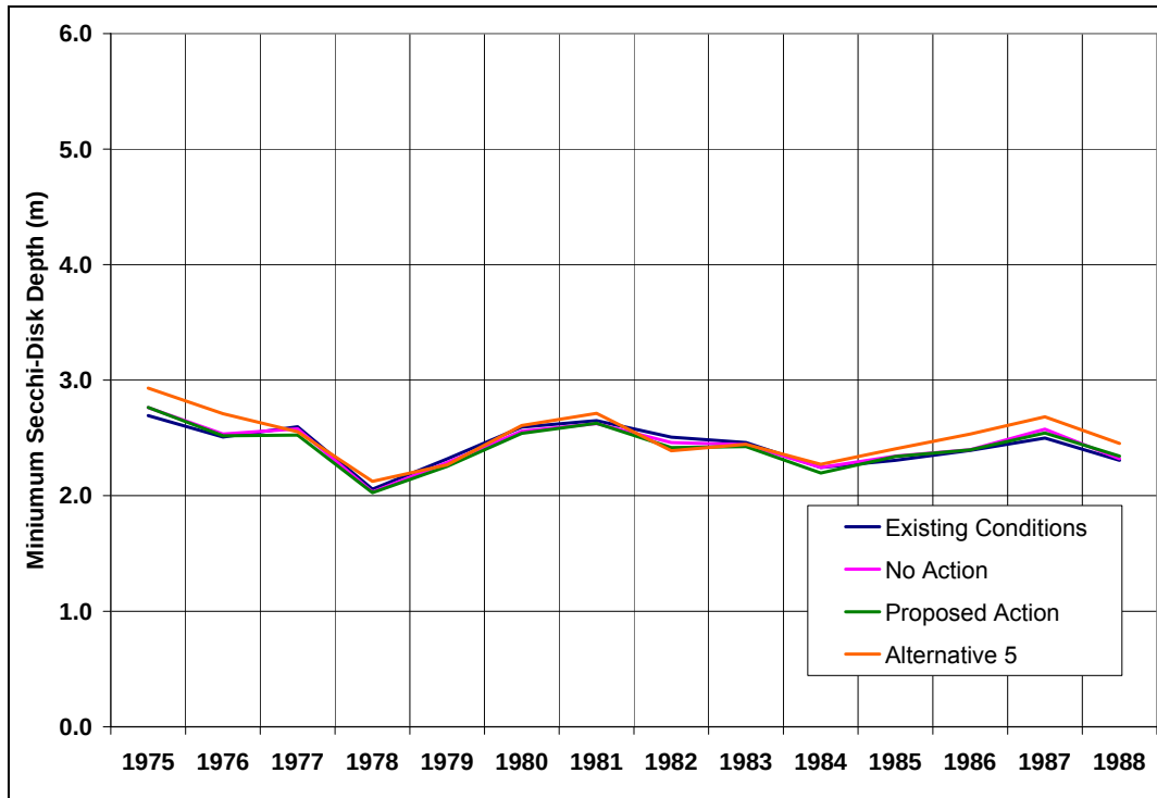
Figure 129: Predicted Minimum Secchi-Disk Depths in Granby Reservoir--Cumulative Effects
