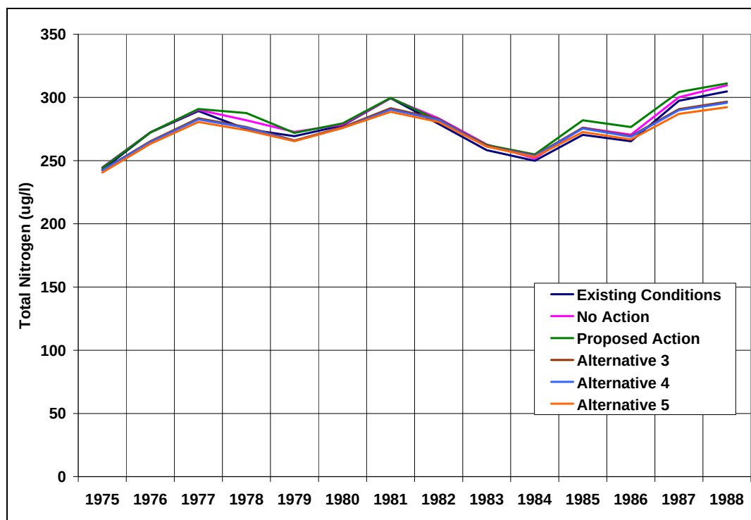
Figure 56: Predicted Annual Average Total Nitrogen Concentrations in Shadow Mountain Reservoir (Existing Conditions and All Alternatives)
