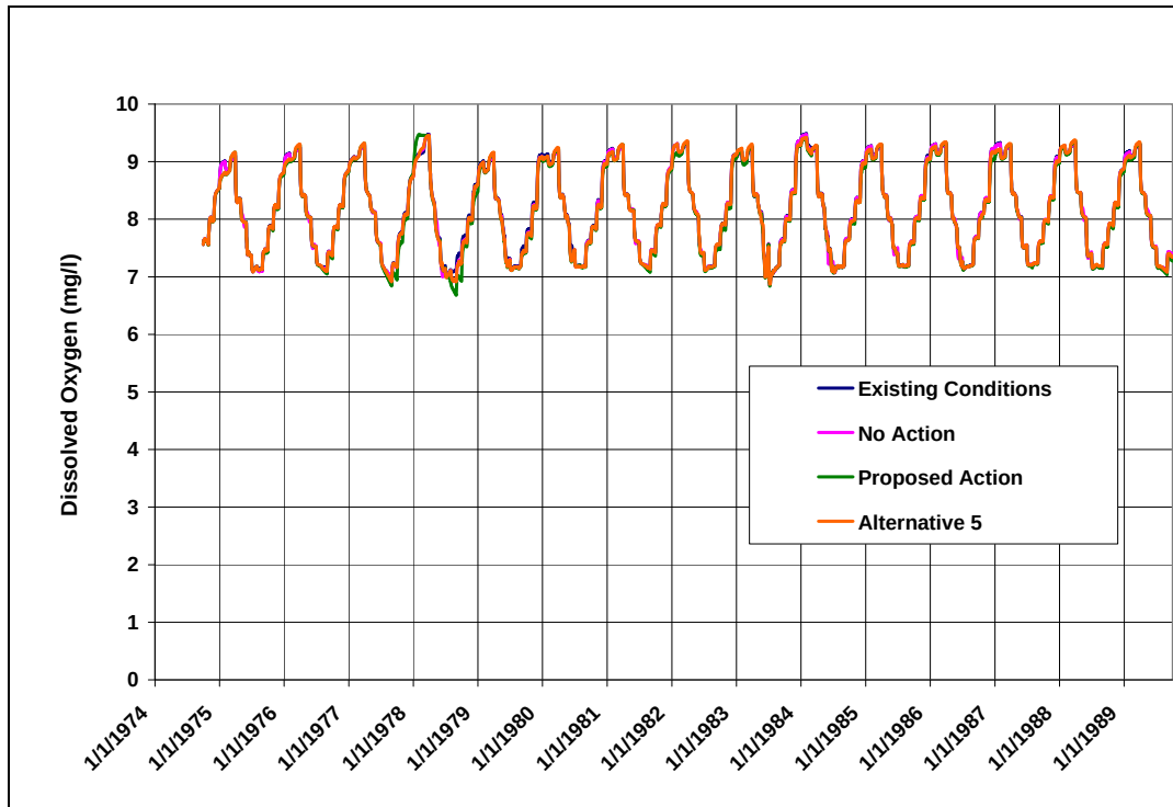
Figure 151: Predicted Daily Dissolved Oxygen in Shadow Mountain Reservoir--Cumulative Effects
