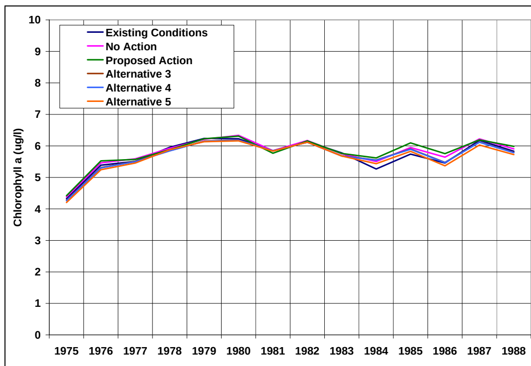
Figure 58: Predicted Annual Average Chlorophyll a Concentrations in Shadow Mountain Reservoir (Existing Conditions and All Alternatives)
