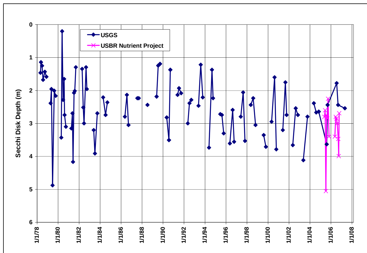
Figure 21: Carter Lake Secchi-Disk Depth (Data Sources: USGS, 2007; NCWCD, 2007b)
