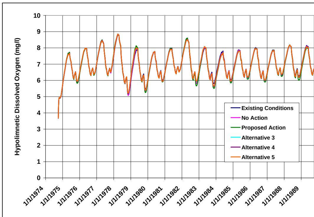
Figure 49: Predicted Daily Dissolved Oxygen Concentration in Granby Reservoir Hypolimnion (Existing Conditions and All Alternatives)
