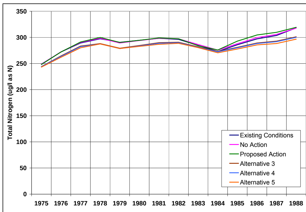
Figure 38: Predicted Annual Average Total Nitrogen Concentrations in Granby Reservoir Epilimnion (Existing Conditions and All Alternatives)
