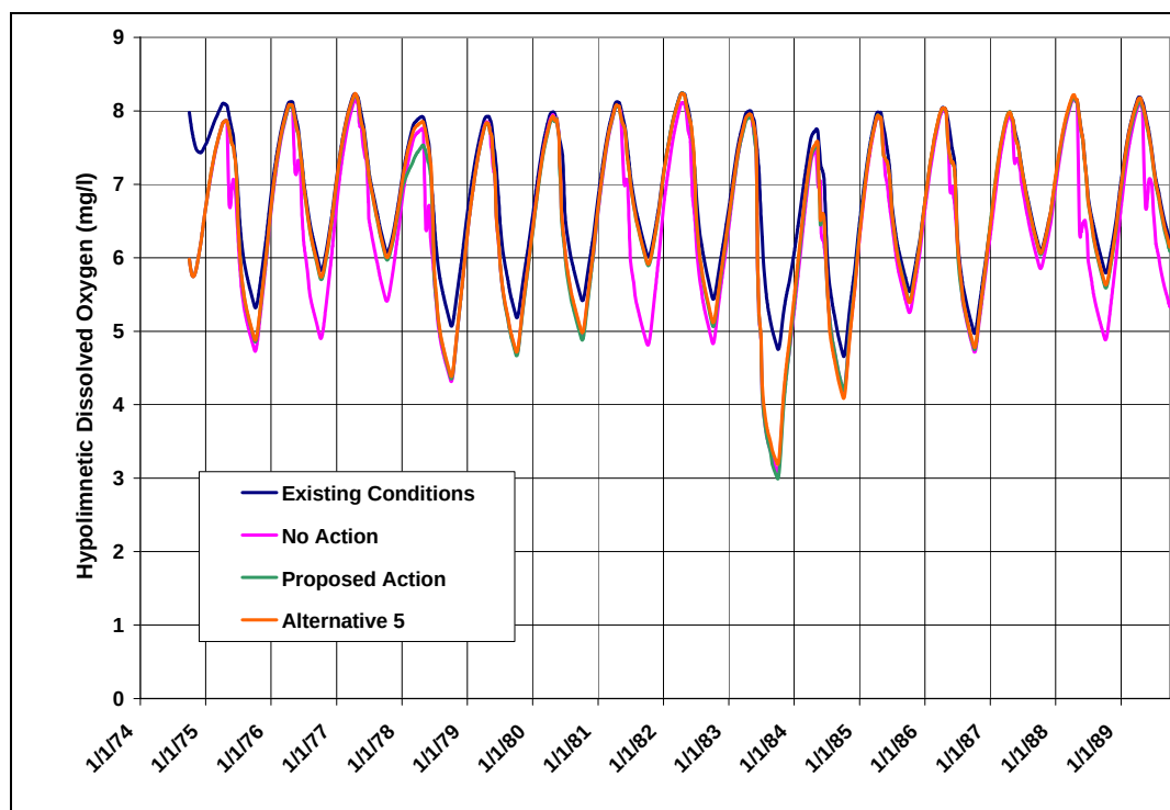
Figure 167: Predicted Daily Dissolved Oxygen Concentrations in Grand Lake--Cumulative Effects
