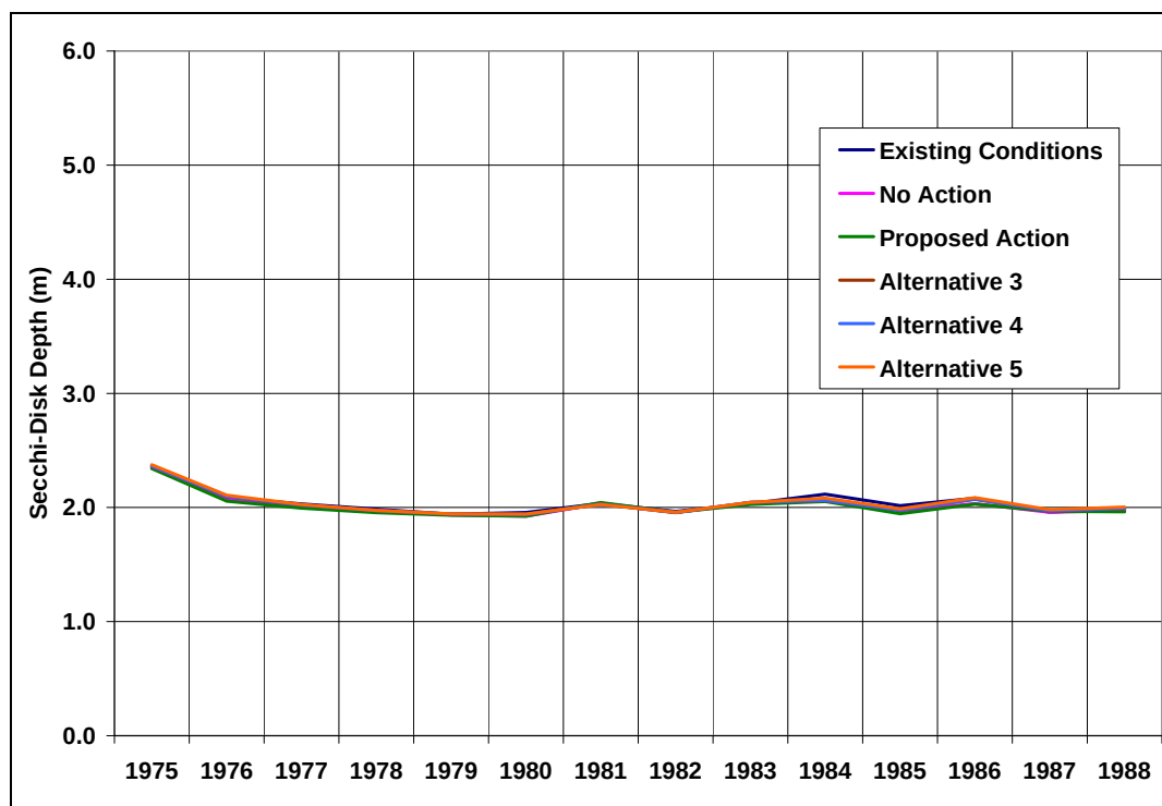
Figure 61: Predicted Annual Average Secchi-Disk Depths in Shadow Mountain Reservoir (Existing Conditions and All Alternatives)
