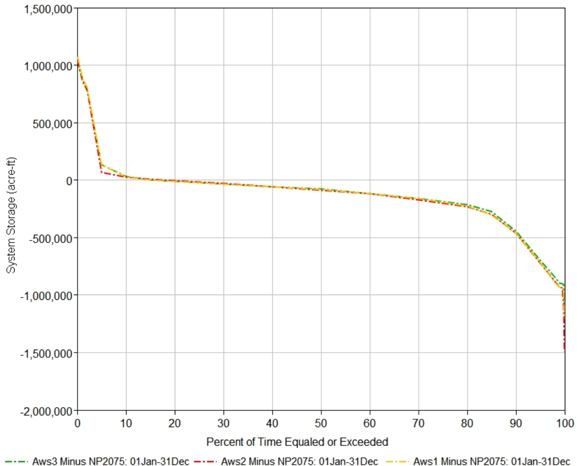
Figure 4-1: Duration curves of the change in System relative to NP2075 for each scenario.
