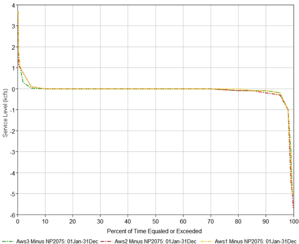
Figure 4-4: Duration curves of the change in service level relative to NP2075 for each scenario.
