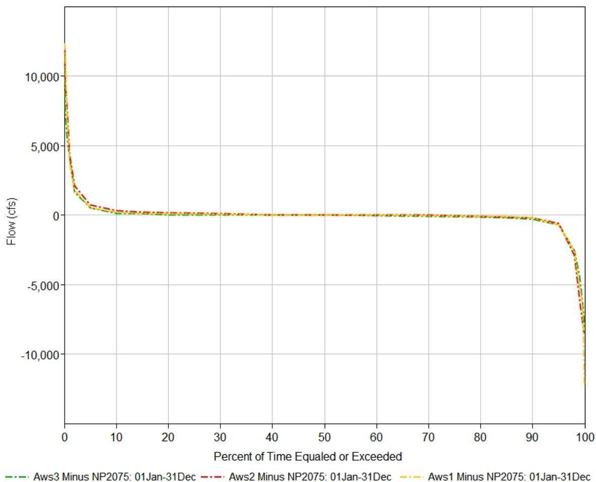
Figure 4-17: Duration curves of the change in Bismarck ND flows relative to NP2075 for each scenario.
