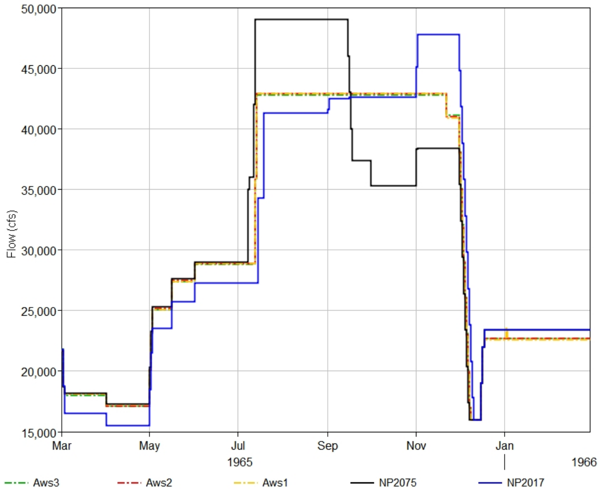
Figure 4-13: Garrison releases during 1965, a flood evacuation year.
