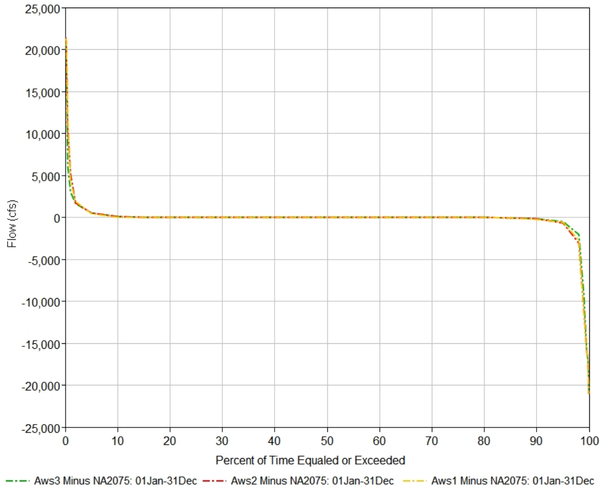
Figure 4-20: Duration curves of the change in Nebraska City, NE flows relative to NP2075 for each scenario.
