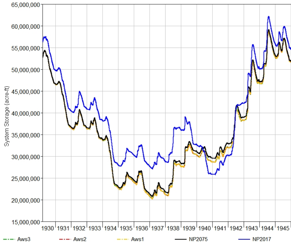
Figure 4-2: System storage during the 1930's drought.
