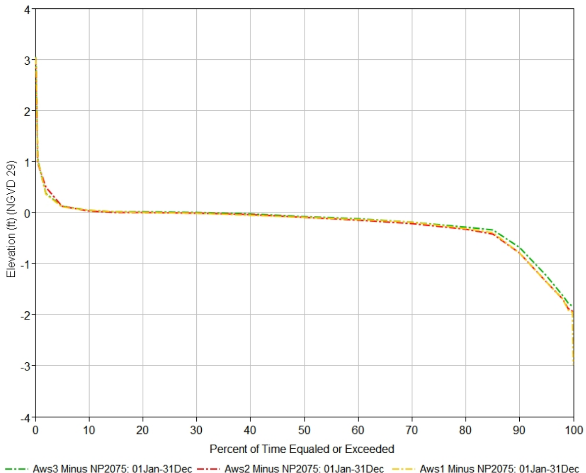
Figure 4-6: Duration curves of the change in Fort Peck pool elevation relative to NP2075 for each scenario.
