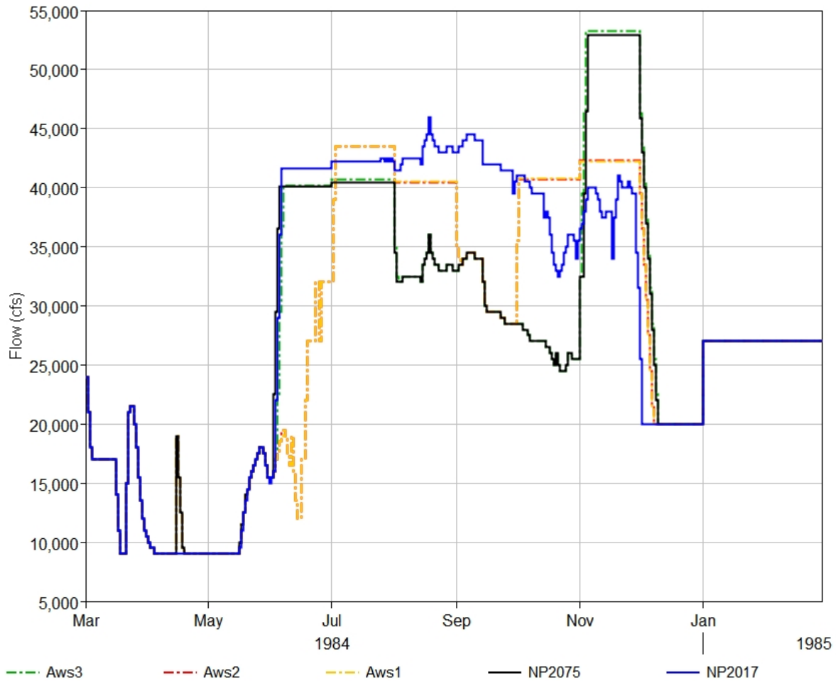
Figure 4-16: Gavins Point releases during 1984, a flood evacuation year.
