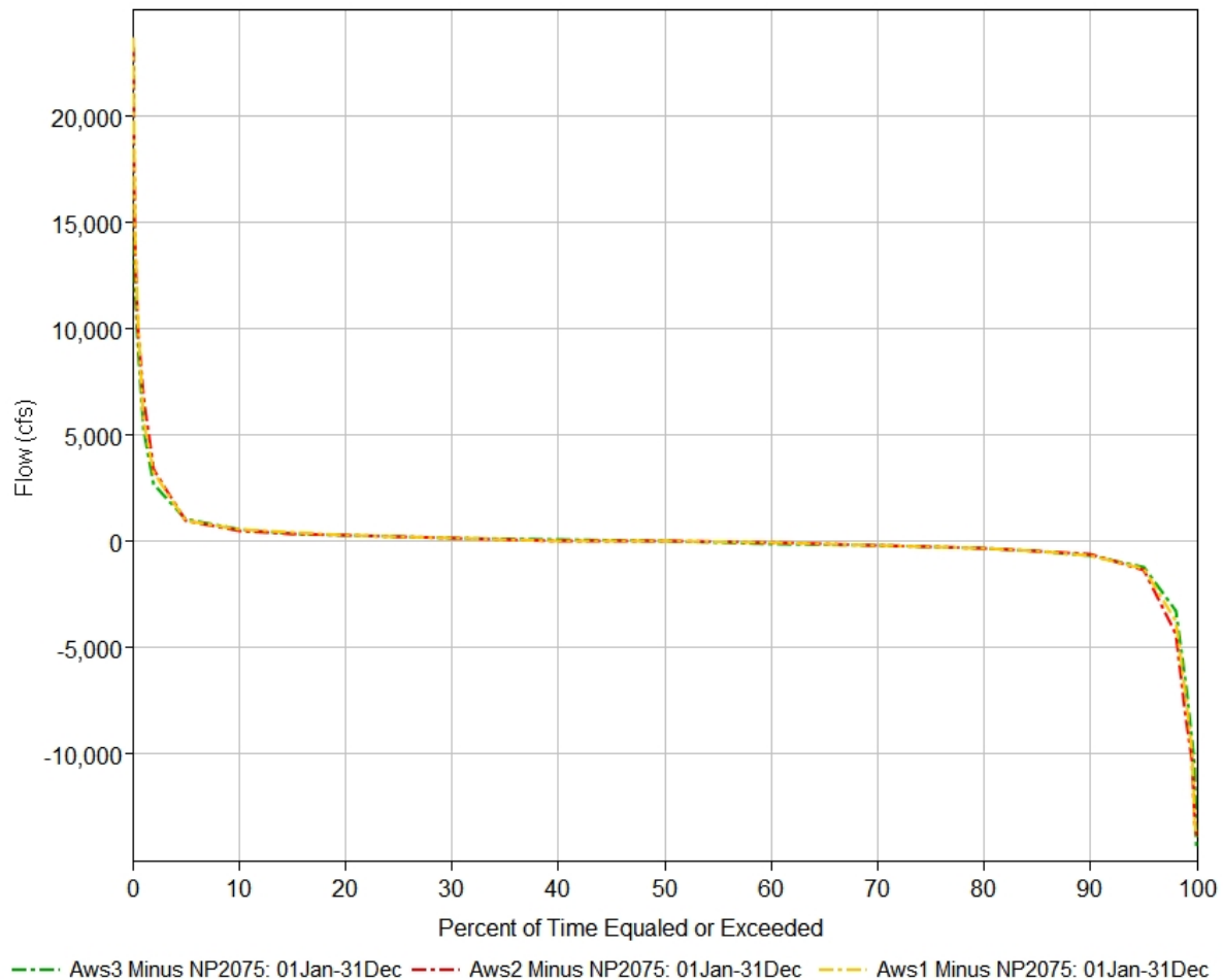
Figure 4-14: Duration curves of the change in Oahe releases relative to NP2075 for each scenario.
