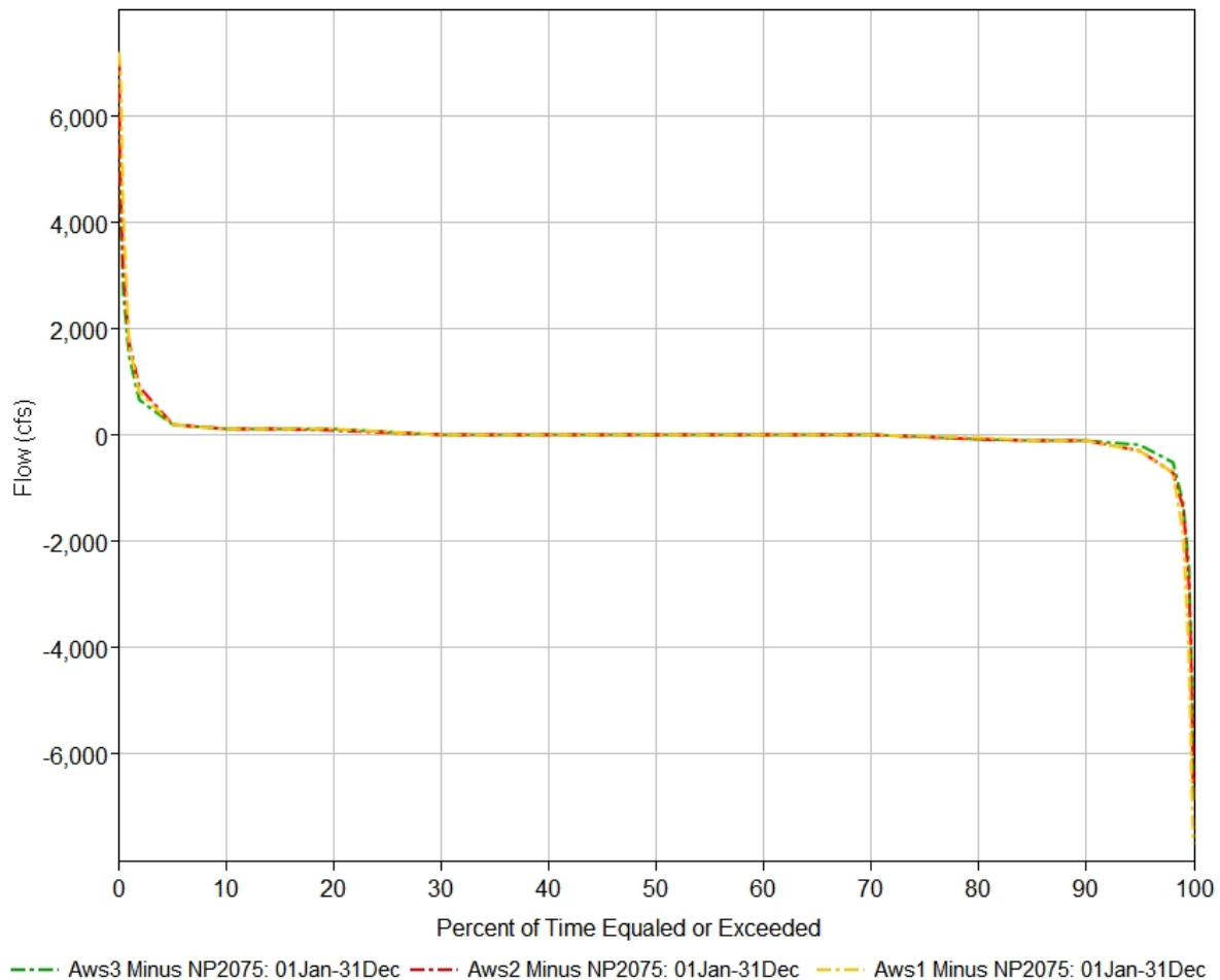
Figure 4-10: Duration curves of the change in Fort Peck releases relative to NP2075 for each scenario.
