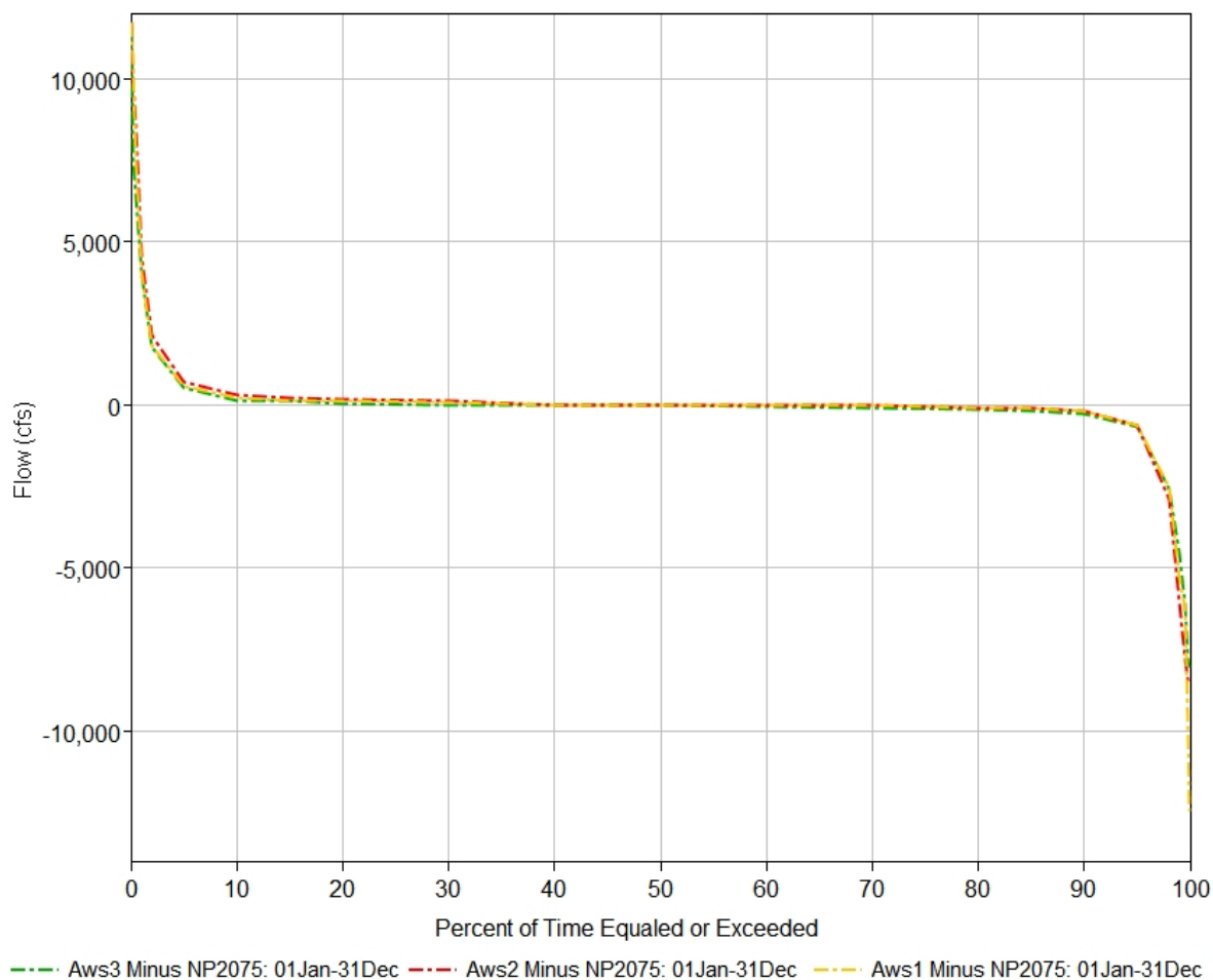
Figure 4-12: Duration curves of the change in Garrison releases relative to NP2075 for each scenario.
