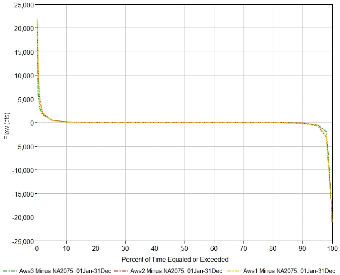
Figure 4-19: Duration curves of the change in Omaha, NE flows relative to NP2075 for each scenario.
