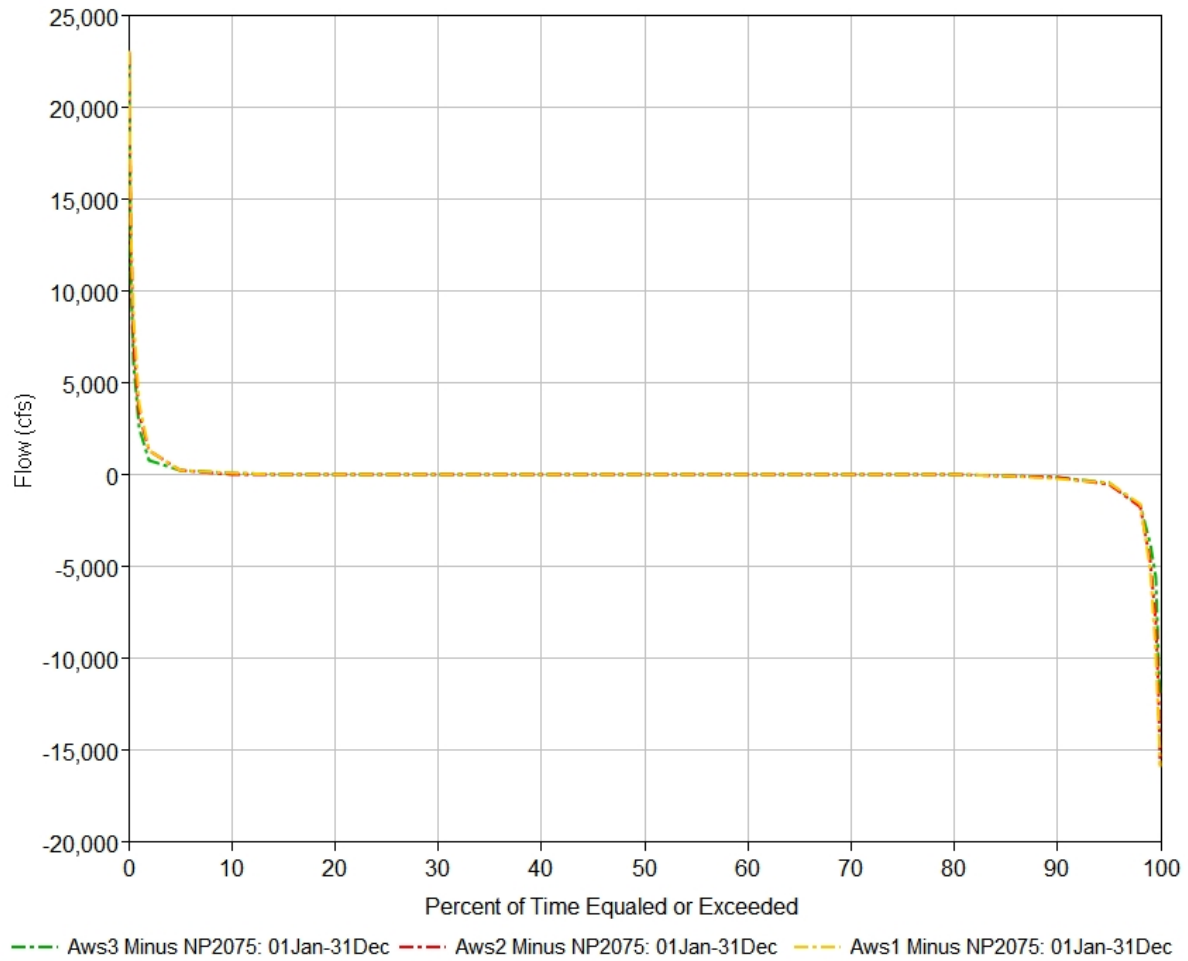
Figure 4-15: Duration curves of the change in Gavins Point releases relative to NP2075 for each scenario.
