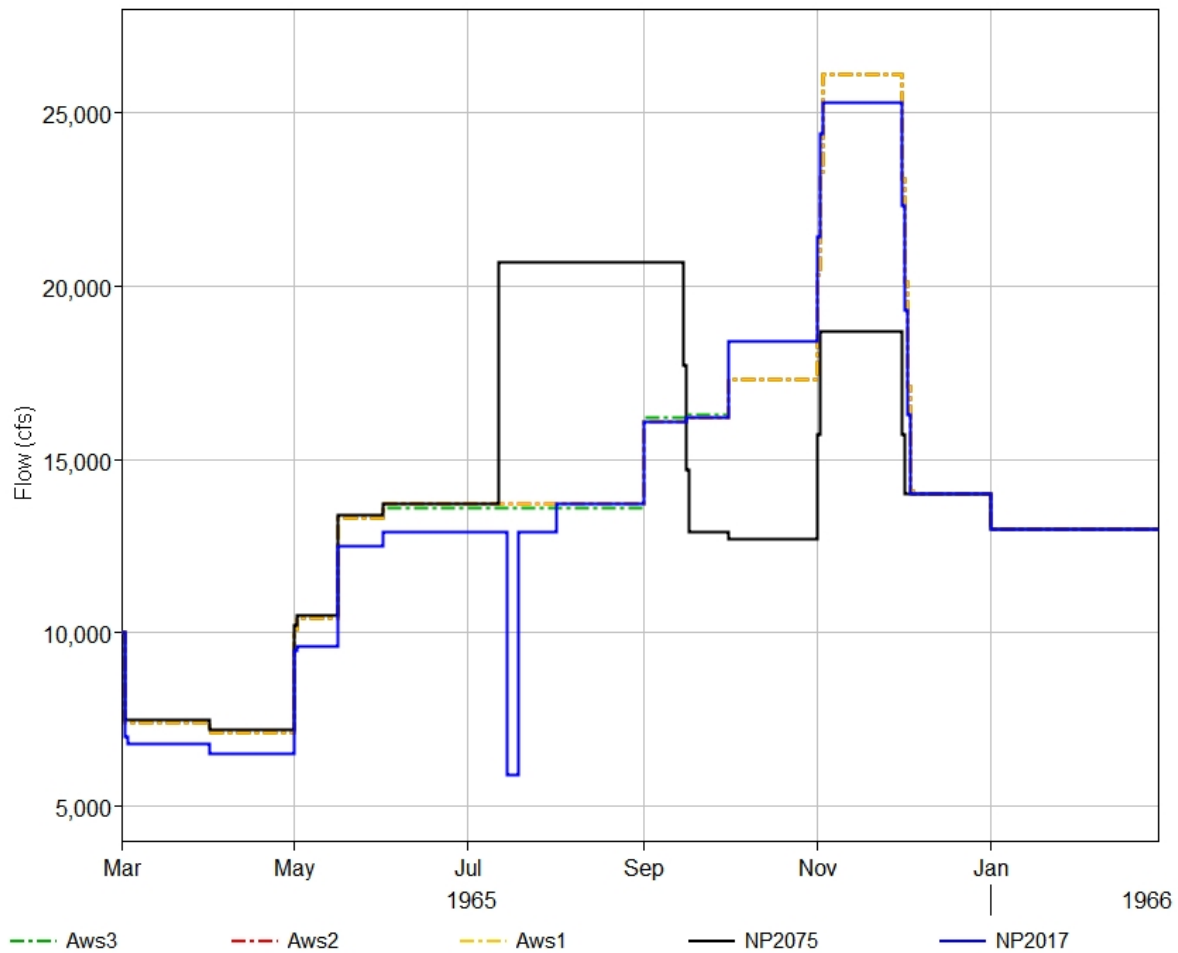
Figure 4-11: Fort Peck releases during 1965, a flood evacuation year.
