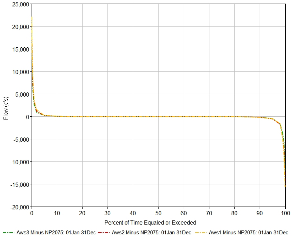
Figure 4-18: Duration curves of the change in Sioux City, IA flows relative to NP2075 for each scenario.
