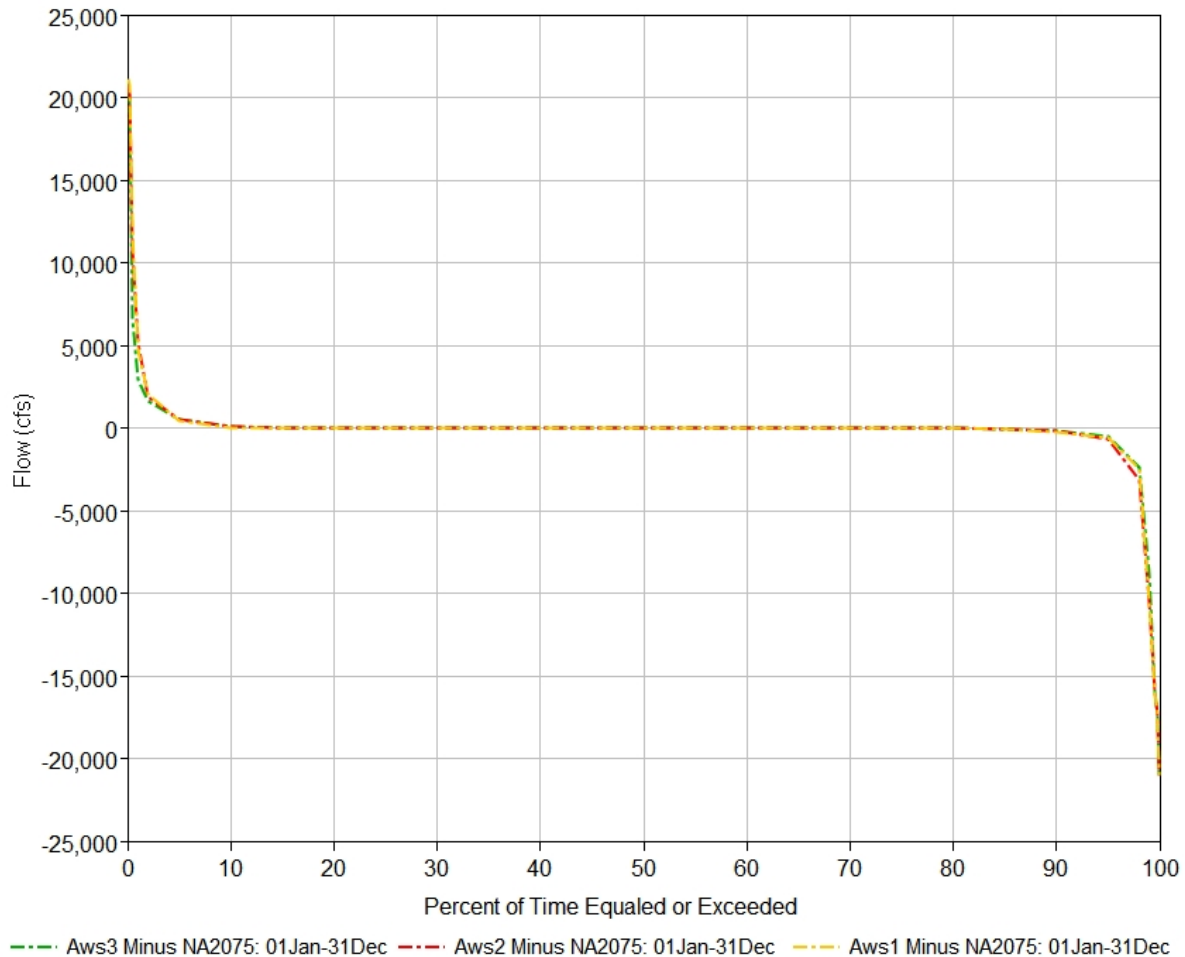
Figure 4-21: Duration curves of the change in Kansas City, MO flows relative to NP2075 for each scenario.
