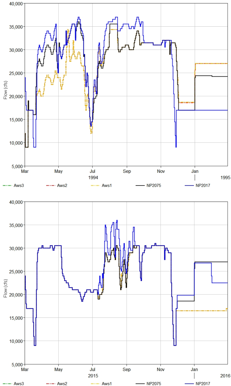
Figure 4-3: The top plot shows Gavins Point releases during 1994, a flood evacuation year. The bottom plot shows Gavins Point releases during 2015, a winter evacuation year.
