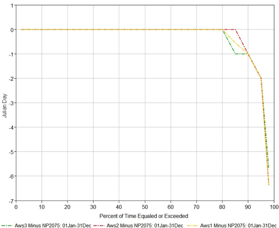
Figure 4-5: Duration curves of the change in navigation end date relative to NP2075 for each scenario.
