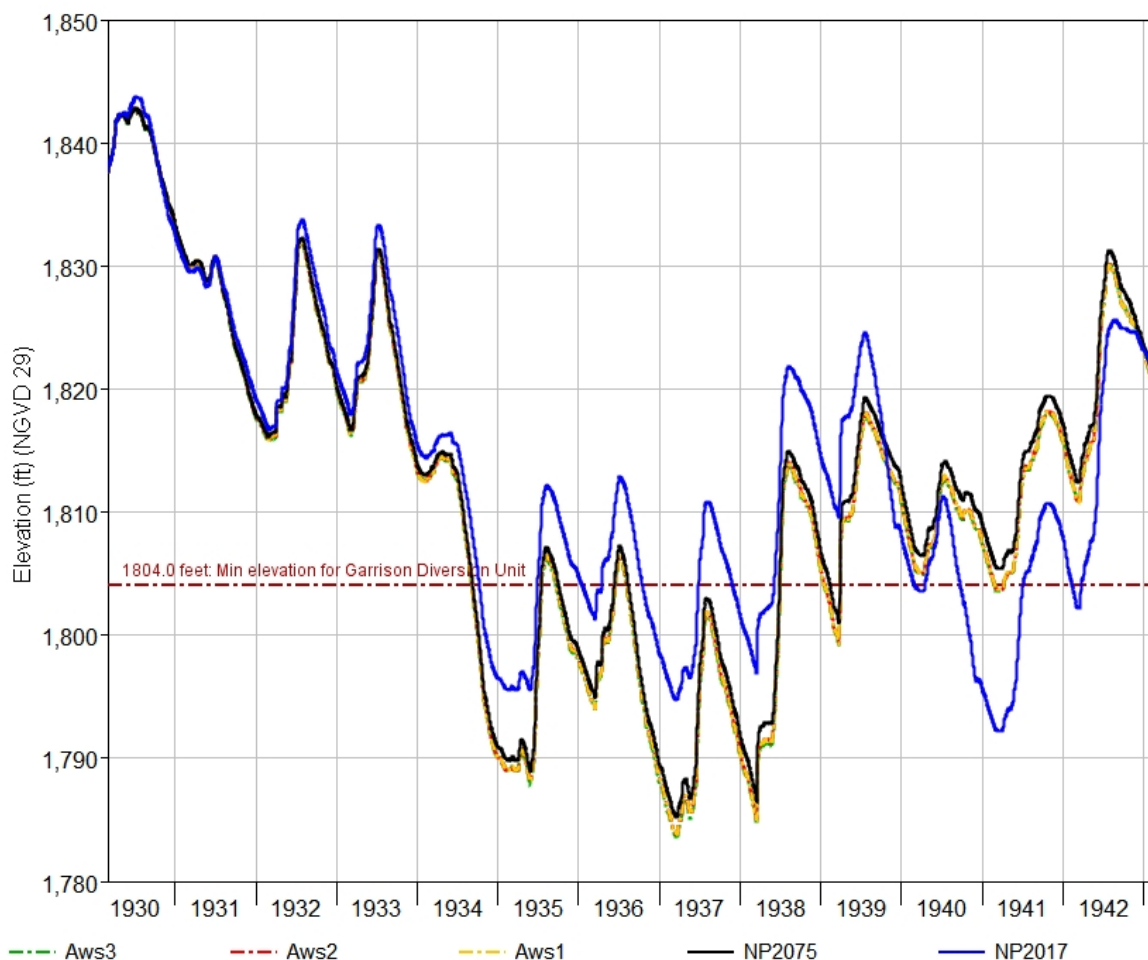
Figure 4-8: Garrison pool elevation compared to the minimum operation elevation for the Garrison Diversion Unit.
