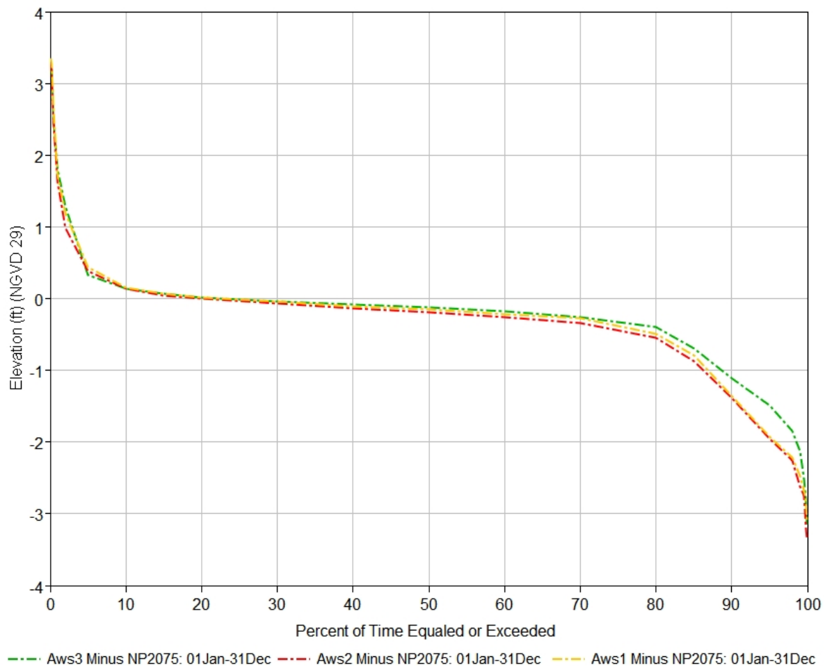
Figure 4-9: Duration curves of the change in Oahe pool elevation relative to NP2075 for each scenario.
