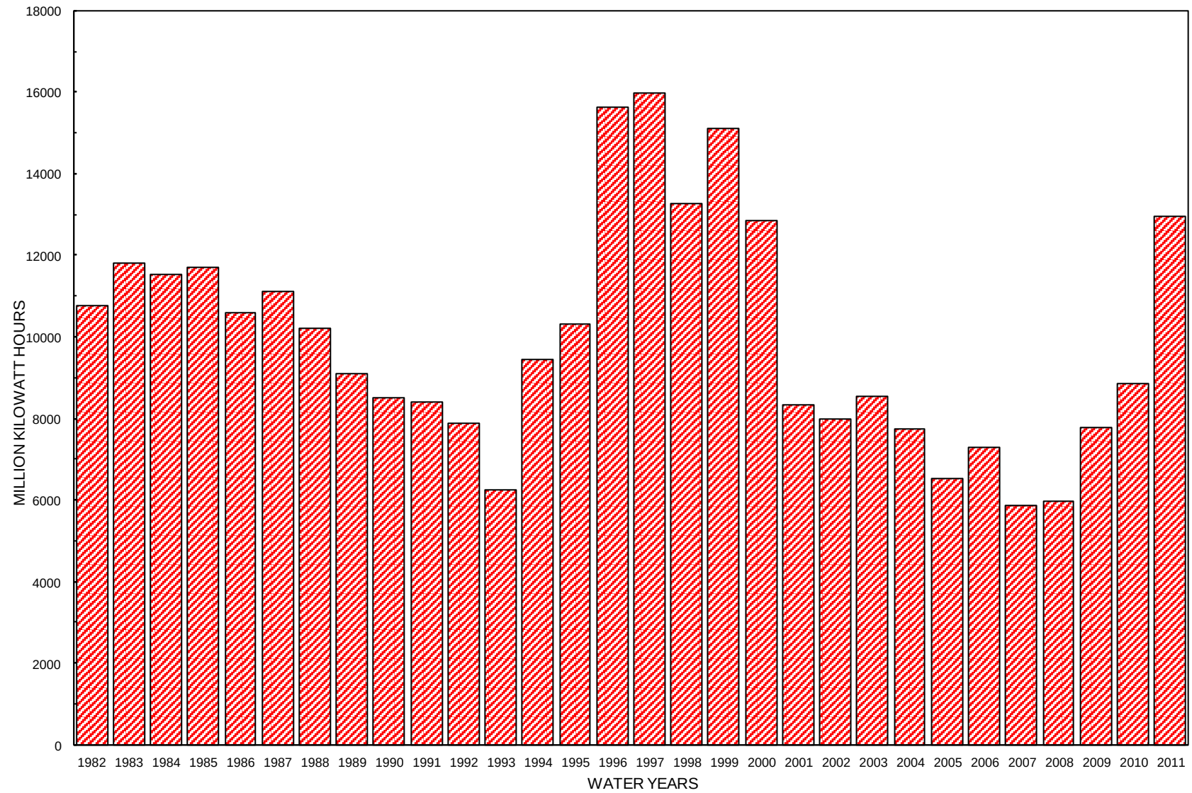
FIGURE CEG5 ANNUAL GENERATION - USBR & COE PLANTS
