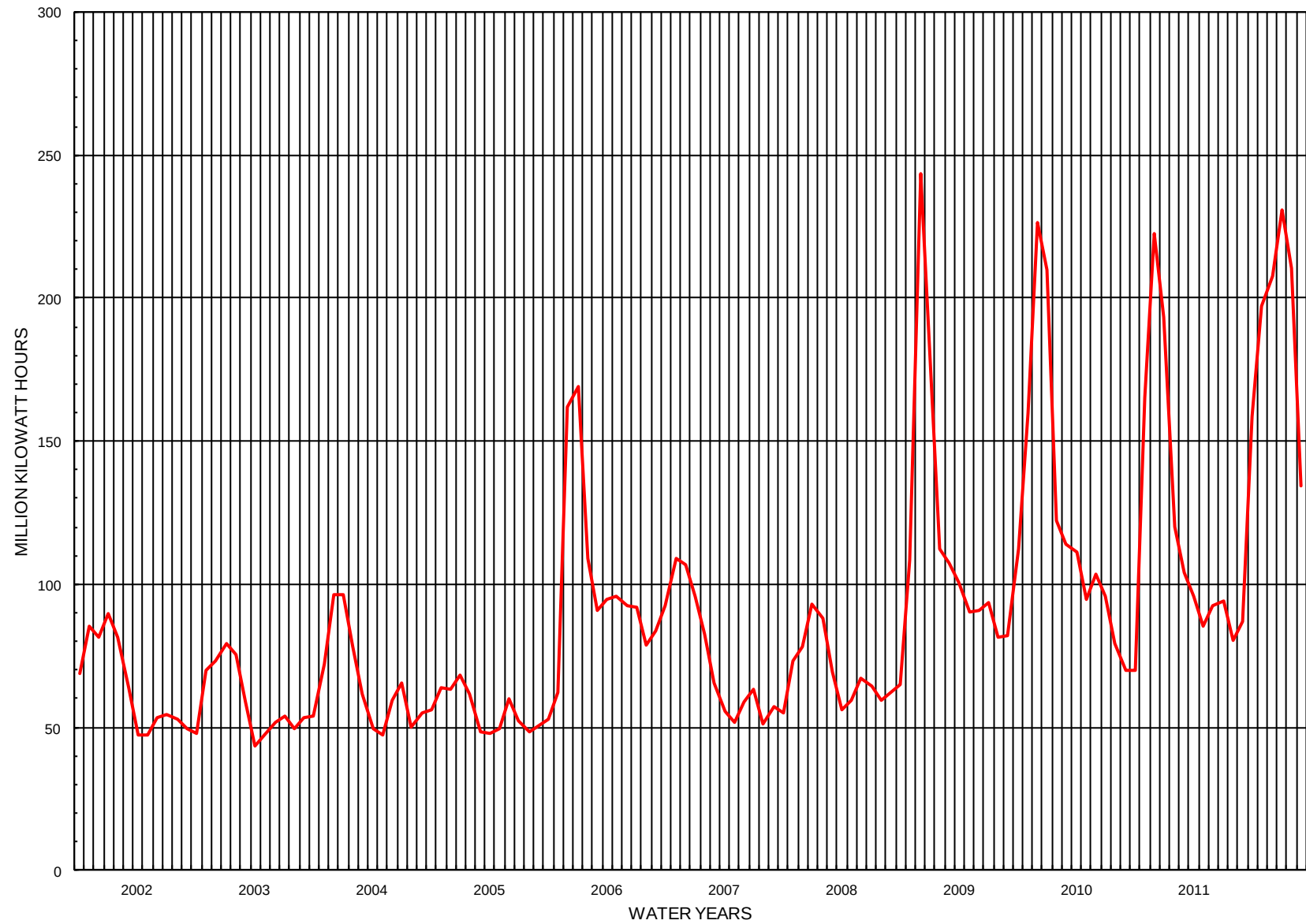
FIGURE CEG2 MONTHLY GENERATION AT USBR PLANTS
