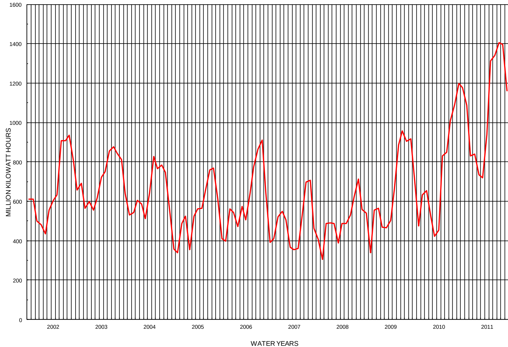
FIGURE CEG6 MONTHLY GENERATION - USBR & COE PLANTS
