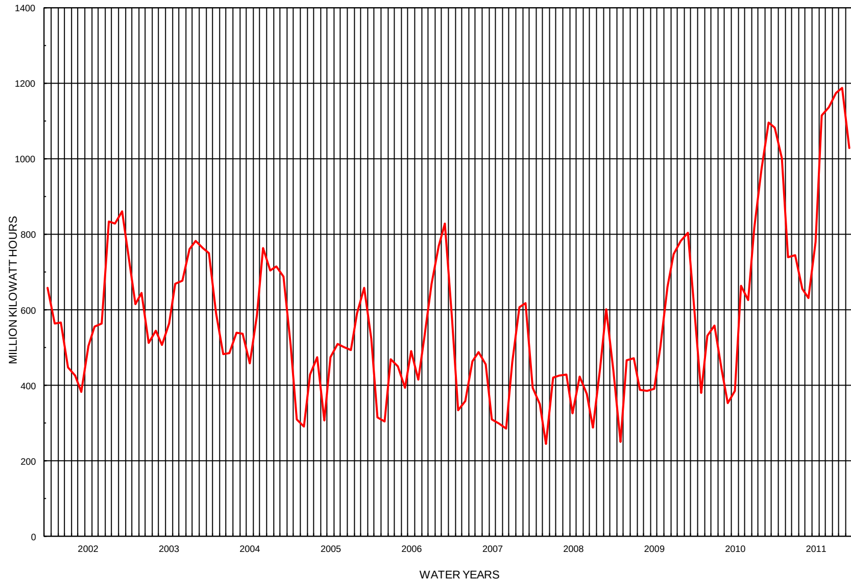
FIGURE CEG4 MONTHLY GENERATION AT COE PLANTS
