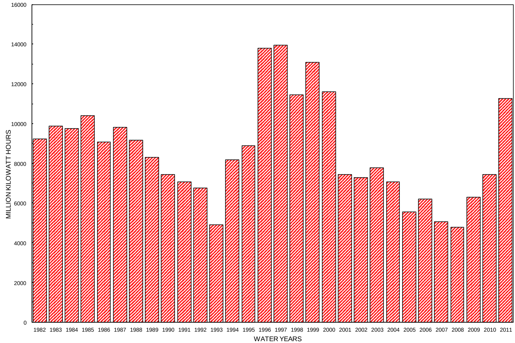
FIGURE CEG3 ANNUAL GENERATION AT COE PLANTS
