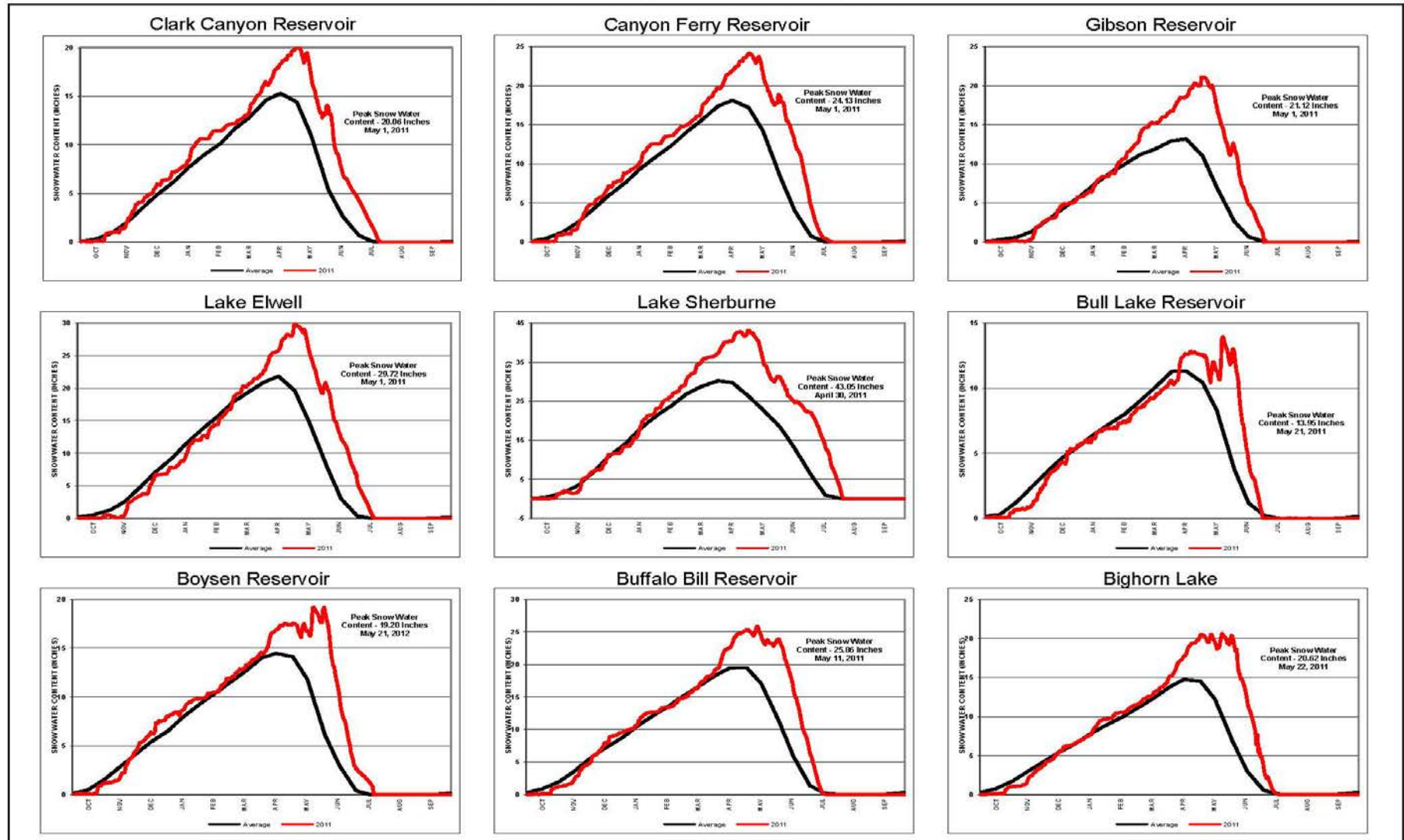
Figure MTG1 WATER YEAR 2011 SNOW WATER CONTENT
