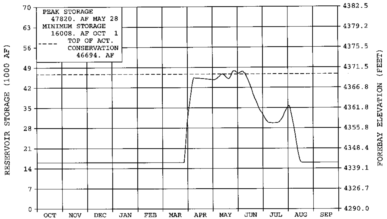
FIGURE MTG6 PISHKUN RESERVOIR NEAR AUGUSTA
