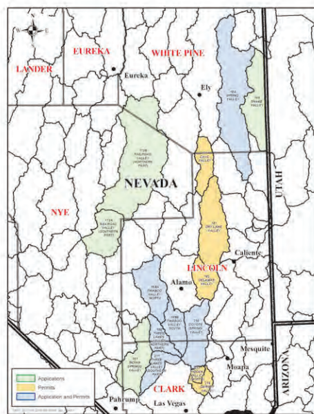
FIGURE 21 –Groundwater Basins with Active Applications/Permits
