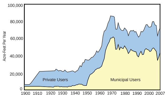
FIGURE 18 – Groundwater Use by User Type
