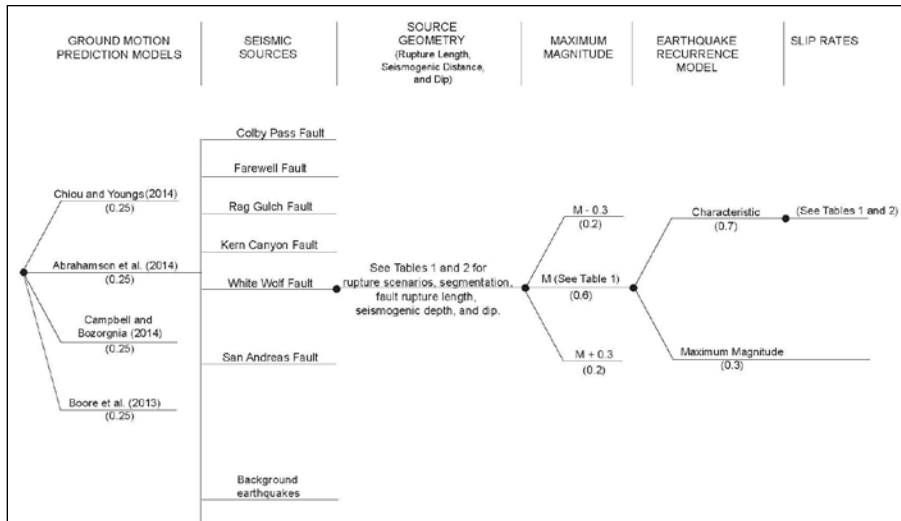
Figure B-2-2.—Example seismic source characterization logic tree, showing GPME used for each seismic source (listed on chart without a nodal circle), and subsequent fault characterization nodes. The source geometry node consists of several individual nodes similar to logic tree on figure B-2-1.
