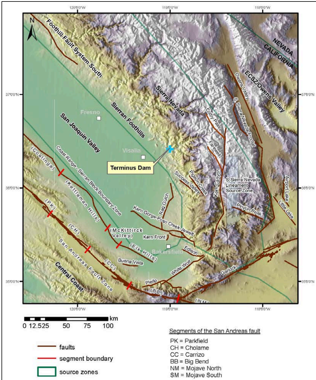
Figure B-2-3.—Map showing simplified traces (bold red lines) of faults considered potential seismic sources of significance to Terminus Dam, and areal source zones (outlined in green) used in background seismicity analysis (USGS).
