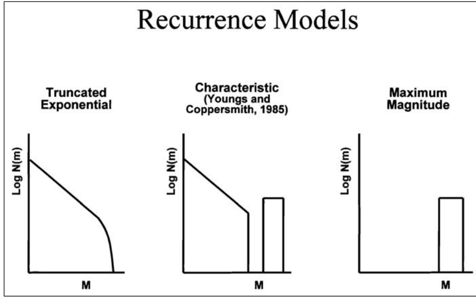
Figure B-2-5.—Three recurrence models typically used in PSHA; M (x-axis) is earthquake magnitude and Log N(m) (y-axis) is number of events per year.
