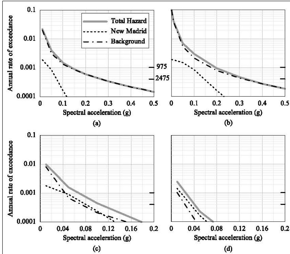
Figure B-2-12.—Mean hazard curves for average horizontal component (a) PGA, (b) spectral acceleration = 0.2 s, (c) spectral acceleration = 1.0 s, and (d) spectral acceleration = 3.0 s; before applying site amplification factors. Two return periods of 975 and 2,475 years are marked on the right y-axis (from Hashash et al. 2015).
