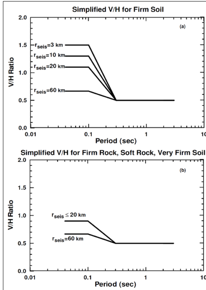
Figure B-2-11.—Plots showing differences in V/H ratios with site class and distance from the seismic source.
