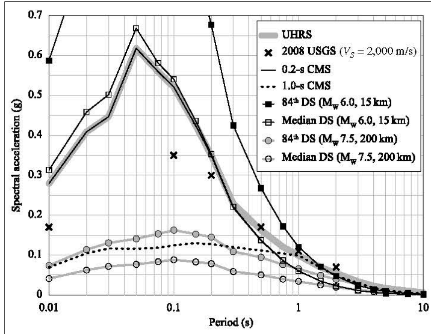
Figure B-2-13.—Horizontal UHRS (with 5% damping) and CMS for T = 0.2 s and T = 1.0 s for a 2,475-year return period, compared with median and 84th percentile for M_w 6.0 and M_w 7.5 deterministic spectra (DS). Also shown is the 2008 USGS-derived UHRS data for a 2,475-year return period and “rock” site conditions ( V_S = 2,000 meters per second). Note similarity between the 1.0-sec CMS (dotted line) and the spectra derived from the large ( M_w 7.5 ) NMSZ earthquake; and the similarity between the 0.2-sec CMS and the spectra derived from the smaller ( M_w 6.0 ) background-source earthquake.
