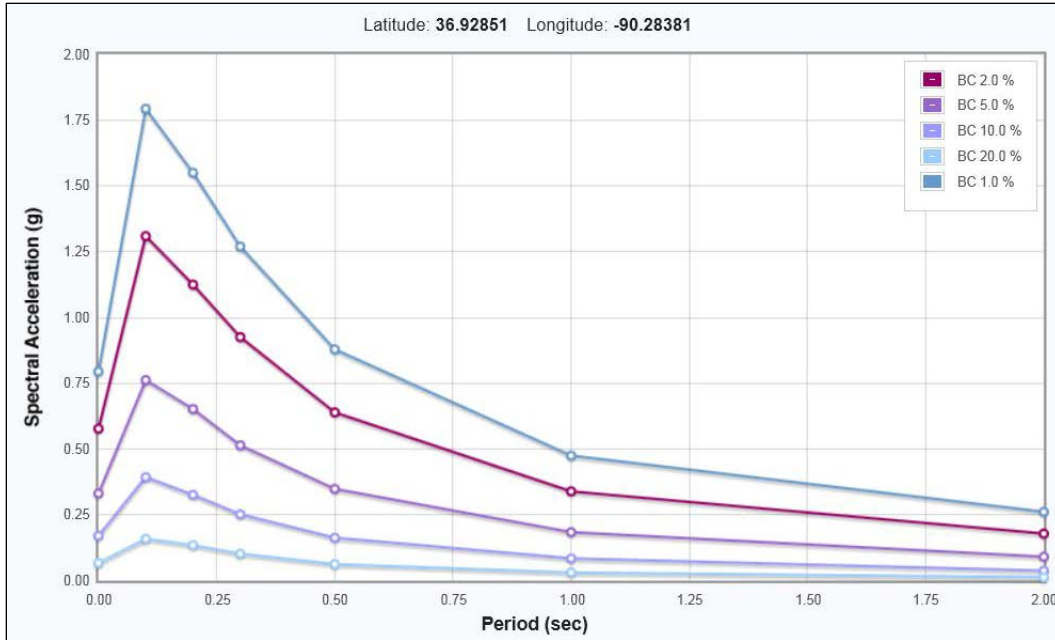
Figure B-2-10.—Mean UHRS from all sources for Wappapello Dam, Missouri, for return periods of 225 years (20% in 50 years), 475 years (10% in 50 years), 975 years (5% in 50 years), 2,475 years (2% in 50 years), and 5,000 years (1% in 50 years) (from USGS Unified Hazard Tool).
