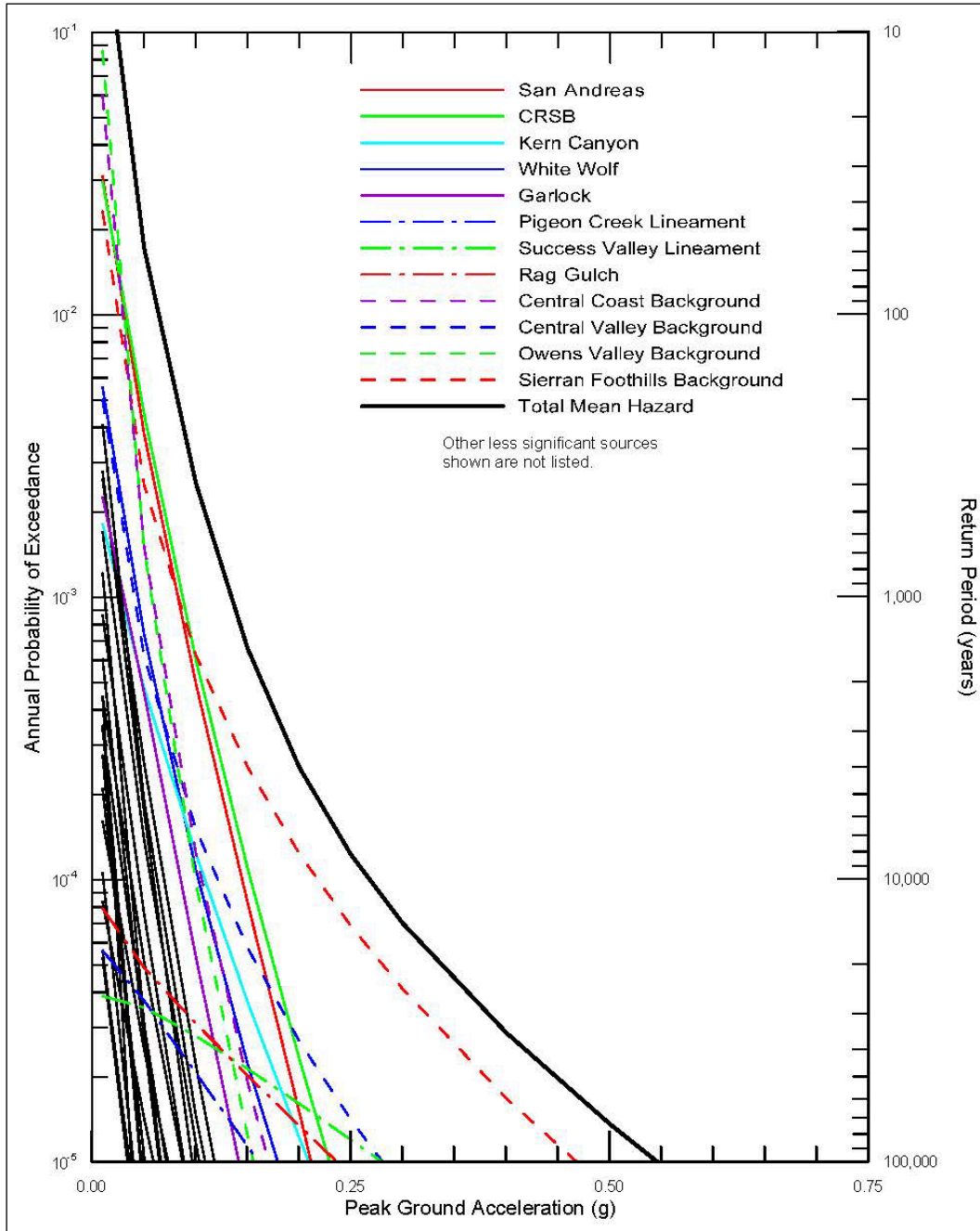
Figure B-2-7.—Seismic hazard curves for Success Dam in south-central California, showing contributions to PGA cumulative hazard from various local and regional fault sources and areal source zone.
