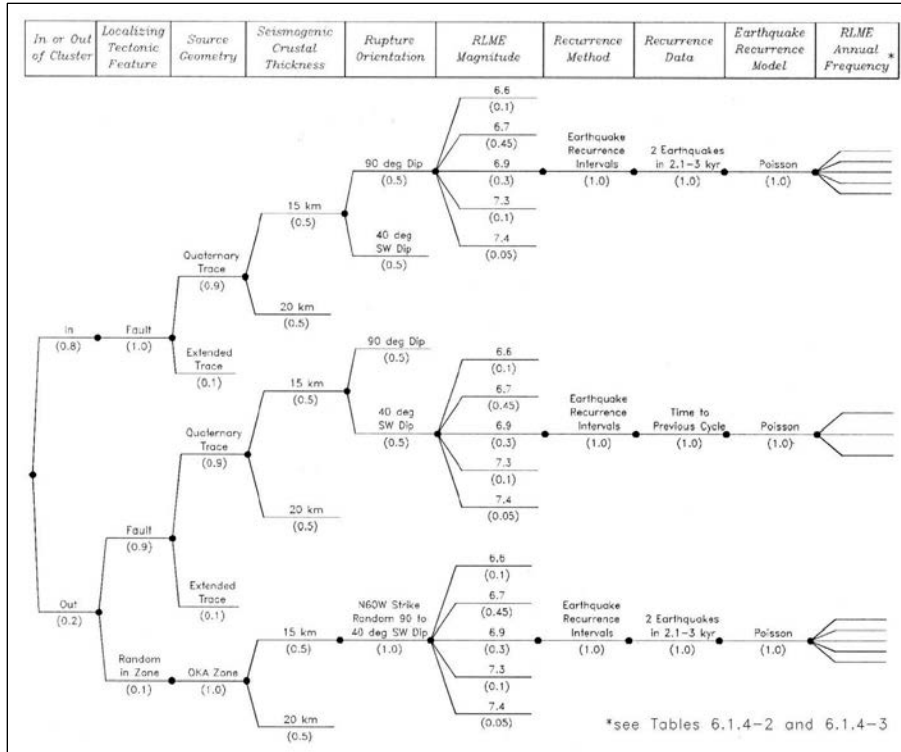
Figure B-2-1.—Example fault source logic tree for a single fault, showing fault parameters in boxes above each node, cases considered for each node in the tree, and assigned weights (in parentheses) for each case. Nodes are repeated for entire logic tree, but shown only once on figure (example is Meers fault, Oklahoma [CEUS-SSC 2012]).
