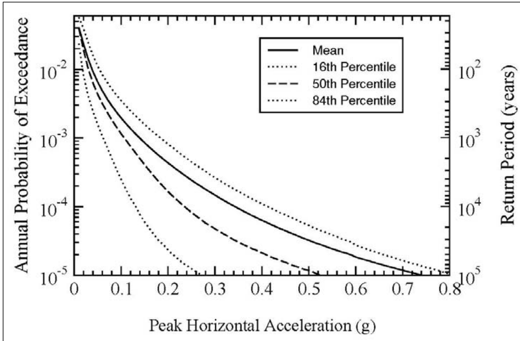
Figure B-2-6.—Example of mean and percentile hazard curves for PHA.
