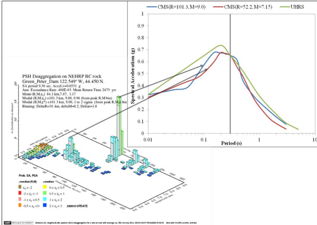
Figure B-2-14.—Example CMS for Green Peter Dam (Oregon) generated using the 2008 USGS de-aggregation tool for probability of exceedance of 2% in 50 yr.
