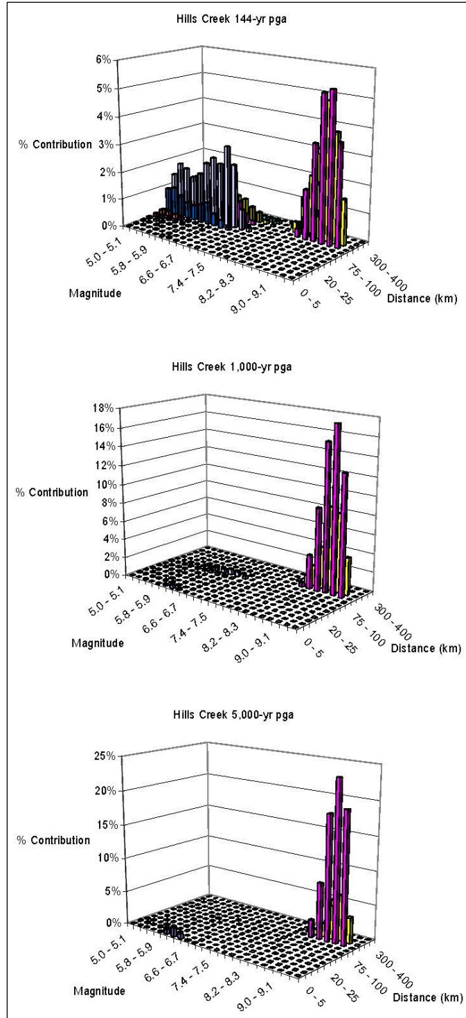
Figure B-2-9.—Seismic hazard de-aggregation plots showing contributions to mean PGA hazard for each magnitude-distance pair for Hills Creek Dam in central Oregon, for return periods of: a) 144 years, b) 1,000 years, and c) 5,000 years.
