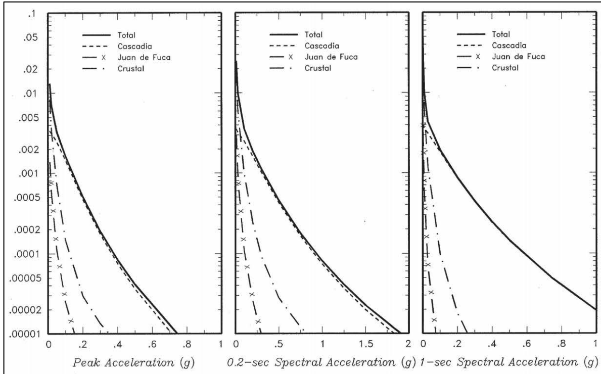
Figure B-2-8.—Seismic hazard curves for Hills Creek Dam in central Oregon, showing Annual Exceedance Probabilities (AEP) for PGA and two spectral frequencies. The plots show the contributions to various spectral acceleration cumulative hazard from the Cascadia Subduction Zone (CSZ) source, the Juan de Fuca intra-slab source, and shallow crustal fault sources. Note that the CSZ dominates hazard for all three spectral accelerations, but that relative contributions from other sources vary for different spectral accelerations.
