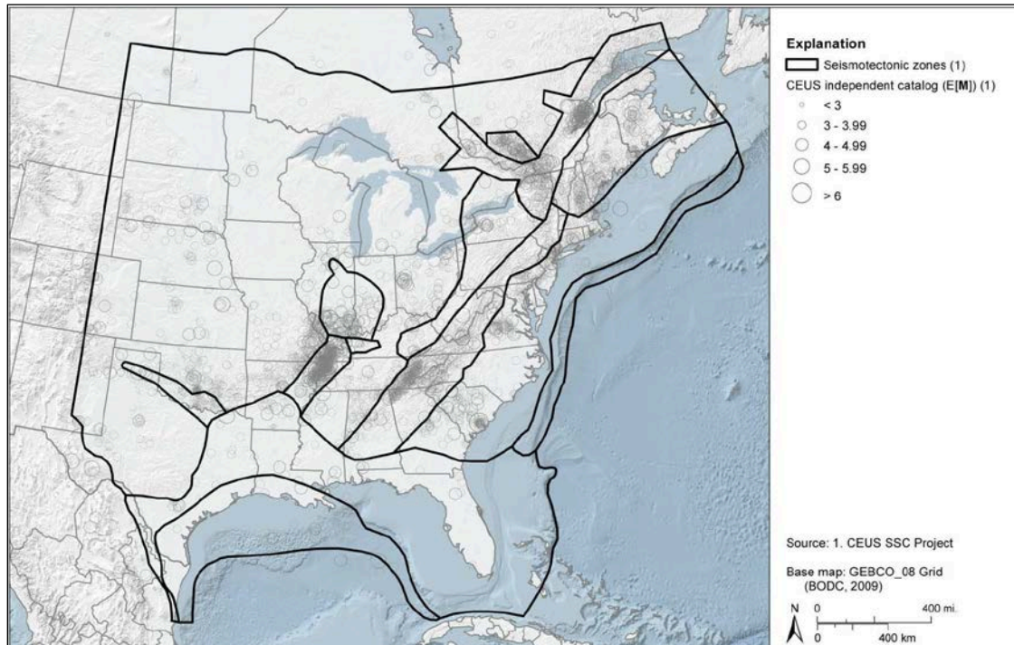
Figure B-2-4.—Example map of seismotectonic zones in the CEUS (black polygons) and earthquakes in the historical seismicity catalog (grey circles) (CEUS-SSC 2012).
