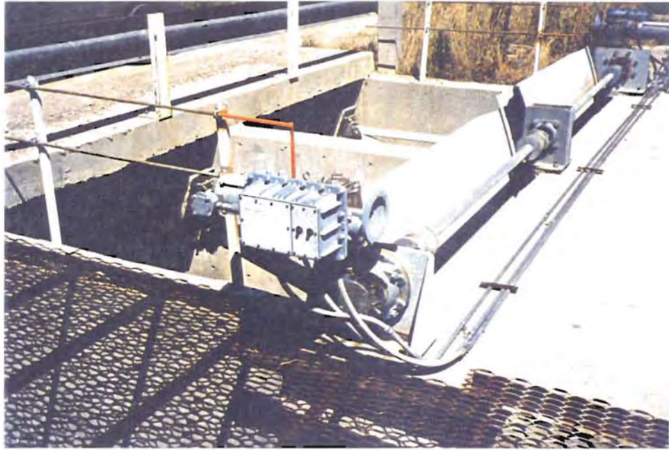
Photo 7 - Radial gates at GMC-57 Check (Mary Taylor Drop)
