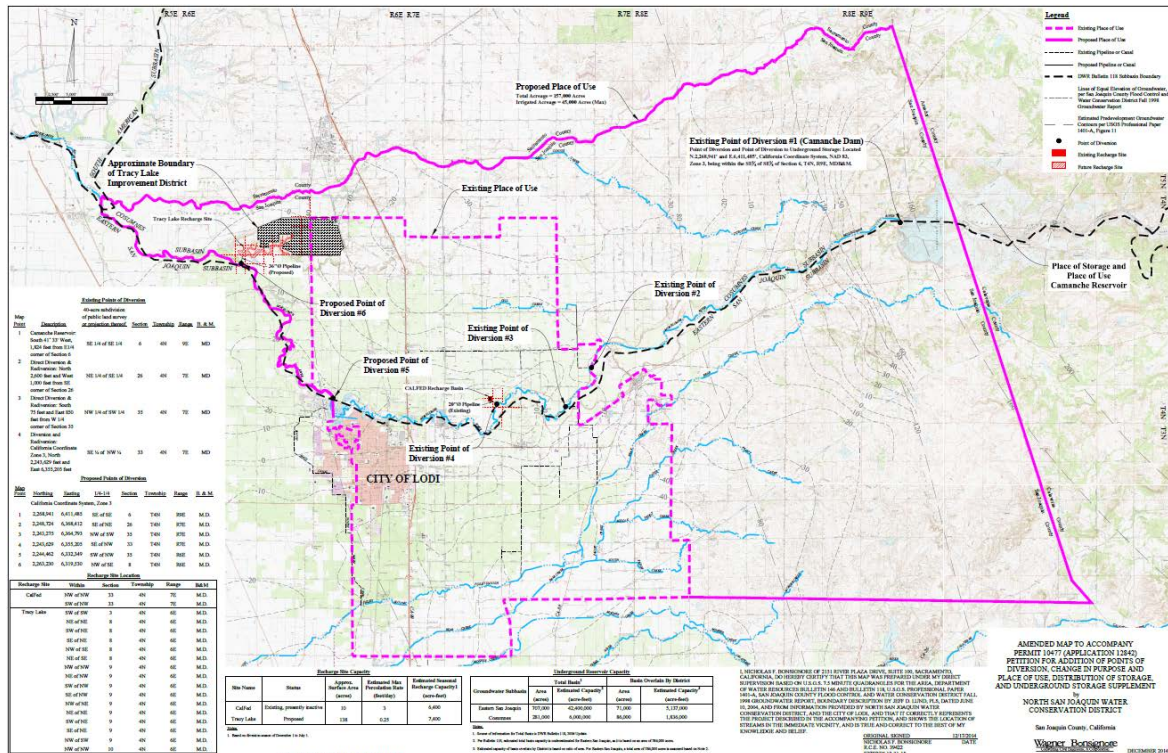
Figure 1. NSJWCD District Boundaries and Points of Diversion.
