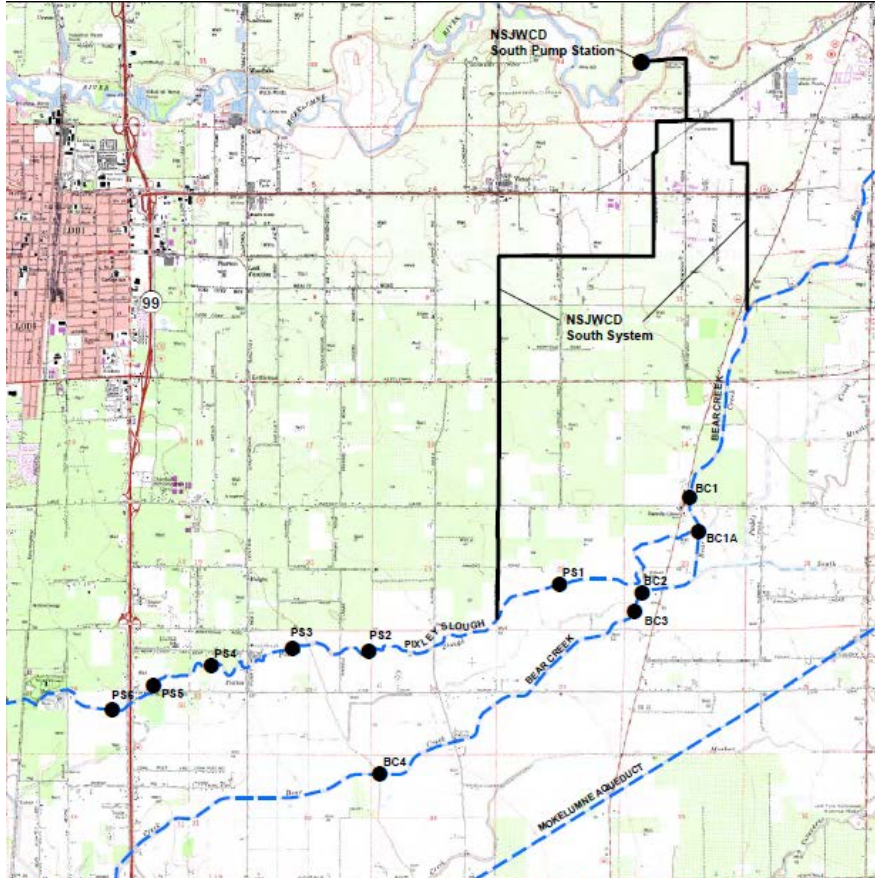
Figure 2. Diagram of South System Facilities.
