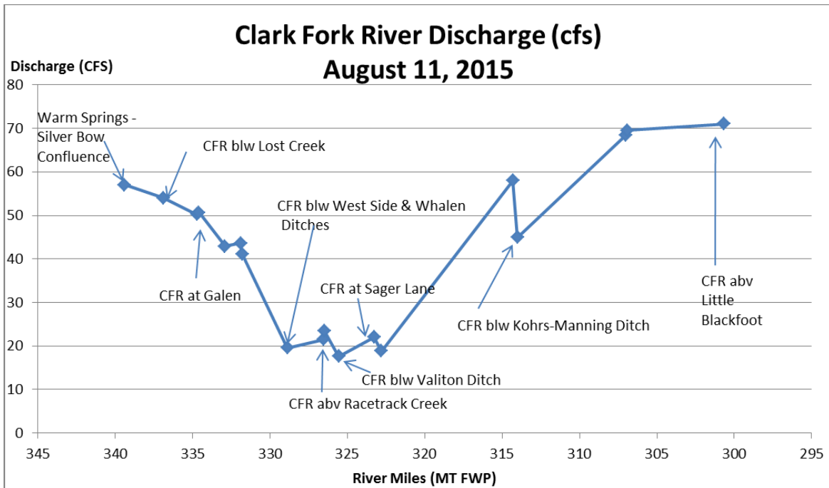
Figure 9- Graph showing CFC’s synoptic stream flow measurements from August, 2015 on the reach of the Upper Clark Fork River from the confluence of Silver Bow and Warm Springs Creeks downstream (north) to just above the mouth of the Little Blackfoot River near Garrison. Downstream of Sager Lane the river goes through a gaining reach, and recovers rapidly as return flows become the dominant hydrologic process. Much of these return flows are attributable to leaky ditches and inefficient irrigation techniques. Flows are still impaired at Deer Lodge at times but to a much smaller degree than upstream locations. Gage data from Deer Lodge show a mean annual flow rate of 287 cfs, or ~200,000 acre feet per year (USGS, 2016b). August shows the lowest mean monthly flow at 109 cfs (July and August flows often dip below aquatic habitat-derived flow targets – see Fig. 10) but the river experiences a marked recovery of flows from late September to mid-November. This is likely due to a combination of reduced irrigation demand, irrigation return flows, fall precipitation, and overall reduced basin evapotranspiration as air temperatures drop. Mean monthly flows between November and March remain fairly stable, at 200 - 250 cfs (Figure 11).
