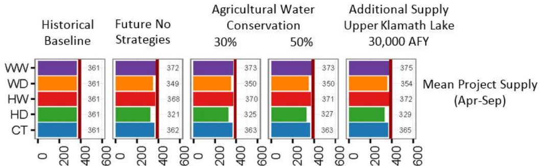
Figure 12.—Summary of historical and future system reliability for the 2070s with adaptation strategy concepts for average seasonal Klamath Project supply.
